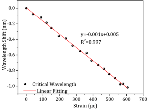
Fig. 8. Wavelength shift of CWL over the strain range from 0 to 600με.
