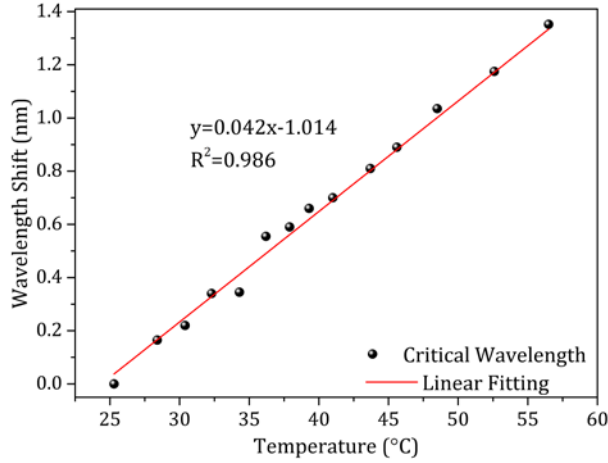
Fig. 9. Wavelength shift of CWL over the temperature range from 25.3 to 58°C.
