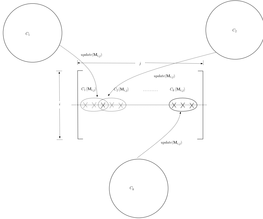
Figure A.2: Showing example global matrix allocated across controllers allowing overlaps, i.e. \bigcap_{n \in \mathbb{N}} C_n(\mathbf{M}_{i,j}) \neq \emptyset using a tuple space
