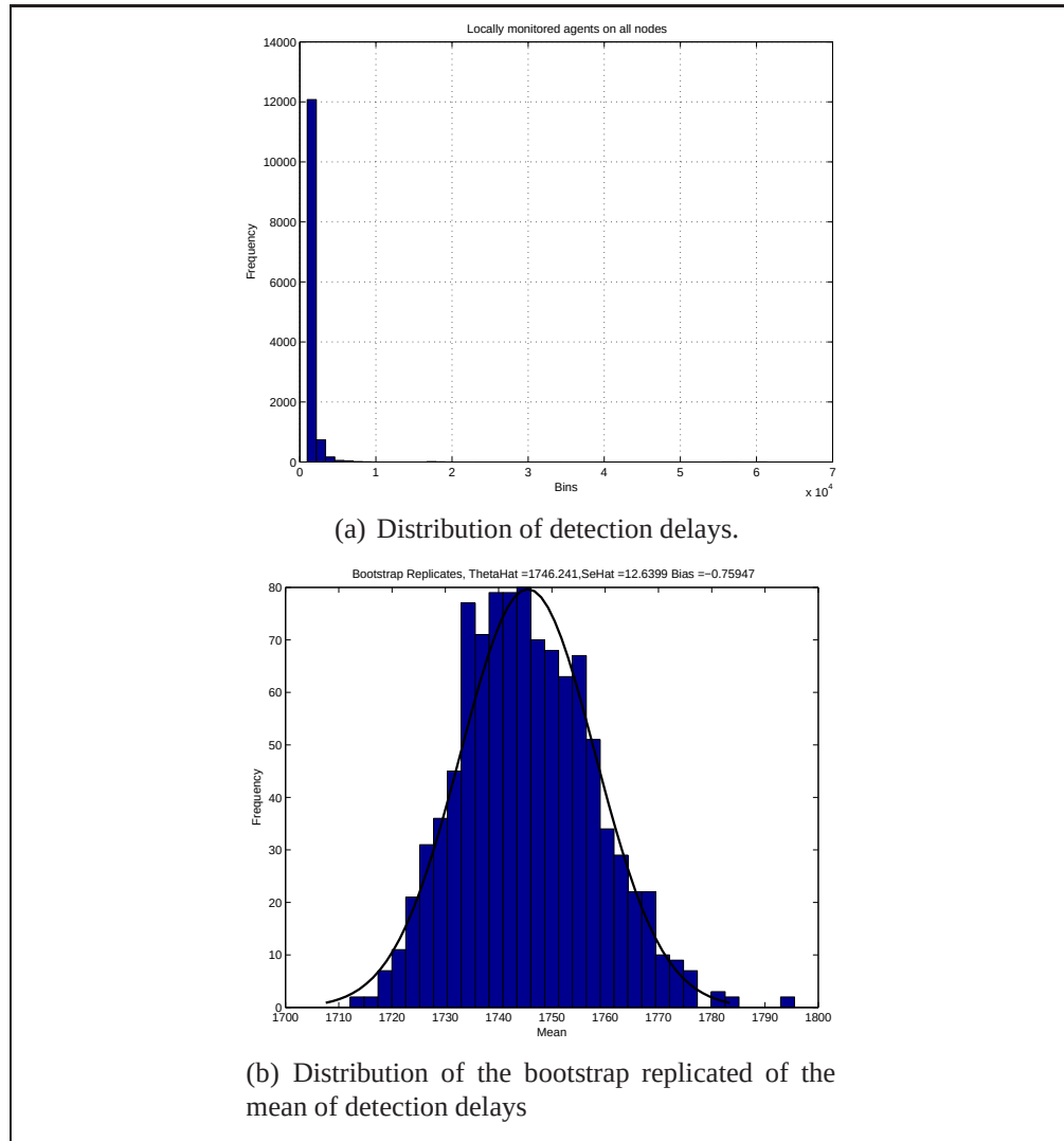
Figure 10.7: (a) This figure shows the distribution of the detection delays. As it is outliers were not filtered out hence the skewed distribution. (b) Showing the distribution of bootstrap replicates for the mean for scenario 1 (all data for locally monitored agents), showing a peak at \approx 1750ms for this dataset.
