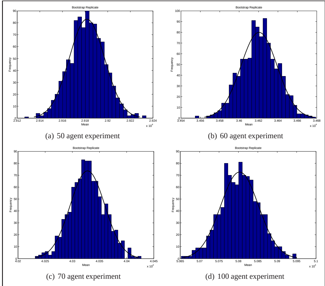
Figure 8.7: Figures (a)-(d) show bootstrap replicates of the mean for centralised experiments using the full protocol scheme where agent numbers were varied from 50 through to 100
