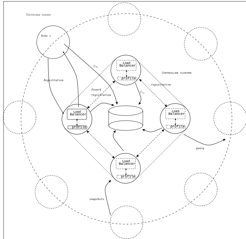
Figure 6.4: Distribution architecture, showing nodes hosting agents in a local area network and a cluster controllers in distributed agent platforms.
