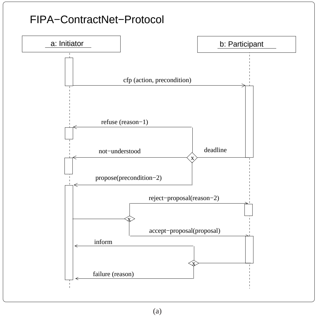
Figure 4.4: FIPA contract-net protocol adapted from [1].
