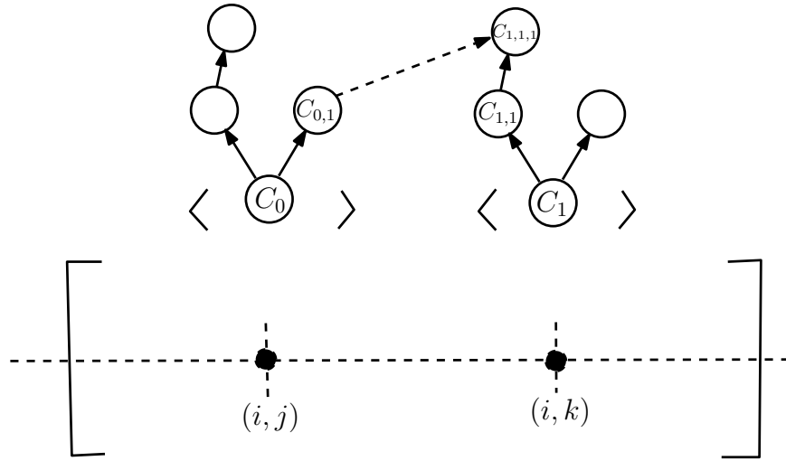
Figure A.4: Showing an extended model for conversations, with dependencies between computation trees
