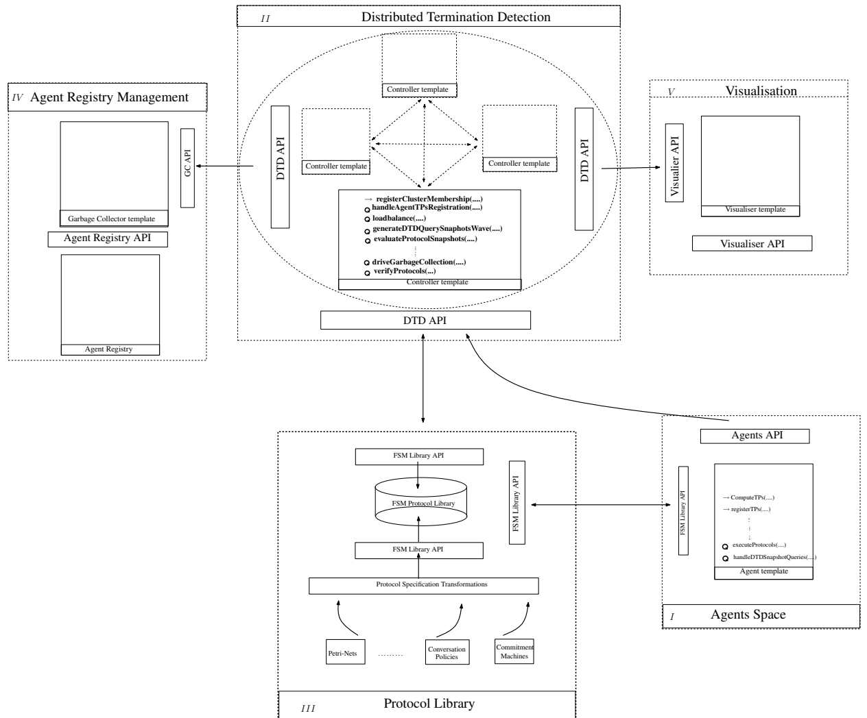
Figure 5.14: A proposed termination detection architecture for a multiagent system.
