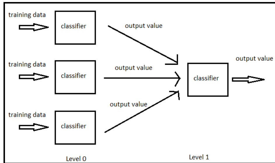
Figure 4.5: Stacking Process
