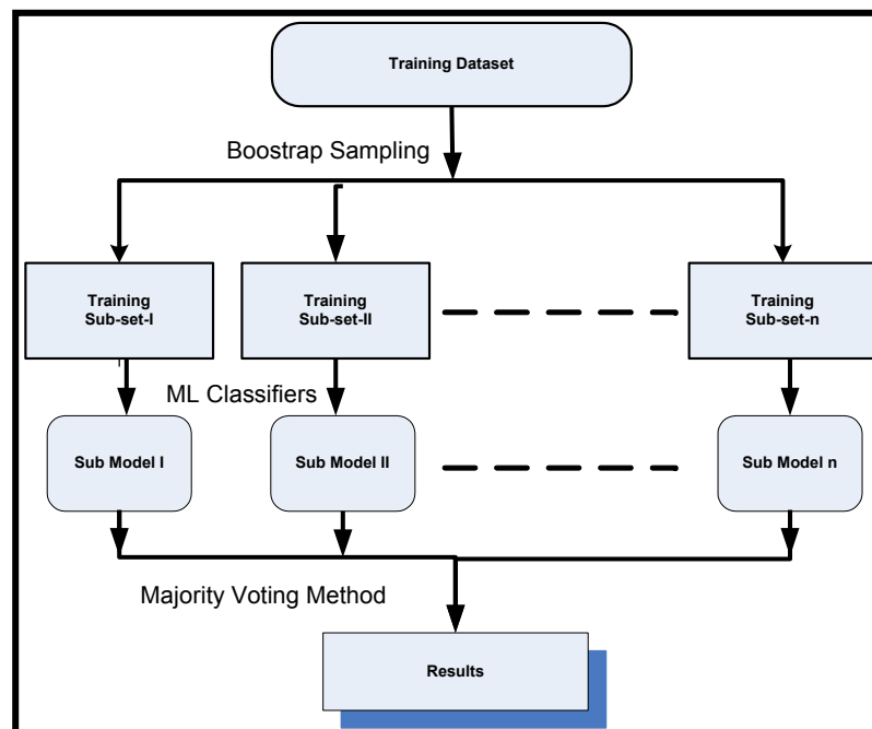
Figure 4.4: Bagging Process
