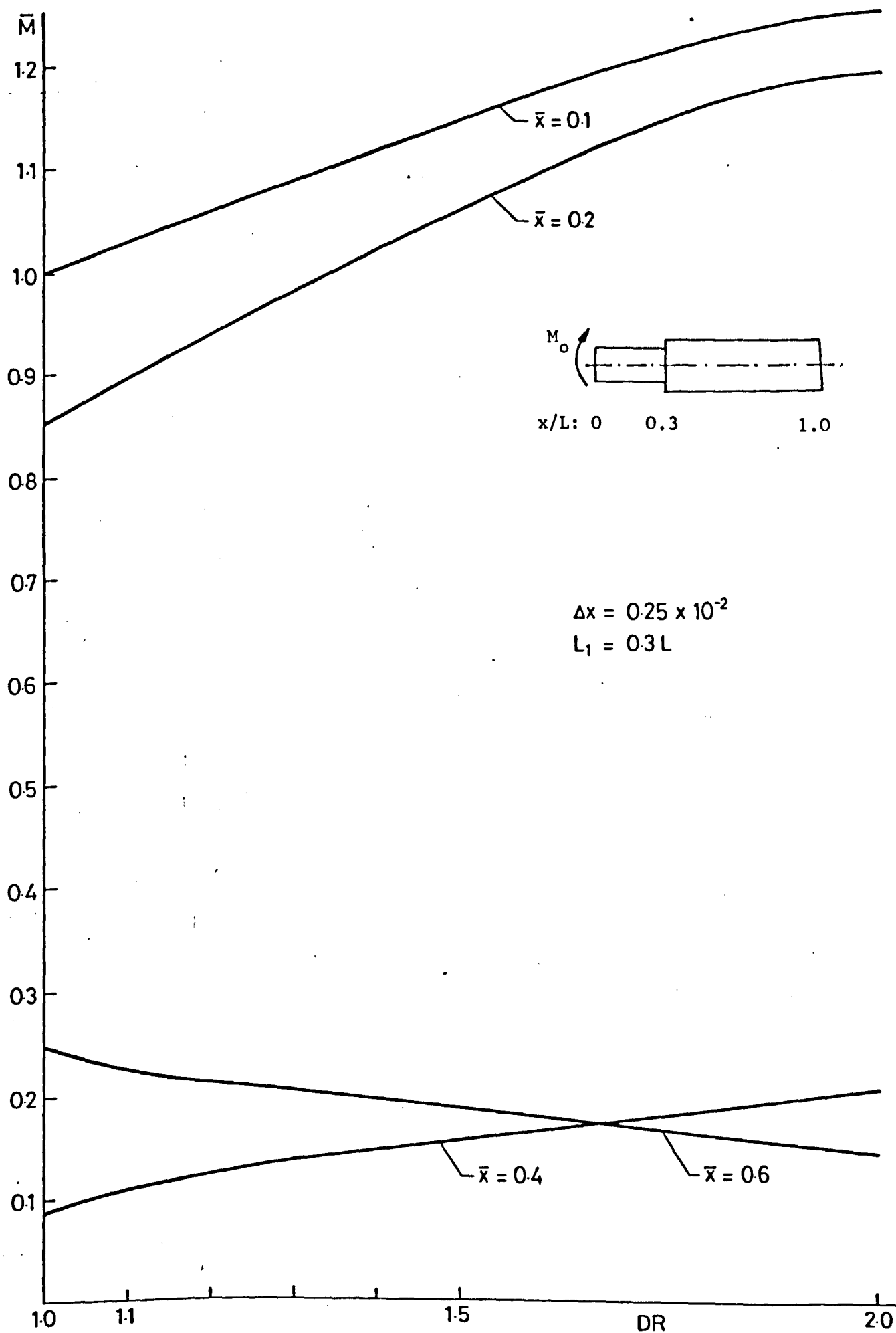
FIG.5.20 PEAK VALUES OF \bar{M} , vs. DIAMETER RATIO
