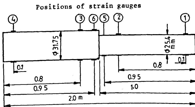
a. Short stepped beam ( Test beam II )
