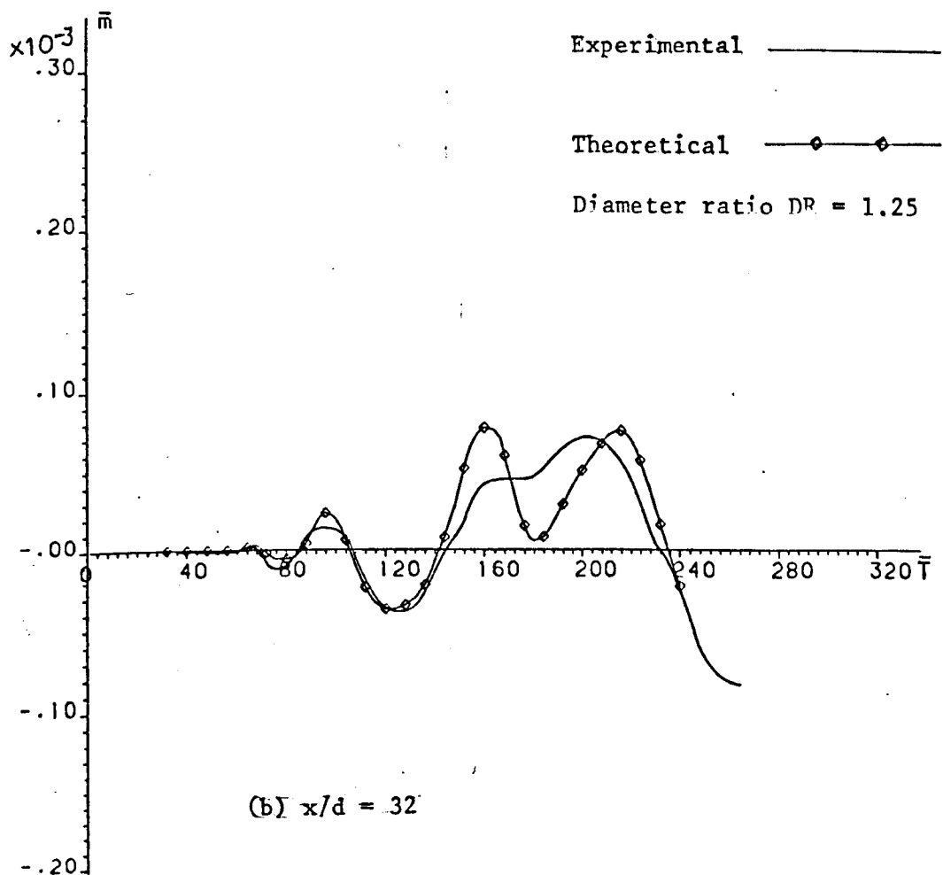
FIG. 8.6 COMPARISON OF EXPERIMENTAL AND THEORETICAL NON-DIMENSIONAL BENDING MOMENT HISTORY FOR THE 3.295 m 3 LONG STEPPED BEAM
