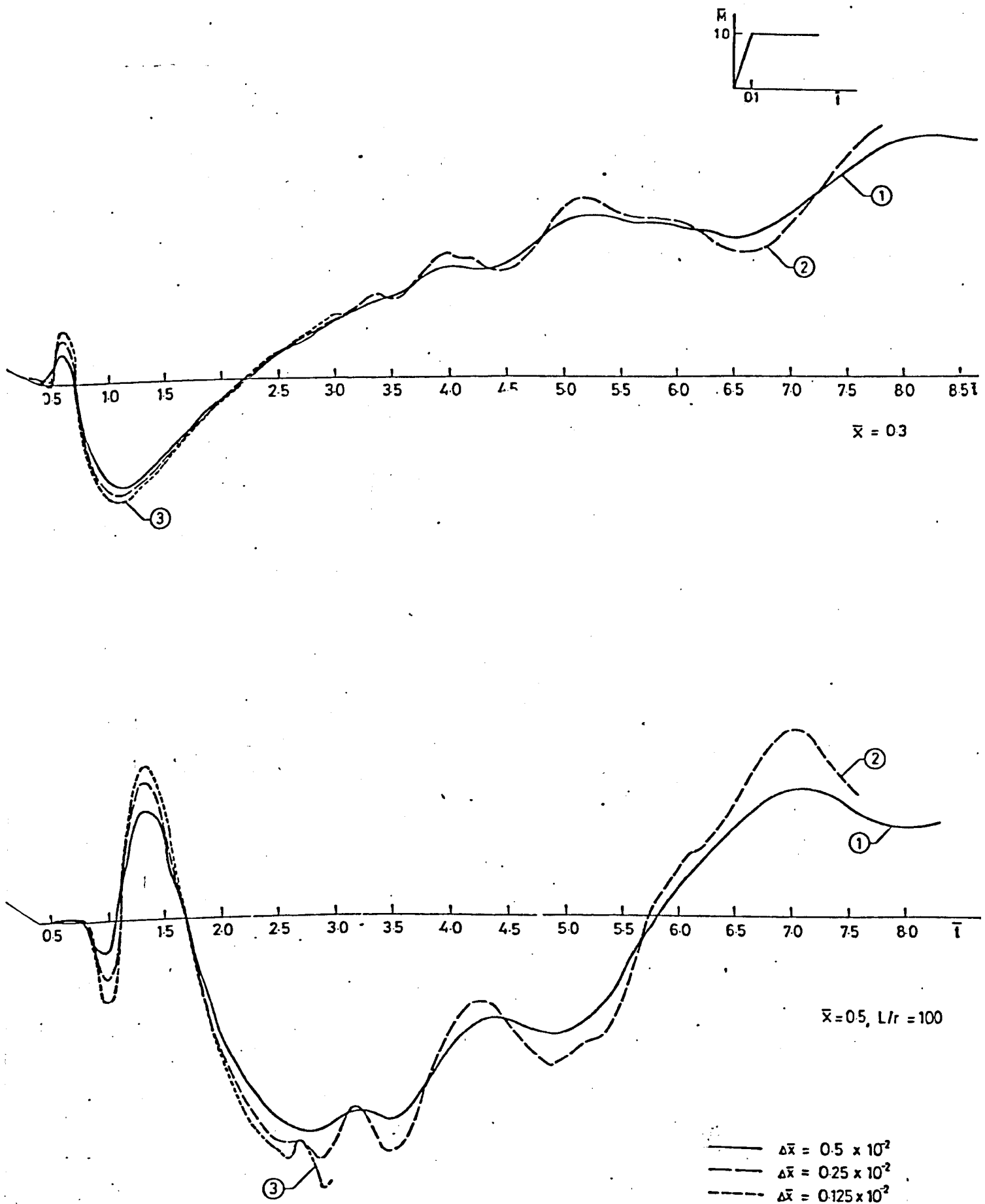
FIG. 512. EFFECT OF MESH SIZE \Delta \bar{x} Simply supported beam
