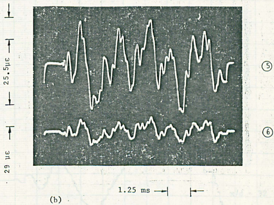
FIG. 7.21 BENDING STRAIN-TIME PROFILES AT VARIOUS POSITIONS ALONG THE 2.0 m LONG STEPPED BEAM DUE TO ECCENTRIC IMPACT
