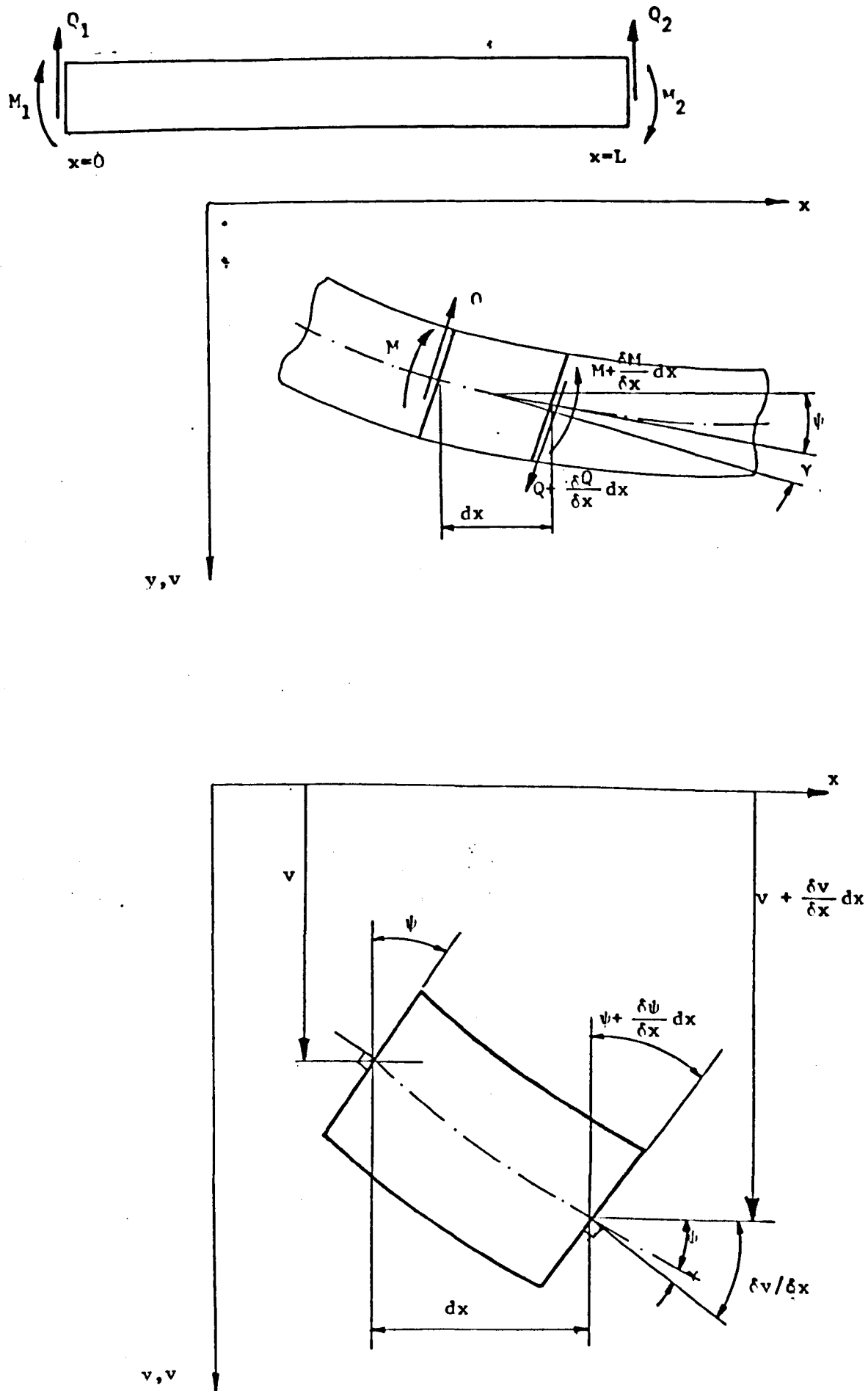
FIG. 3.1 TIMOSHENKO BEAM AND TIMOSHENKO ELEMENT
