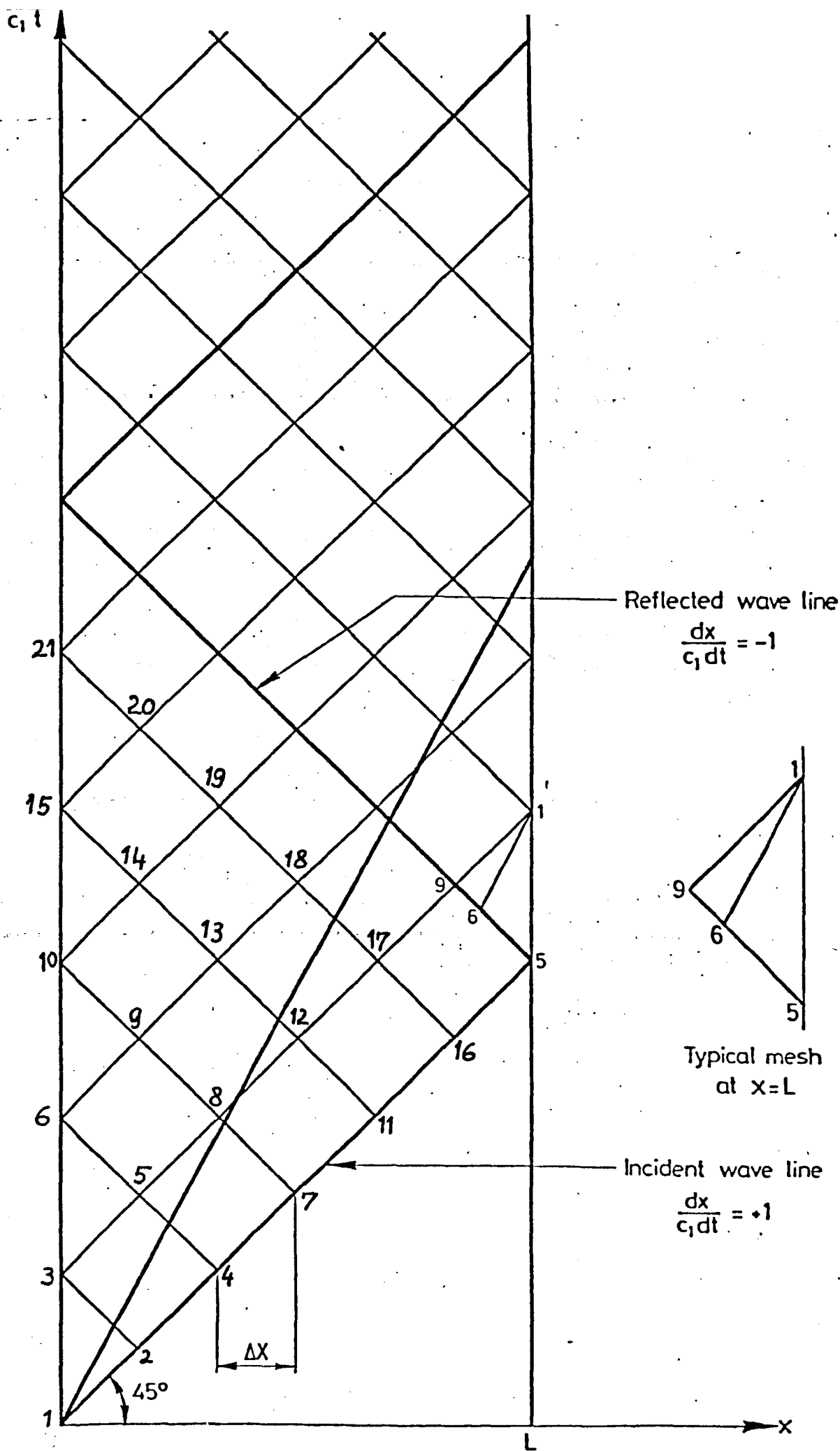
FIG. 4.7 FINITE BEAM CHARACTERISTIC NETWORK
