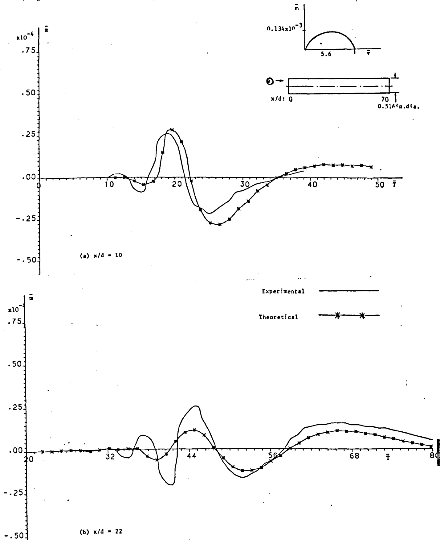
FIG. 5.5 MEASURED AND CALCULATED HISTORIES OF THE BENDING MOMENT FOR A 36.12 in. LONG FREE-FREE CYLINDRICAL BEAM SUBJECTED TO ECCENTRIC IMPACT
