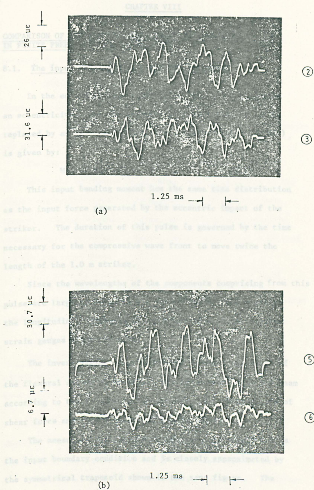
FIG. 7.31 BENDING STRAIN-TIME RESULTS FOR VARIOUS POSITIONS OF THE STEPPED BEAM OF RECTANGULAR CROSS SECTION DUE TO ECCENTRIC IMPACT WITH THE 1.0 m LONG CYLINDRICAL STRIKER
