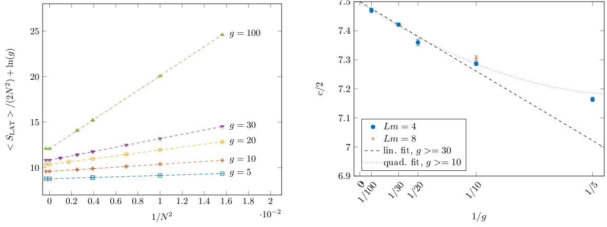
Figure 11: Plots of \frac{\langle S_{\text{LAT}} \rangle}{2N^2} and its continuum extrapolation to determine c/2 , realized here using the SO(6) -breaking discretization (B.1)-(B.2). Detailed explanation and comments as in Fig. 4.
