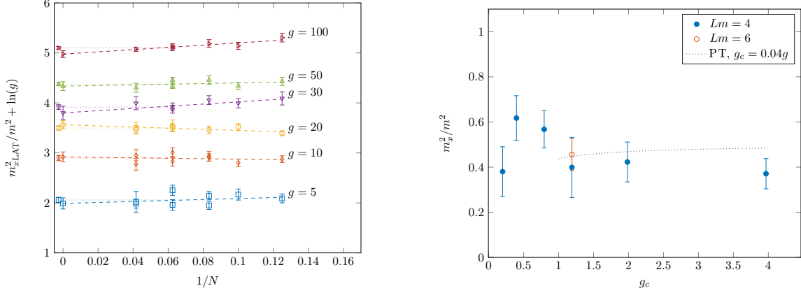
Figure 3: Left panel: Plot of m_{x\text{LAT}}^2(N, g)/m^2 = m_x(g) + \mathcal{O}(1/N) , as from plateaux average of results which for g = 30 are shown in Fig. 2 (right panel). To ensure better visibility of the fits at different g values, \ln g has been added. Dashed lines represent a linear fit to all the data points for one value of g , while for dotted lines the fit is to a constant and only includes the two smallest lattice spacings. Multiple points at the same value of g and N indicate multiple replica. Right panel: Continuum extrapolation corresponding to the linear fits in the left panel. The simulations represented by the orange point ( mL = 6 ) are used for a check of the finite volume effects, that appear to be within statistical errors. The extrapolation is plotted as a function of the continuum coupling g_c = 0.04g to facilitate the comparison with the prediction coming from the perturbative expectation (PT) (2.4), and uses the matching procedure performed for the observable action. The latter is described in Section 4.2 and commented further in Section 5.
