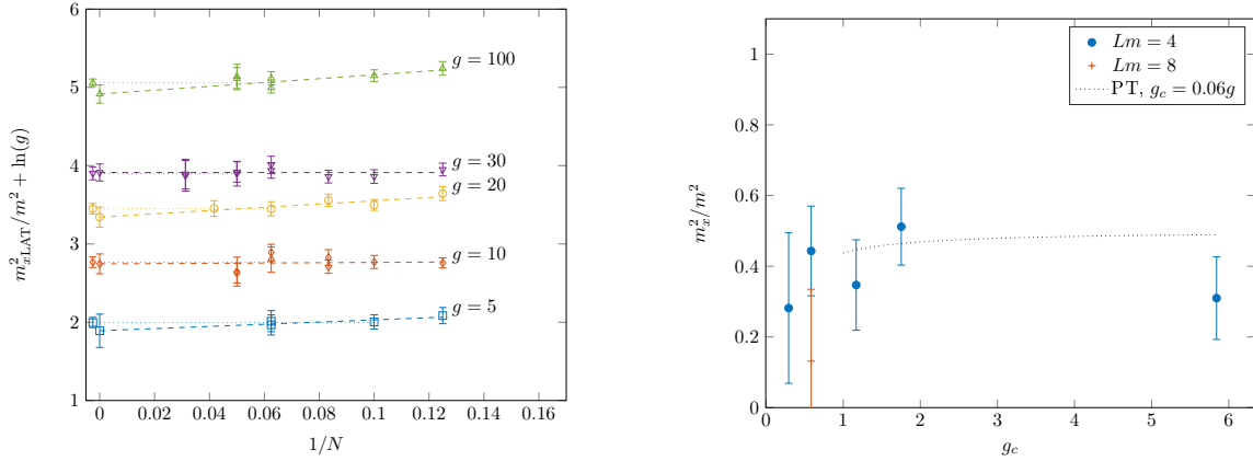
Figure 10: Plot of m_{xLAT}^2(N, g)/m^2 = m_x(g) + \mathcal{O}(1/N) and its continuum extrapolation, realized here using the SO(6) -breaking discretization (B.1)-(B.2). Detailed explanation and comments as in Fig. 3.
