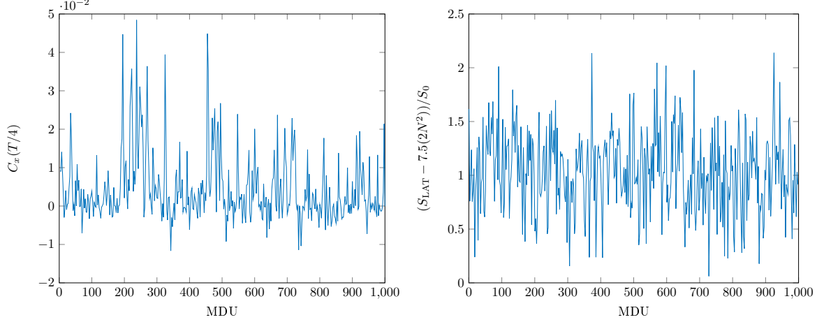
Figure 1: Monte Carlo histories for the correlator \langle x x^* \rangle at time separation T/4 and for \langle S_{\text{cusp}} \rangle , at g = 10 and L/a = 16 , in terms of Molecular Dynamic Units (MDU). The HMC produces a series of bosonic field configurations, on each of them the observable is evaluated and plotted here for the same series at the given parameters. The fact that successive configurations produced by the RHMC are statically correlated might lead to strong so-called auto-correlations in the data, which would appear in these plots as fluctuations with long periods. As one can see, the histories presented here do not suffer from such long fluctuations, and sample well the observables under investigation.
