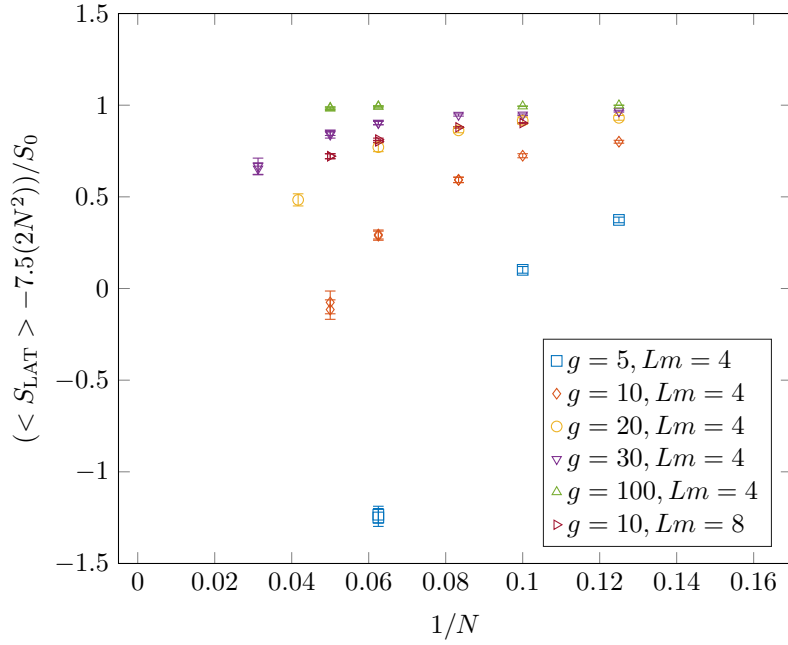
Figure 12: Plot of the ratio \frac{\langle S_{\text{LAT}} \rangle - \frac{c}{2}(2N^2)}{S_0} \equiv \frac{f'(g)}{4} , realized here using the SO(6) -breaking discretization (B.1)-(B.2). Detailed explanation and comments as in Fig. 5.
