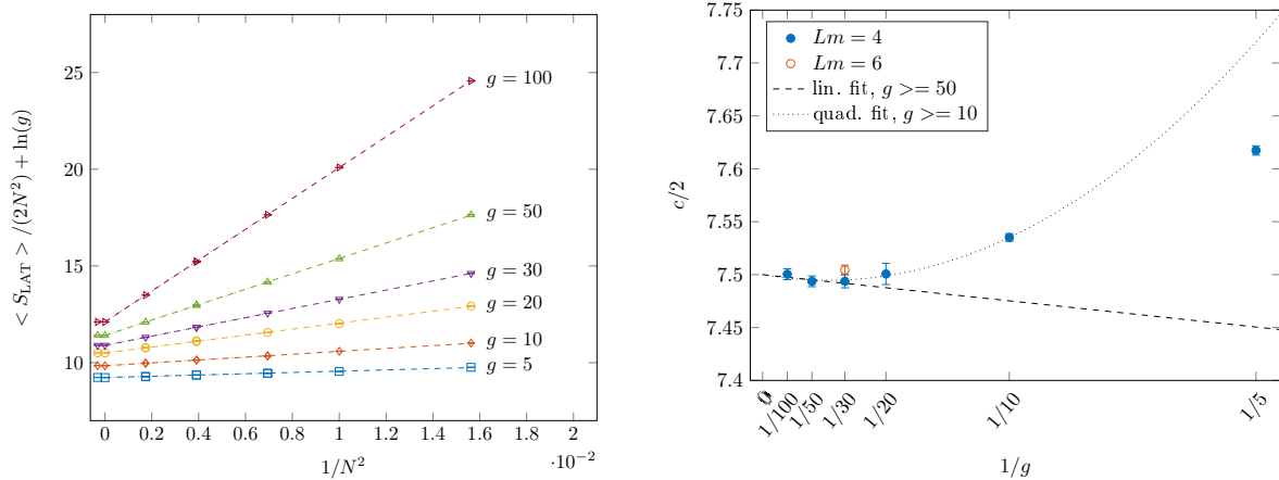
Figure 4: Left panel: Plots of \frac{\langle S_{\text{LAT}} \rangle}{2N^2} , where fits (dashed lines) to data points are linear in 1/N^2 . To ensure better visibility of the fits at different g values, \ln g has been added. The extrapolation to the continuum limit (symbol at infinite N ) determines the coefficient c/2 of the divergent ( \sim N^2 ) contribution in (4.9)-(4.10) and is represented in the diagram of the right of this figure. Right panel: Data points estimate the continuum value of c/2 as from the extrapolations of the linear fits above. The simulations at g = 30 , mL = 6 (orange point) are used for a check of the finite volume effects, which appear here to be visible. Dashed and dotted lines are the results of, respectively, a linear fit in 1/g and a fit to a polynomial of degree two.
