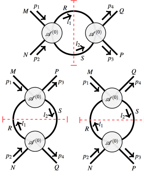
Figure 2: Diagrams representing s-, t- and u-channel cuts contributing to the four-point one-loop amplitude.
