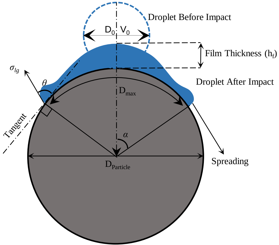
Figure 2.18: Schematic of droplet spreading on a spherical particle surface ( D_0 : droplet diameter, V_0 : droplet velocity, D_{Particle} : particle diameter, D_{max} : maximum spreading diameter, \alpha : half-spread angle, \theta : apparent dynamic contact angle, h_f : thickness of film, \sigma_{lg} : liquid–gas surface tension)
