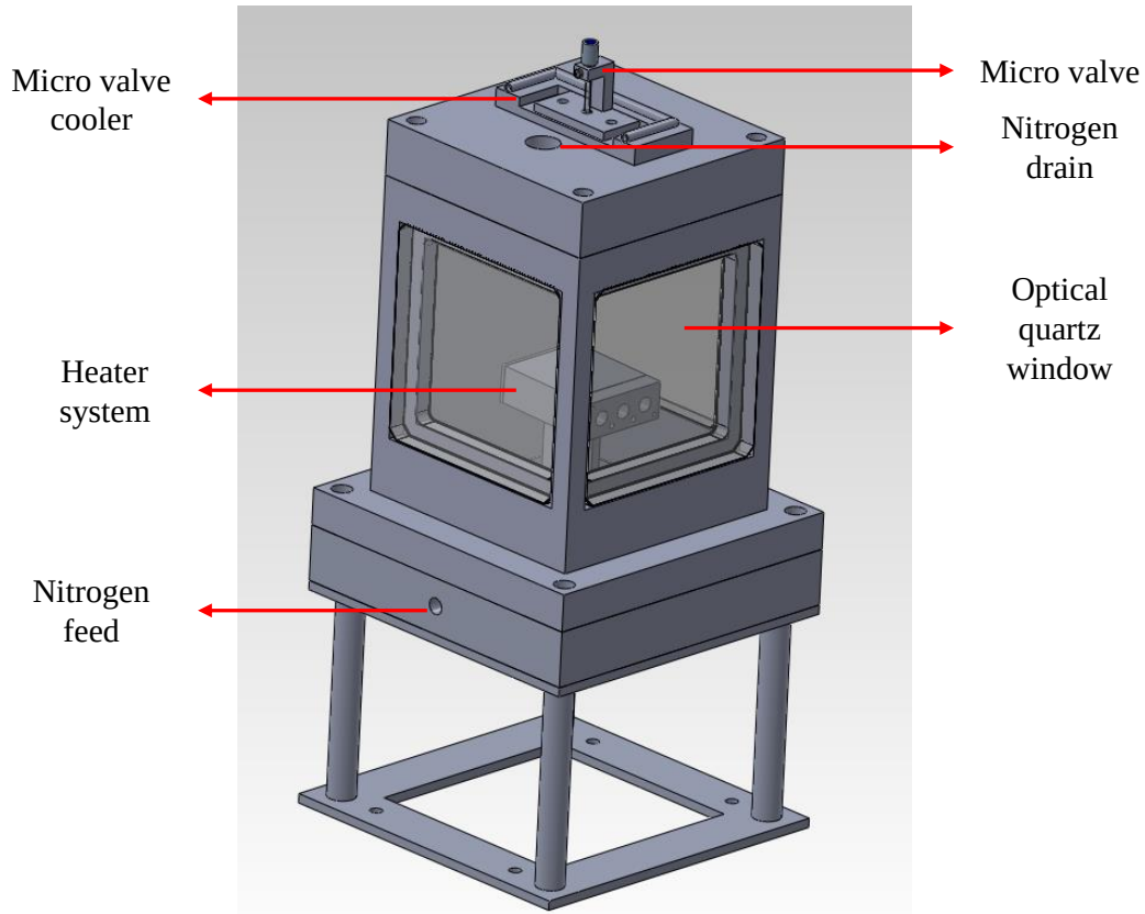
Figure 2.9 3D design of the high pressure chamber facilitated with experimental inserts
