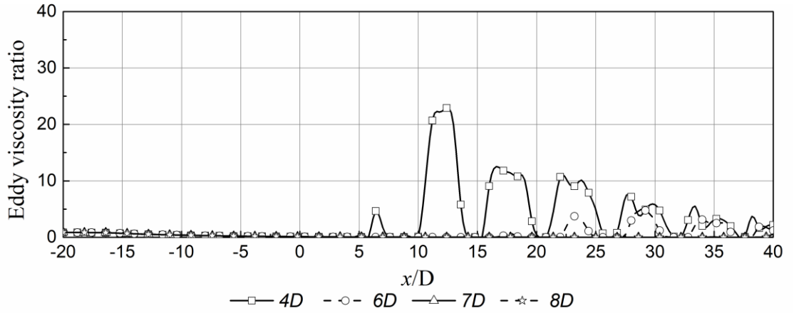
Figure 3.4.17 Turbulent viscosity of (Re, A/D, Fr) = (2300, 0.2, 1.1) along the in-line direction
