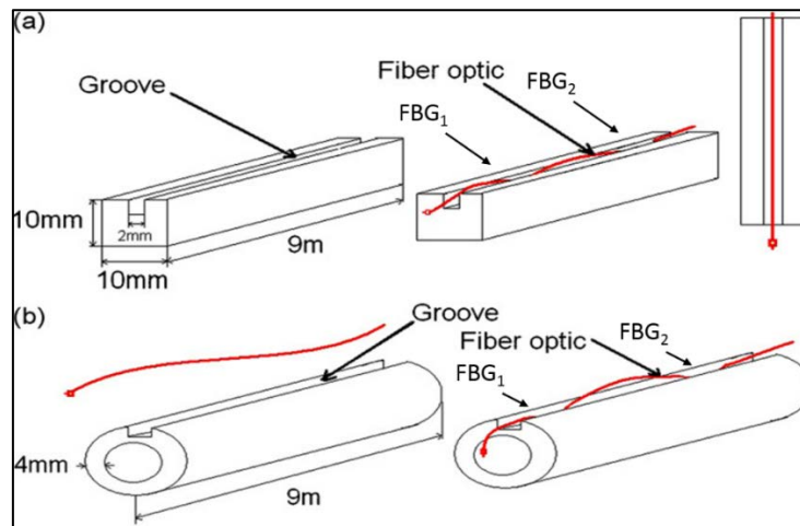
Figure 3.17 Schematic illustration of a sensor protection system using CFRP material (a) FBG installation inside rod (b) CFRP tube with integrated FBGs [161].
