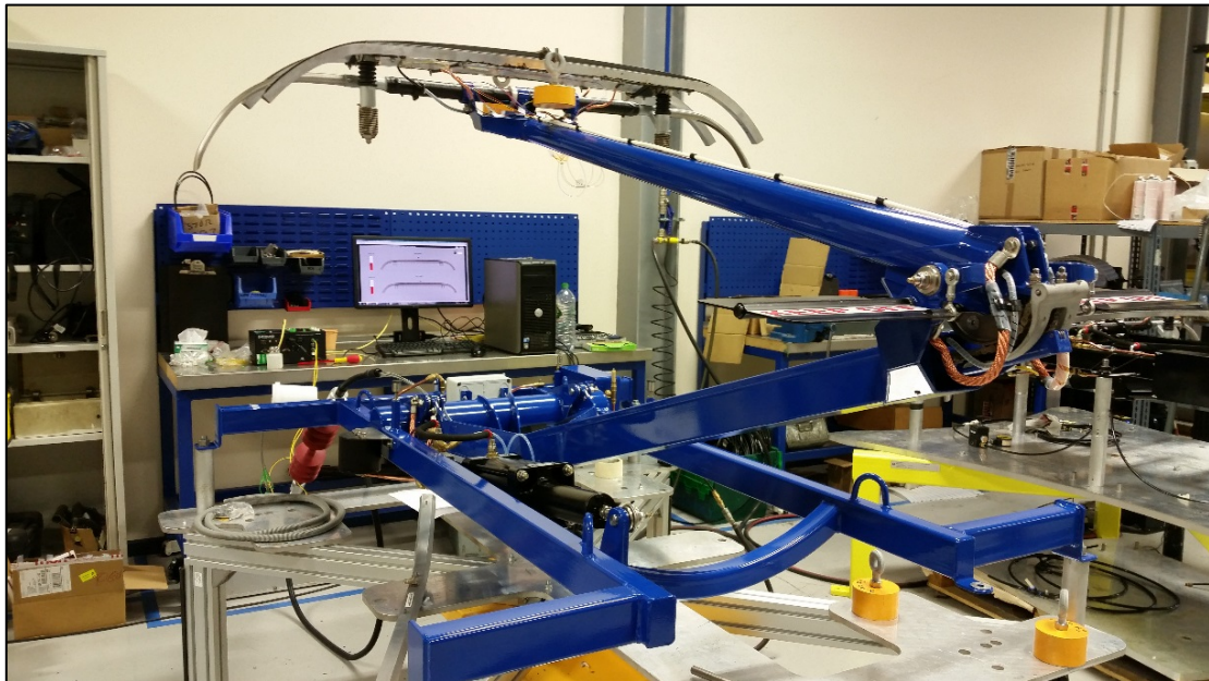
Figure 6.1 Pantograph designed and manufactured at Brecknell Willis
