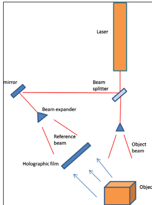
Figure 2.8 Typical holographic experimental setup [52]
