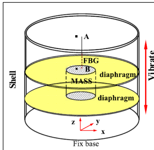
Figure 3.29 Schematic structure FBG accelerometer based on double diaphragms reported by Liu et al [181].
