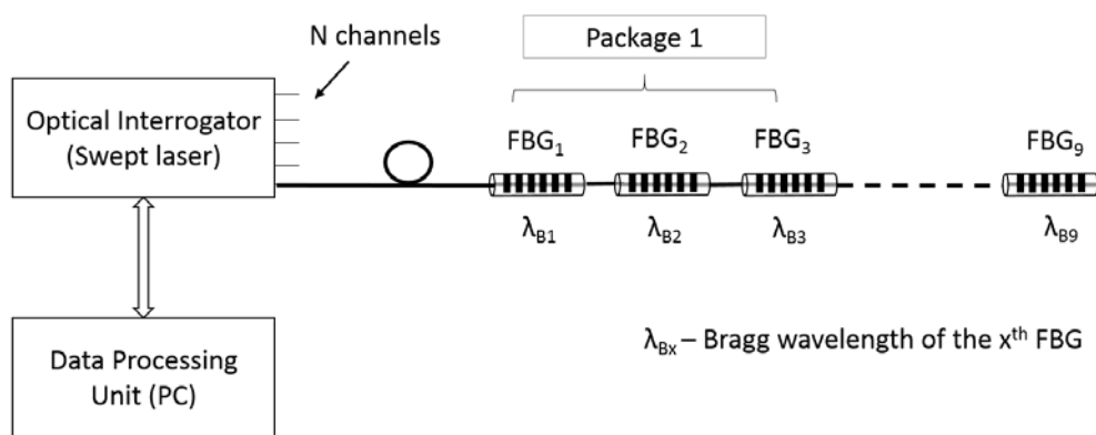
Figure 6.4 Demonstration of an FBG array used for pantograph instrumentation and interrogation setup
