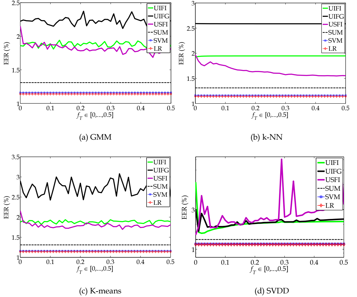
Figure 4.8. Combining two biometric matchers of the XM2VTS LP1 database: The average EER (%) of UIFI, UIFG, and USFI when applied in conjunction with various one-class classifiers, is plotted as a function of the fraction rejection f_T \in [0, \dots, 0.5] . The schemes are also compared with state-of-the-art techniques, such as SUM, SVM and LR.
