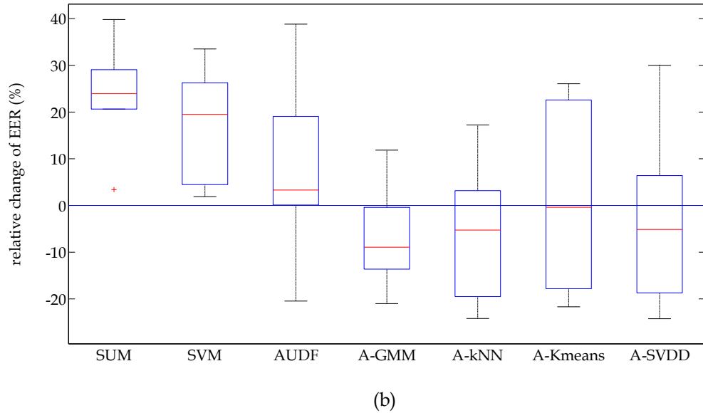
Figure 5.4. Combining three biometric matchers of the BioSecure DS2 database: (a) Average EER (%) for different learning settings (i.e., fraction rejection f_T , and trade-off parameter \alpha ), (b) Relative change of EER (%) across 6 combination possibilities of SUM, SVM, AUDF ( \alpha = 0.7 ), A-GMM ( f_T = 0.01 ), A-kNN ( f_T = 0.01 ), A-Kmeans ( f_T = 0.42 ) and A-SVDD ( f_T = 0.01 ) with respect to LR.
