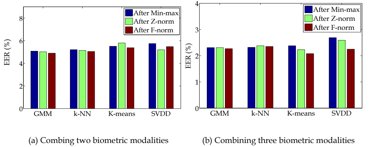
Figure 4.13. EER (%) of various one-class classification methods, as applied to train the user-specific score fusion when the Min-max, Z-norm and F-norm are used prior to fusion.
