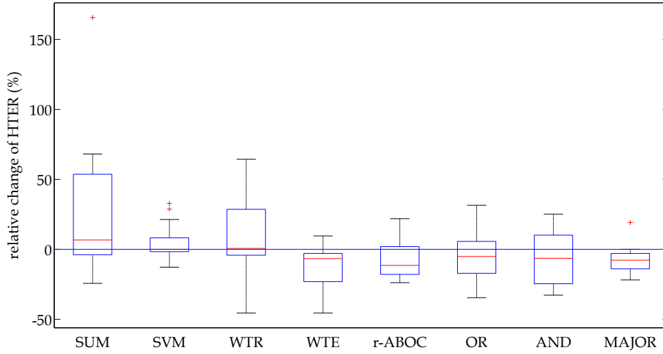
Figure 5.7. Combining two biometric matchers of the XM2VTS LP1 database: (a) Average HTER (%) as a function of the number of weak classifiers, used in classifier ensembles, (b) Relative change of HTER (%) across 15 combination possibilities of SUM, SVM, WTR, WTE, r-ABOC, OR ( T = 3 ), AND ( T = 38 ), and MAJOR ( T = 21 ) with respect to LR.
