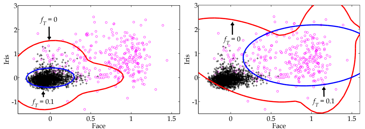
Figure 4.6. User-independent descriptions around (a) the impostor class, and (b) the genuine user class, learned by GMM with various values of f_T . The continuous red (blue) lines correspond to the descriptions learned with f_T = 0 ( f_T = 0.1 ).
