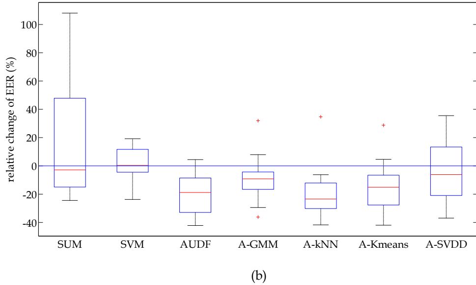
Figure 5.2. Combining two biometric matchers of the XM2VTS LP1 database: (a) Average EER (%) for different learning settings (i.e., fraction rejection f_T , and trade-off parameter \alpha ), (b) Relative change of EER (%) across 15 combination possibilities of SUM, SVM, AUDF ( \alpha = 0.6 ), A-GMM ( f_T = 0.02 ), A-kNN ( f_T = 0.03 ), A-Kmeans ( f_T = 0.43 ) and A-SVDD ( f_T = 0.06 ) with respect to LR.
