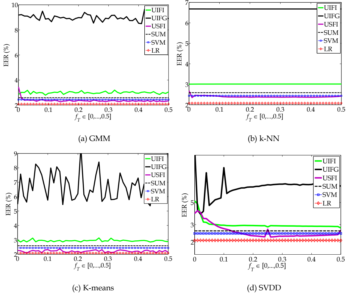
Figure 4.10. Combining three biometric matchers of the BioSecure DS2 database: The average EER (%) of UIFI, UIFG, and USFI when applied in conjunction with various one-class classifiers, is plotted as a function of the fraction rejection f_T \in [0, \dots, 0.5] . The schemes are also compared with state-of-the-art techniques, such as SUM, SVM and LR.
