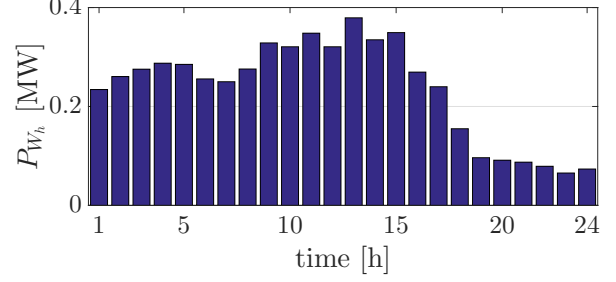
Fig. 4: Hourly wind output for cluster \mathcal{C}_{W_1} .
