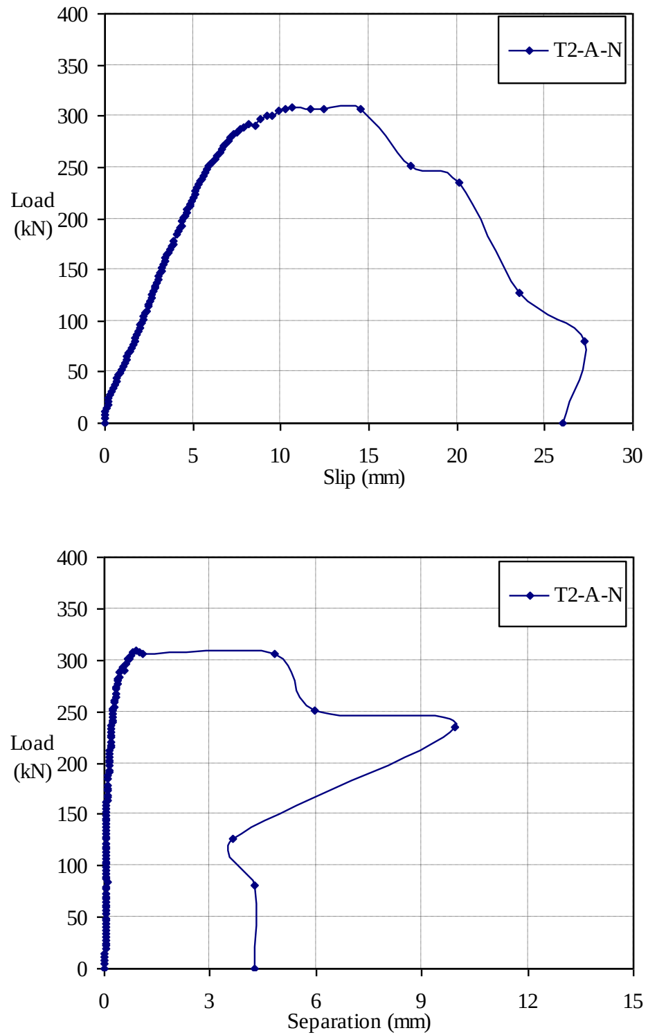
Figure 3.21 Load-slip and load-separation curves of specimen T2-A-N ( \varnothing 150\text{mm} web opening, normal concrete)
