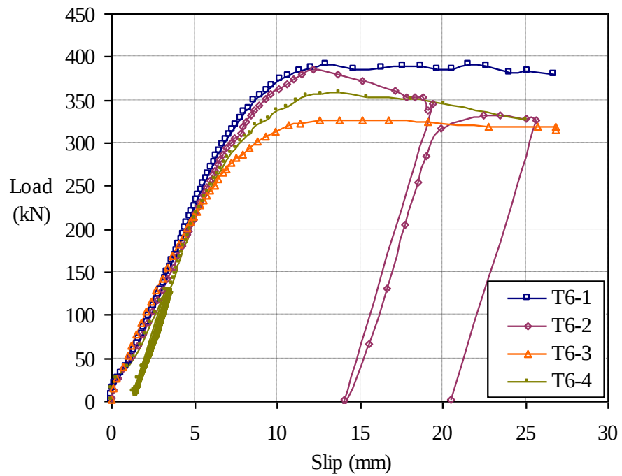
Figure 4.6 Load-slip curves of the tie-bar (Ø16mm) shear connection (test group T6)
