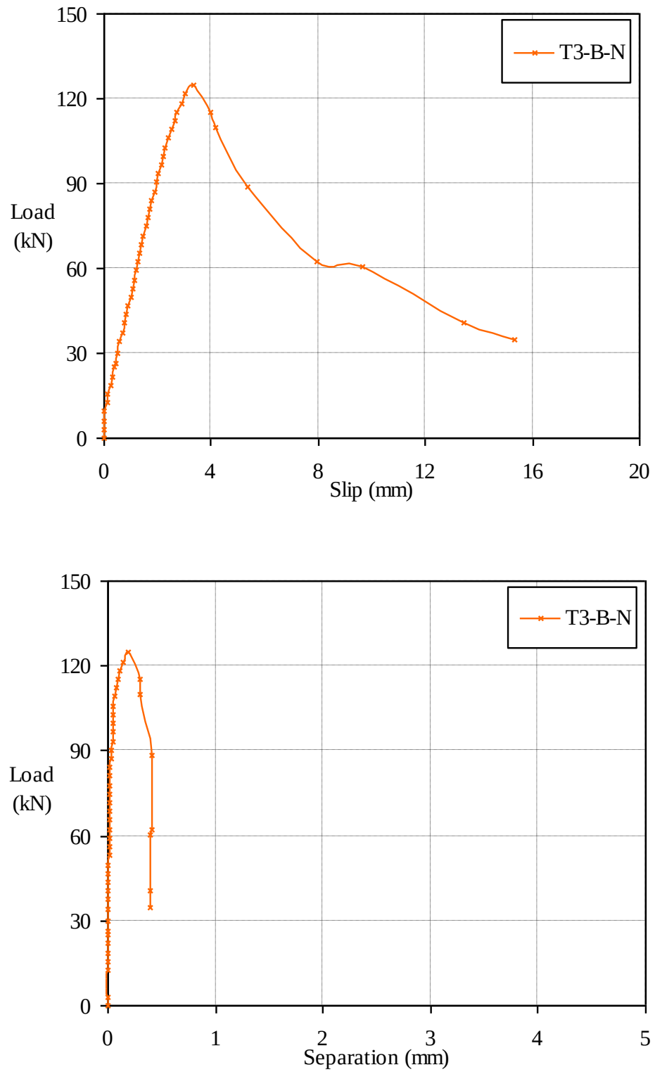
Figure 3.29 Load-slip and load-separation curves of specimen T3-B-N (Ø200mm web opening, Ø150mm ducting, normal concrete)
