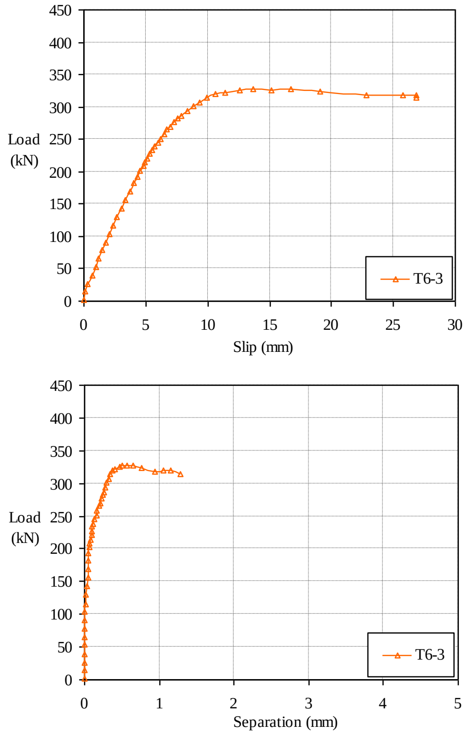
Figure 4.18 Load-slip and load-separation curves of specimen T6-3
