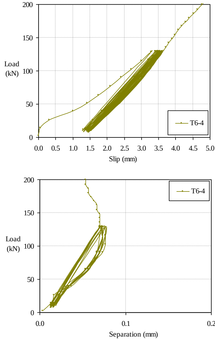
Figure 4.20 Load-slip and load-separation response of the tie-bar (Ø16mm) shear connection during the loading cycles
