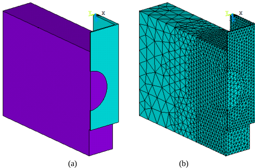
Figure 5.2 FEA model of a 1/4 of the test specimen with one concrete-infill-only shear connection of Ø150mm (a) geometry model, (b) meshed model
