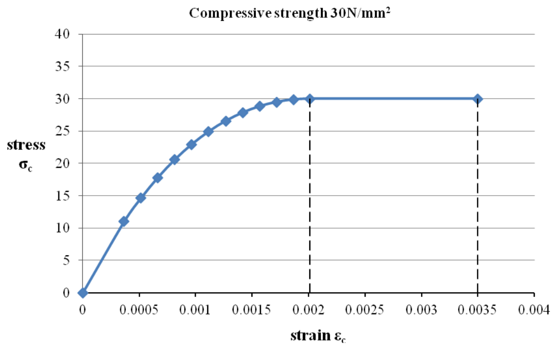
Figure L1 Stress-strain curve for concrete compressive strength of 30N/mm 2
