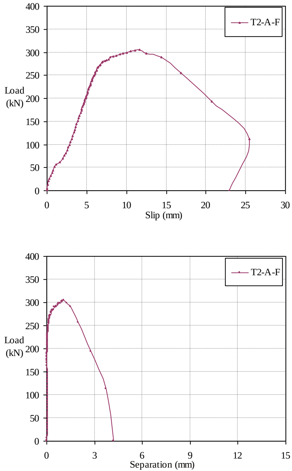
Figure 3.22 Load-slip and load-separation curves of specimen T2-A-F (Ø150mm web opening, fibre-reinforced concrete)
