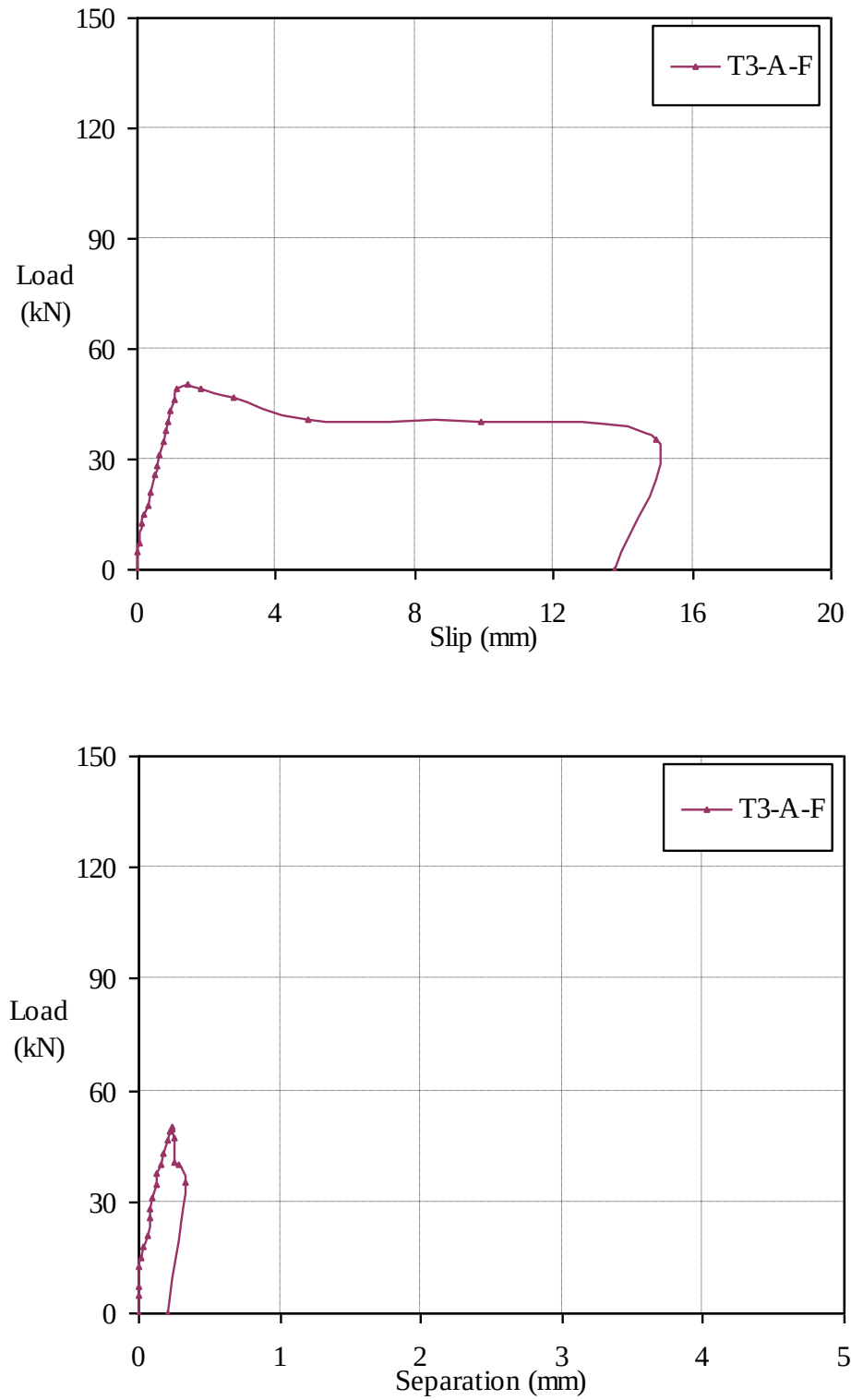
Figure 3.28 Load-slip and load-separation curves of specimen T3-A-F ( \varnothing 150\text{mm} web opening, \varnothing 125\text{mm} ducting, fibre-reinforced concrete)
