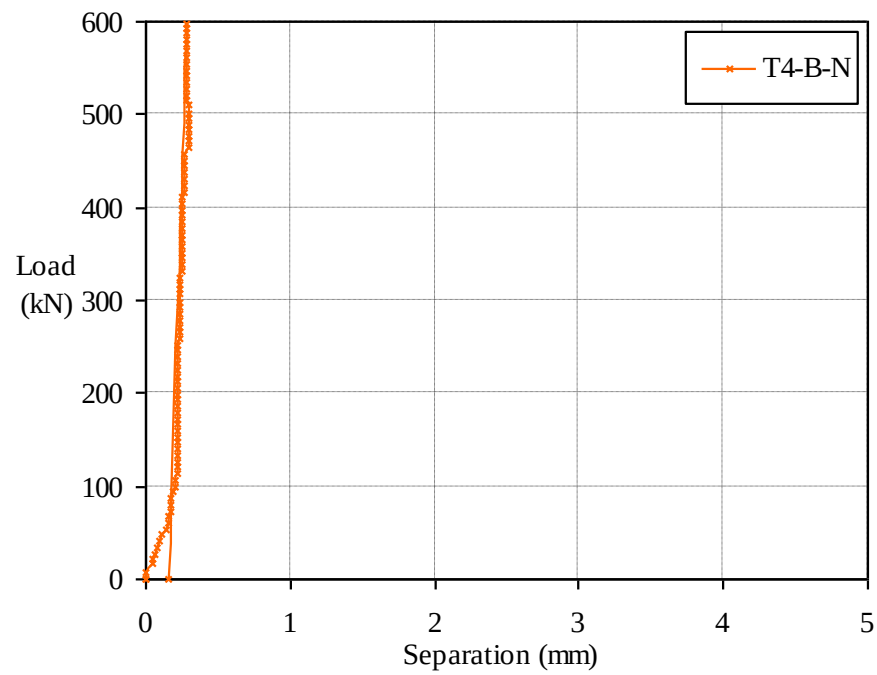
Figure 3.34 Load-slip and load-separation curves of specimen T4-B-N ( \varnothing 200\text{mm} web opening, normal concrete)
