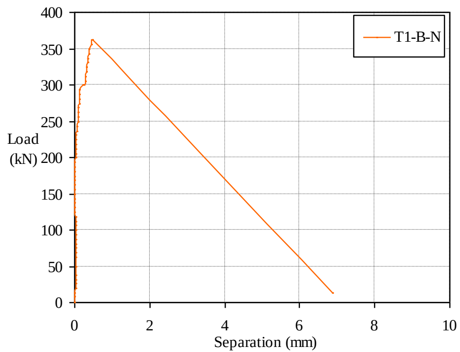
Figure 3.18 Load-slip and load-separation curves of specimen T1-B-N (Ø200mm web opening, normal concrete)
