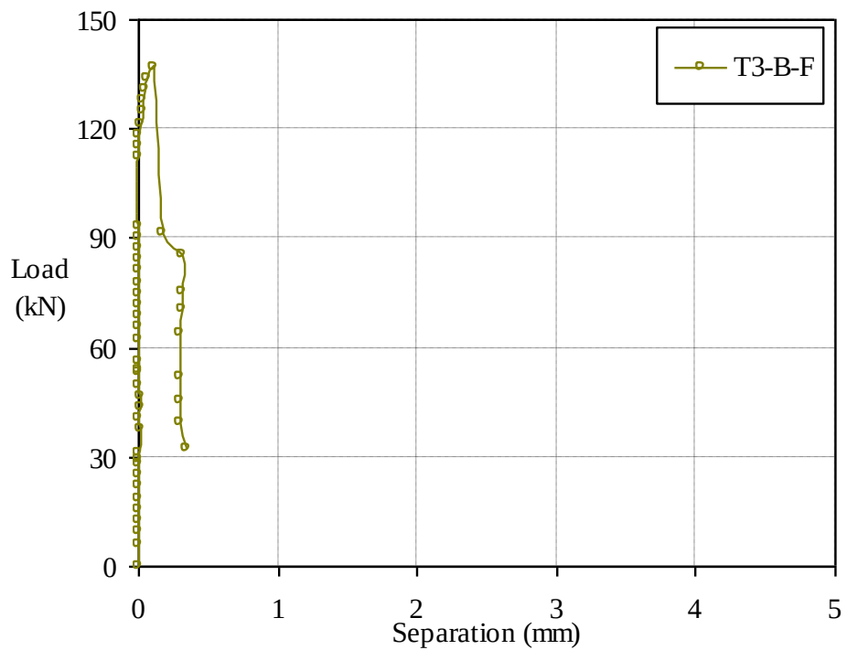
Figure 3.30 Load-slip and load-separation curves of specimen T3-B-F ( \varnothing 200 mm web opening, \varnothing 150 mm ducting, fibre-reinforced concrete)
