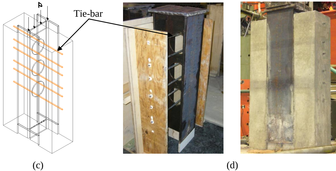
Figure 3.4 Drawings of the T2 specimens: (a) with Ø150mm web openings, (b) with Ø200mm web openings, (c) Schematic of the T2 specimens, (d) Cast test specimens
