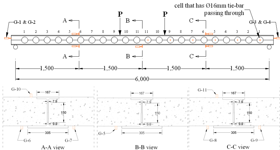
Figure 6.18 Locations of slip instrumentation and labels of the dial gauges
