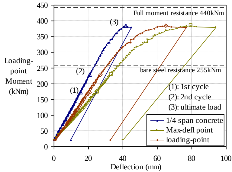
Figure 6.30 Deflections of the three-point asymmetric bending test
