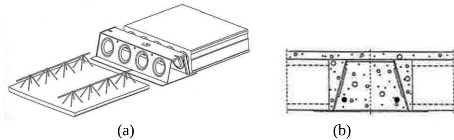
Figure 2.8 (a) Schematic of the Deltabeam; (b) Cross-section of the Deltabeam (Peltonen and Leskelä(2004)
