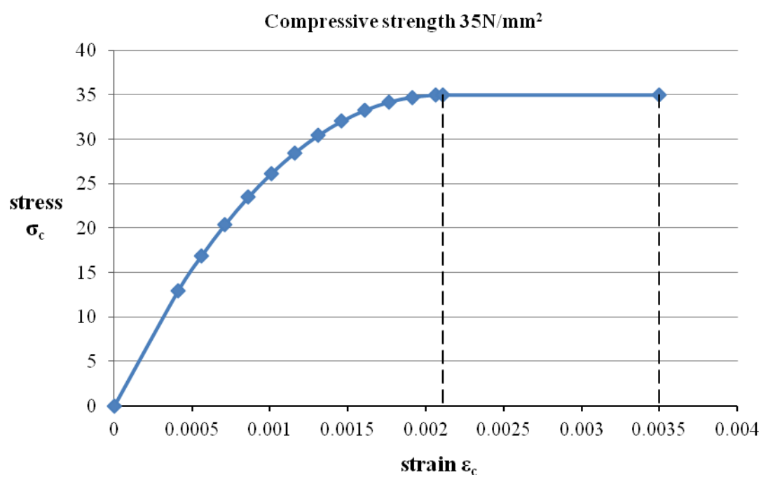
Figure L3 Stress-strain curve for concrete compressive strength of 35N/mm 2
