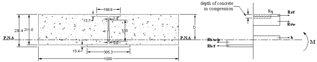
Figure G-4 Stress block diagram of the cross section in degree of shear connection of 0.7
