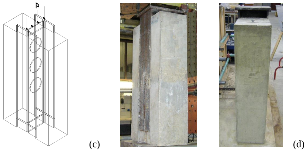
Figure 3.3 Drawings of the T1 specimens: (a) with \varnothing 150\text{mm} web openings, (b) with \varnothing 200\text{mm} web openings, (c) Schematic of the T1 specimens, (d) Cast test specimens
