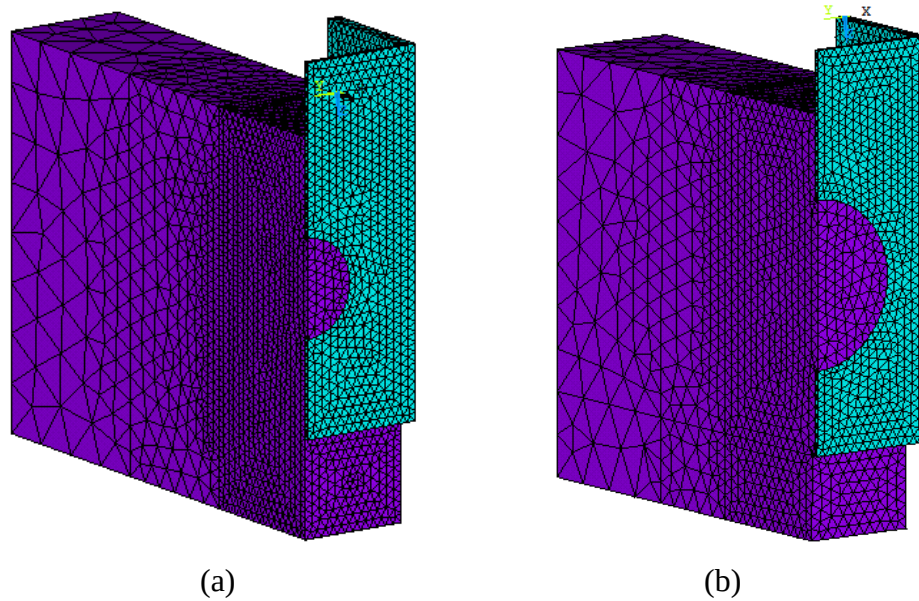
Figure 5.12 FEA models of the concrete-infill-only shear connection with web opening diameters of (a) 100mm, (b) 200mm
