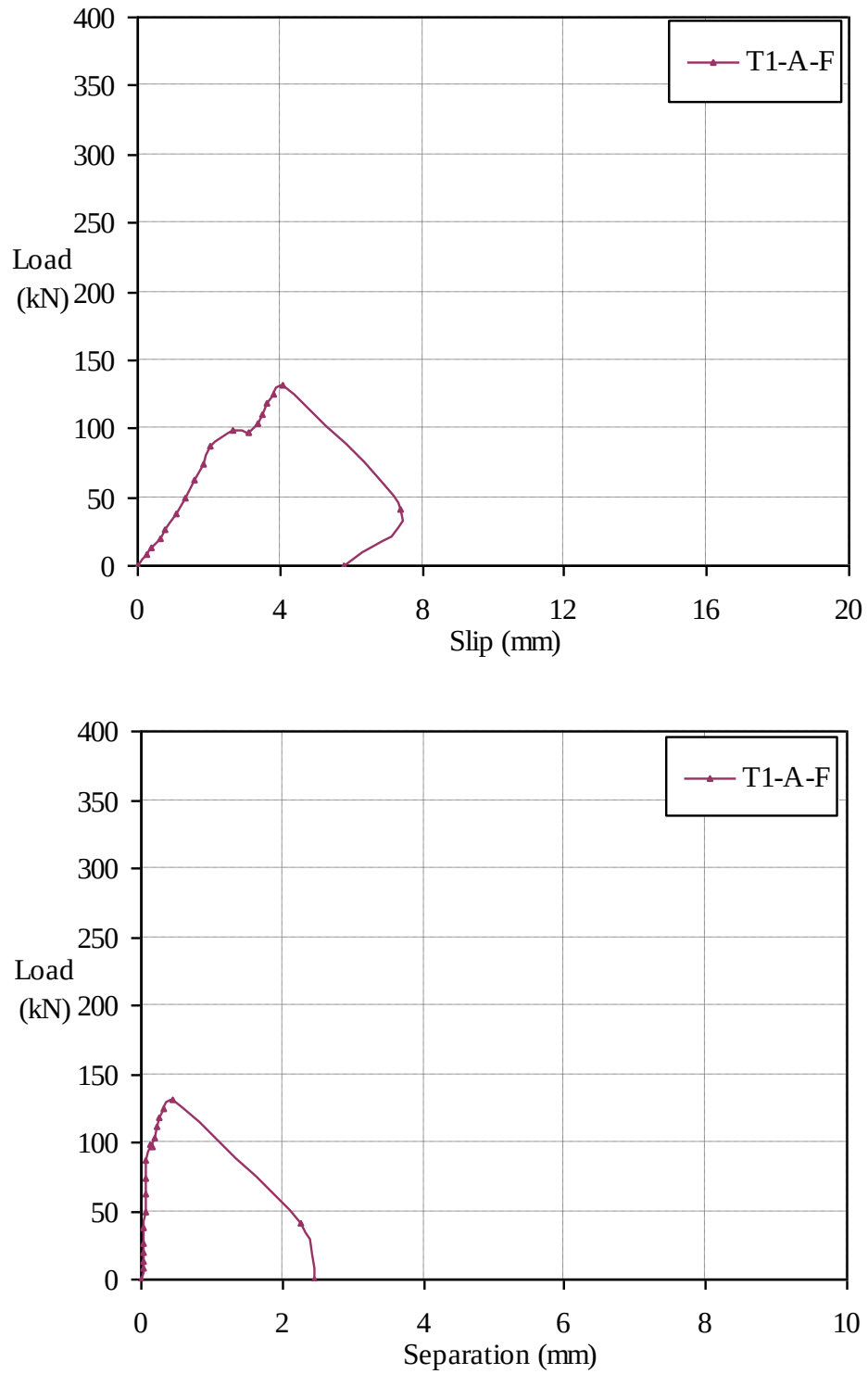
Figure 3.17 Load-slip and load-separation curves of specimen T1-A-F (Ø150mm web opening, fibre-reinforced concrete)
