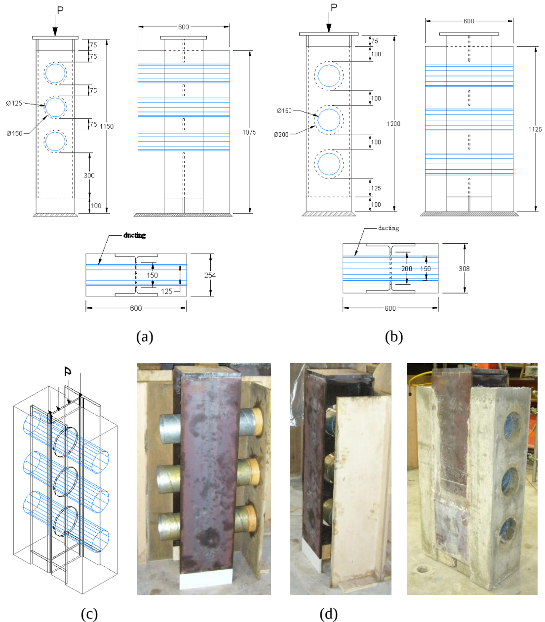
Figure 3.5 Drawings of the T3 specimens (a): with Ø150mm web openings, (b): with Ø200mm web openings; (c) Schematic of the T3 specimens; (d): Cast test specimens
