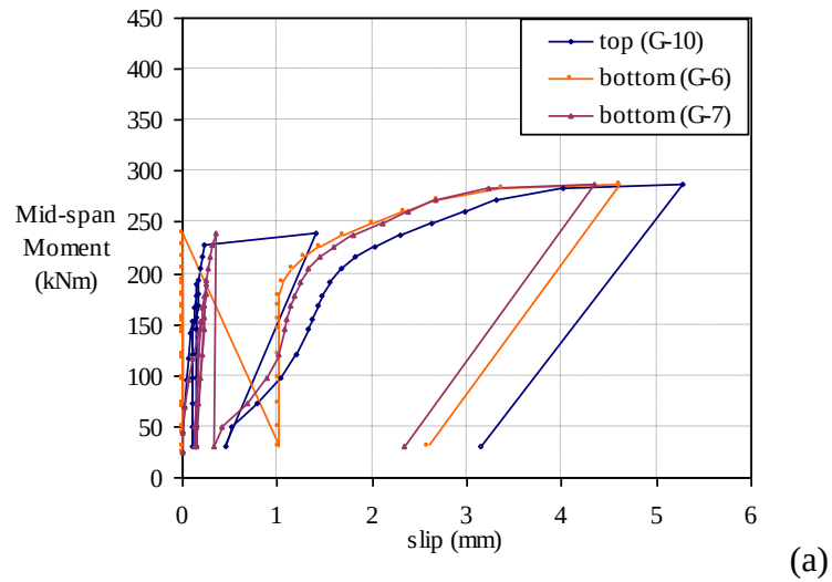
Figure 6.21 (a) End-span slip curves of the right shear span with the combination of shear connection; (b) Comparison of the slips between the two shear spans
