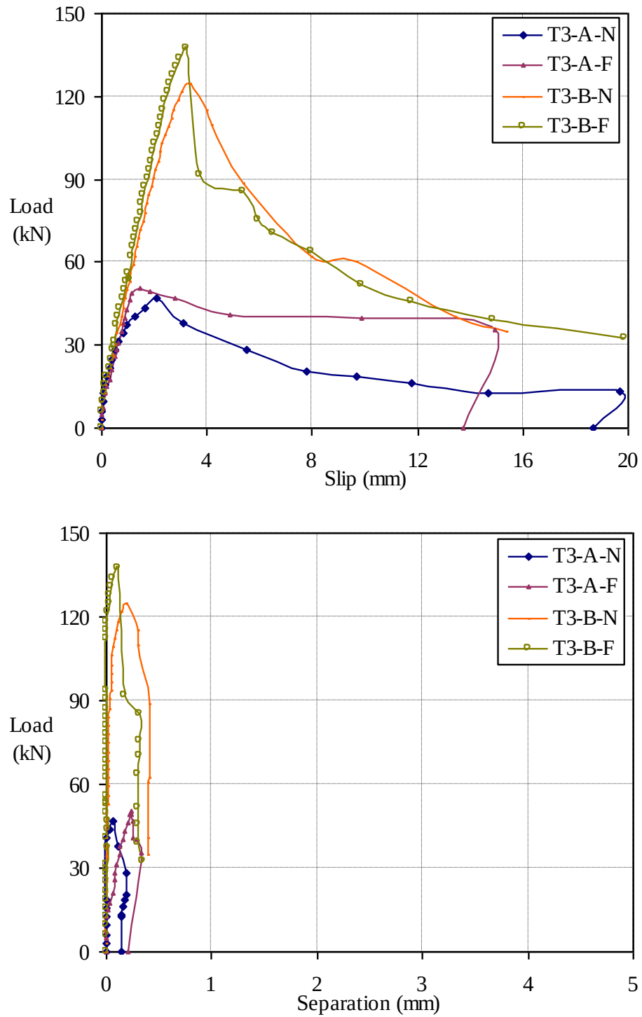
Figure 3.26 Load-slip and load-separation curves of the ducting shear connection
