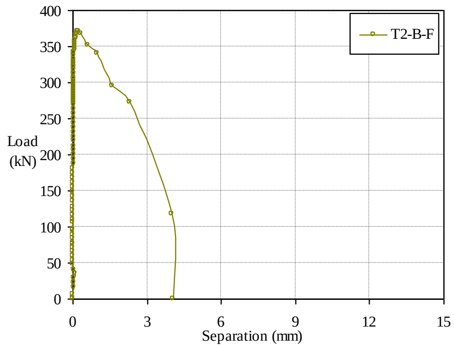
Figure 3.24 Load-slip and load-separation curves of specimen T2-B-F ( \varnothing 200 mm web opening, fibre-reinforced concrete)
