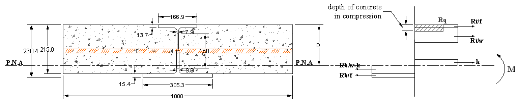
Figure J-4 Stress block diagram of the cross section in degree of shear connection of 0.7
