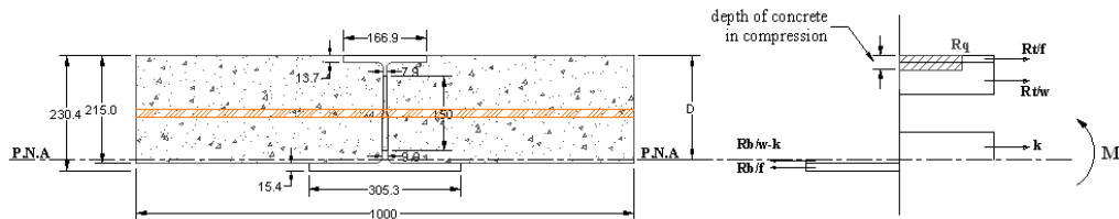
Figure J-3 Stress block diagram of the cross section in degree of shear connection of 0.5
