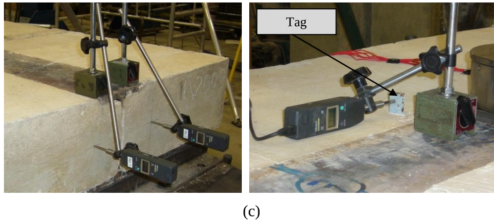
Figure 6.6 Instrumentation for deflections and slips: (a) measuring locations, (b) deflection instrumentation, (c) slip instrumentation
