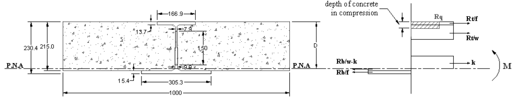
Figure G-3 Stress block diagram of the cross section in degree of shear connection of 0.5
