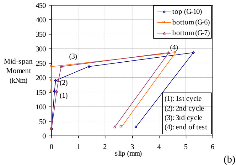
Figure 6.22 Quarter-span slips of the left shear span with the concrete-infill-only shear connection: (a) slip curves, (b) slips reached at different loading stages
