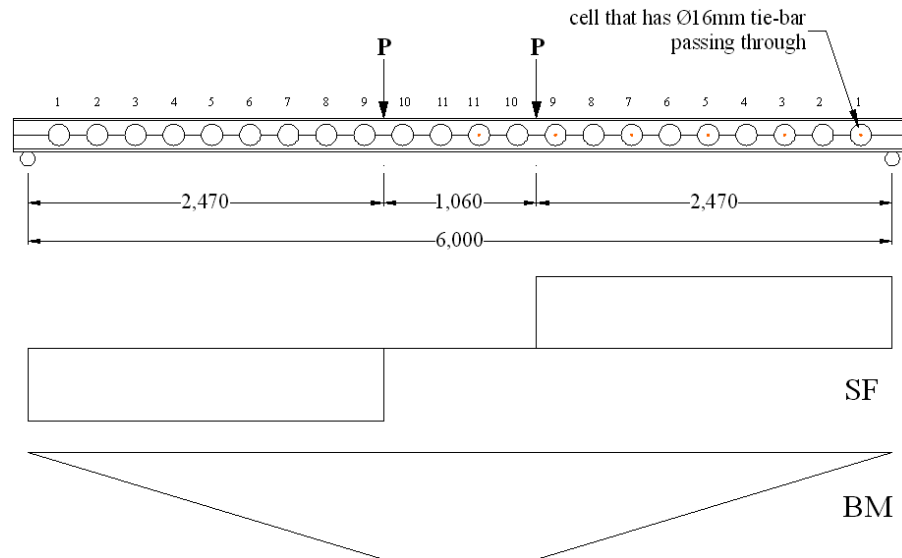
Figure 6.4 Loading position, shear force and bending moment diagrams of the four-point symmetric bending test
