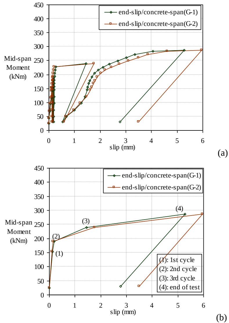
Figure 6.20 End-span slip curves of the left shear span with the concrete-infill-only shear connection: (a) slip curves, (b) slips reached at different loading stages
