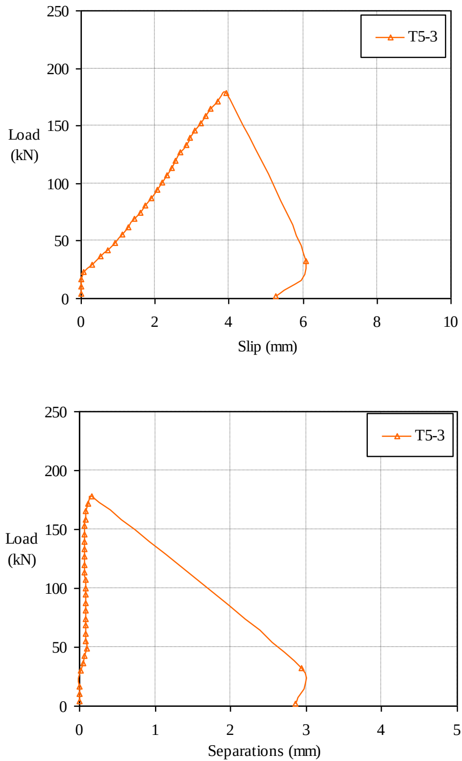
Figure 4.12 Load-slip and load-separation curves of specimen T5-3
