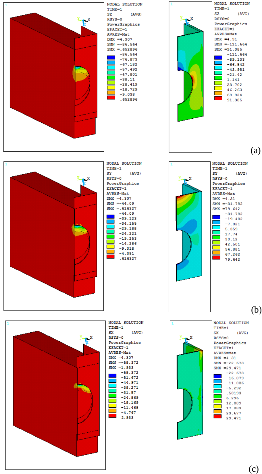
(a) Compression (vertical direction), (b) y-direction stress in line with web post, (c) Separation (x-direction)
