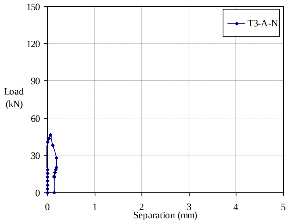
Figure 3.27 Load-slip and load-separation curves of specimen T3-A-N ( \varnothing 150\text{mm} web opening, \varnothing 125\text{mm} ducting, normal concrete)
