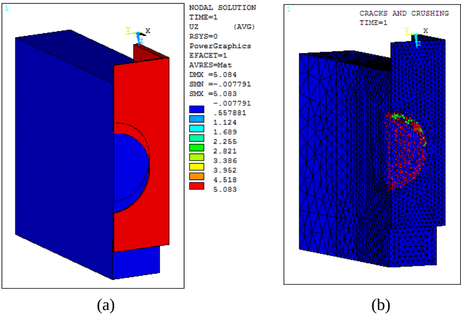
(a) Contour plot of vertical displacement (slips); (b) Contour plot of cracks
