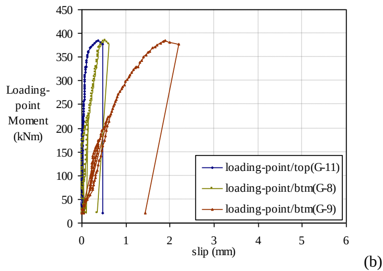
Figure 6.38 (a) End slips of the shorter shear span with the combined shear connection; (b) Slips at the loading point
