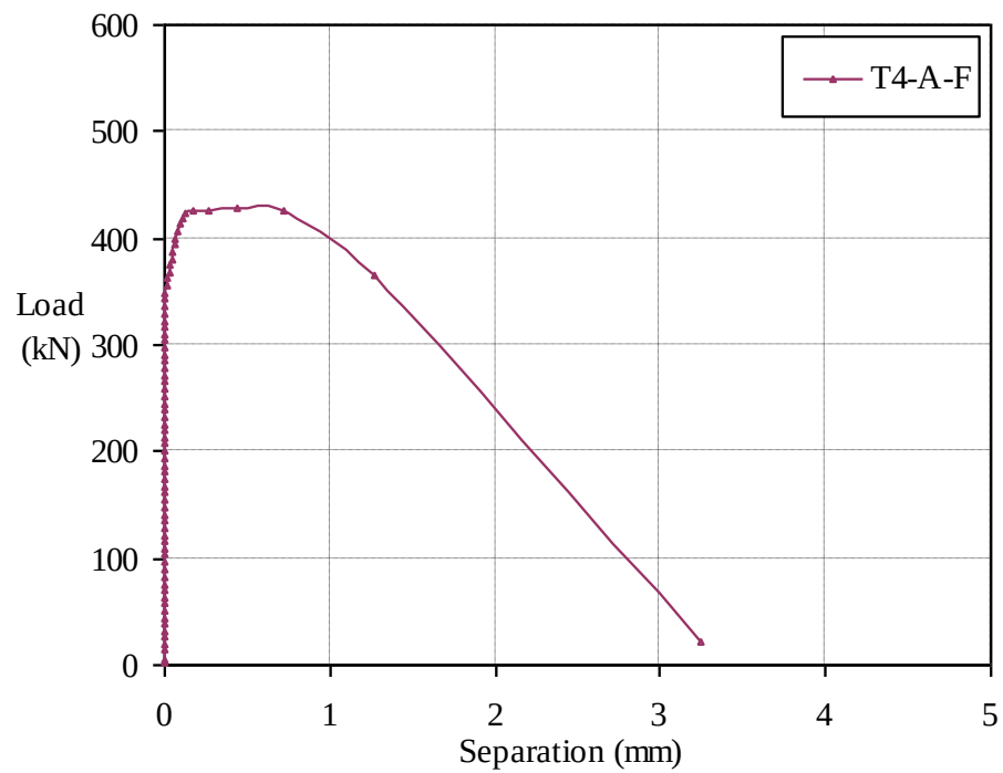
Figure 3.33 Load-slip and load-separation curves of specimen T4-A-F ( \varnothing 150 mm web opening, fibre-reinforced concrete)
