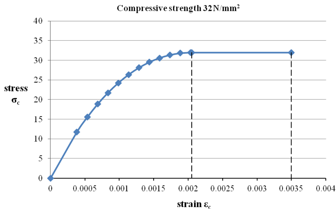
Figure L2 Stress-strain curve for concrete compressive strength of 32N/mm 2
