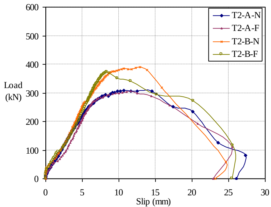
Figure 3.9 Load-slip curves of the tie-bar shear connection (test group T2)
