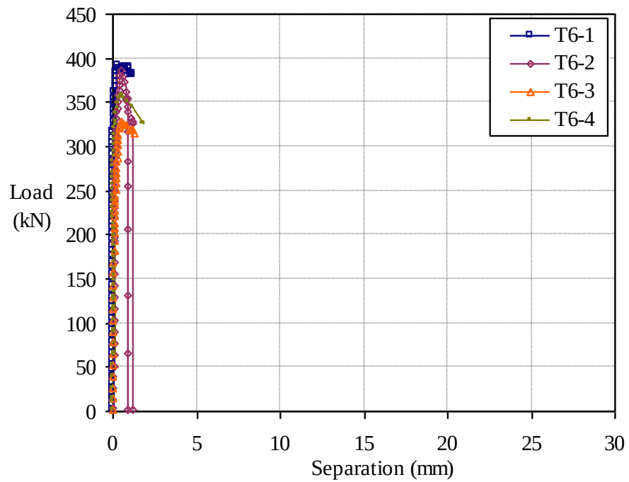
Figure 4.8 Load-separation curves of the tie-bar (Ø16mm) shear connection (T6)
