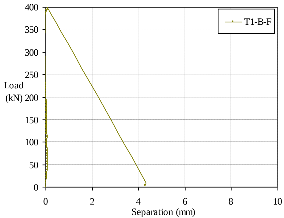
Figure 3.19 Load-slip and load-separation curves of specimen T1-B-F ( \varnothing 200 mm web opening, fibre-reinforced concrete)
