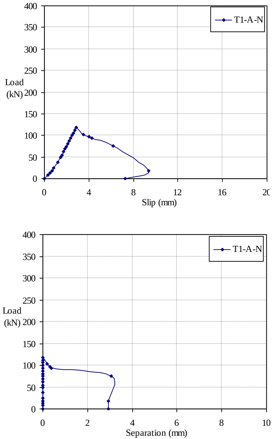
Figure 3.16 Load-slip and load-separation curves of specimen T1-A-N ( \varnothing 150\text{mm} web opening, normal concrete)
