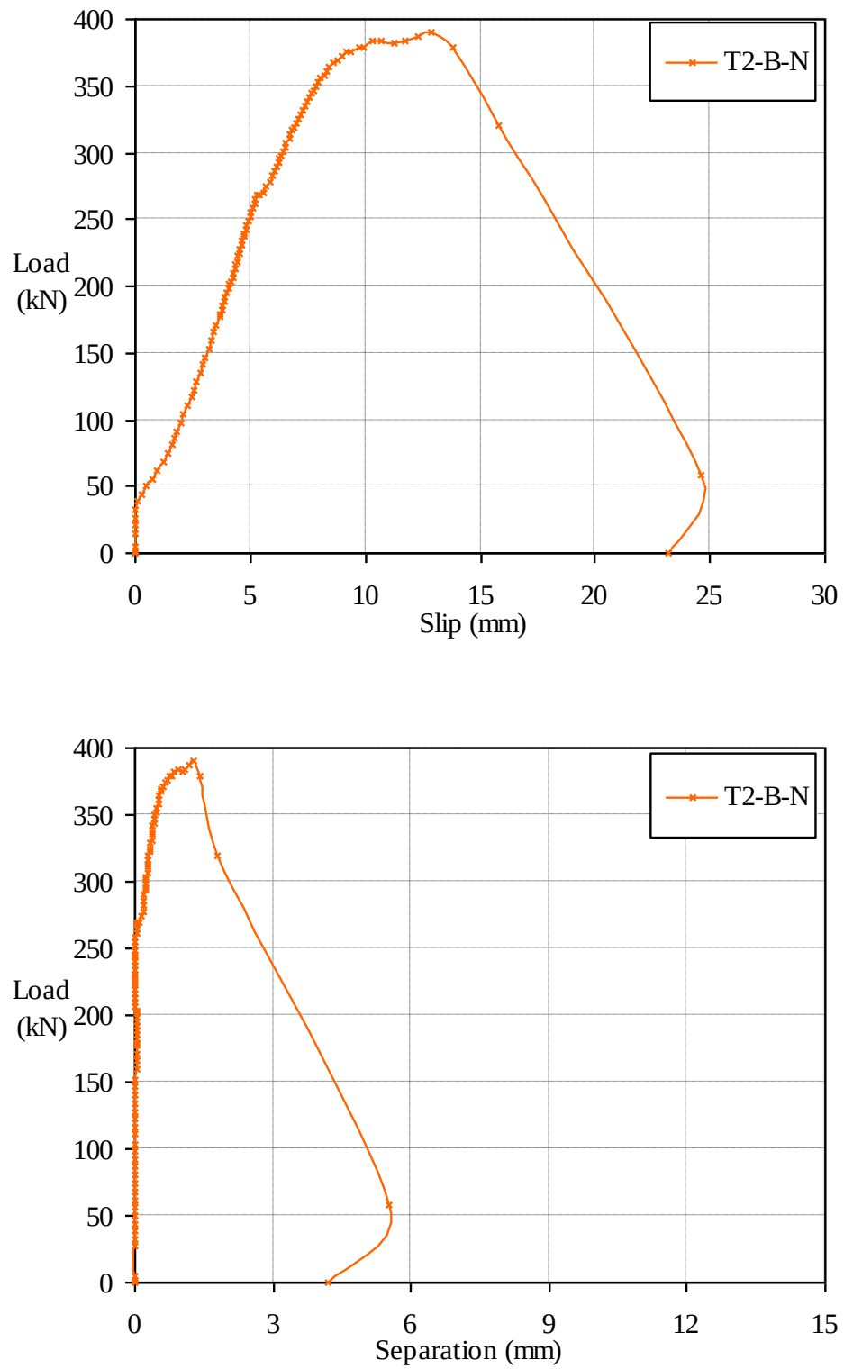
Figure 3.23 Load-slip and load-separation curves of specimen T2-B-N (Ø200mm web opening, normal concrete)
