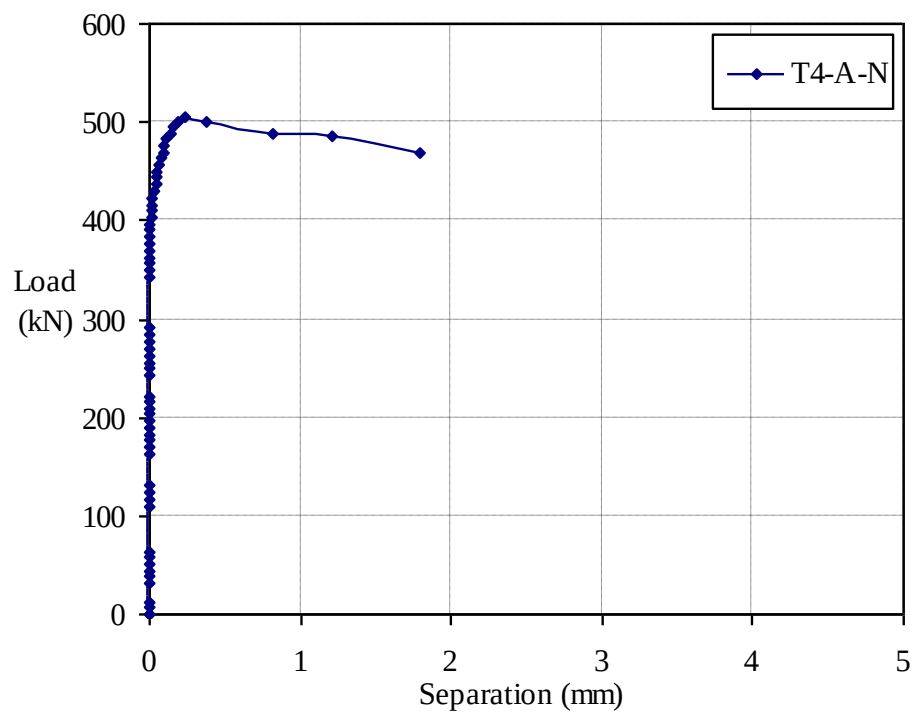
Figure 3.32 Load-slip and load-separation curves of specimen T4-A-N (Ø150mm web opening, normal concrete)
