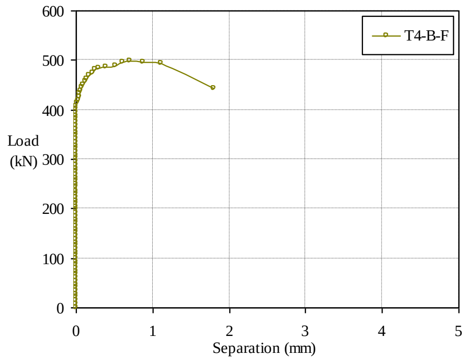
Figure 3.35 Load-slip and load-separation curves of specimen T4-B-F ( \varnothing 200 mm web opening, fibre-reinforced concrete)
