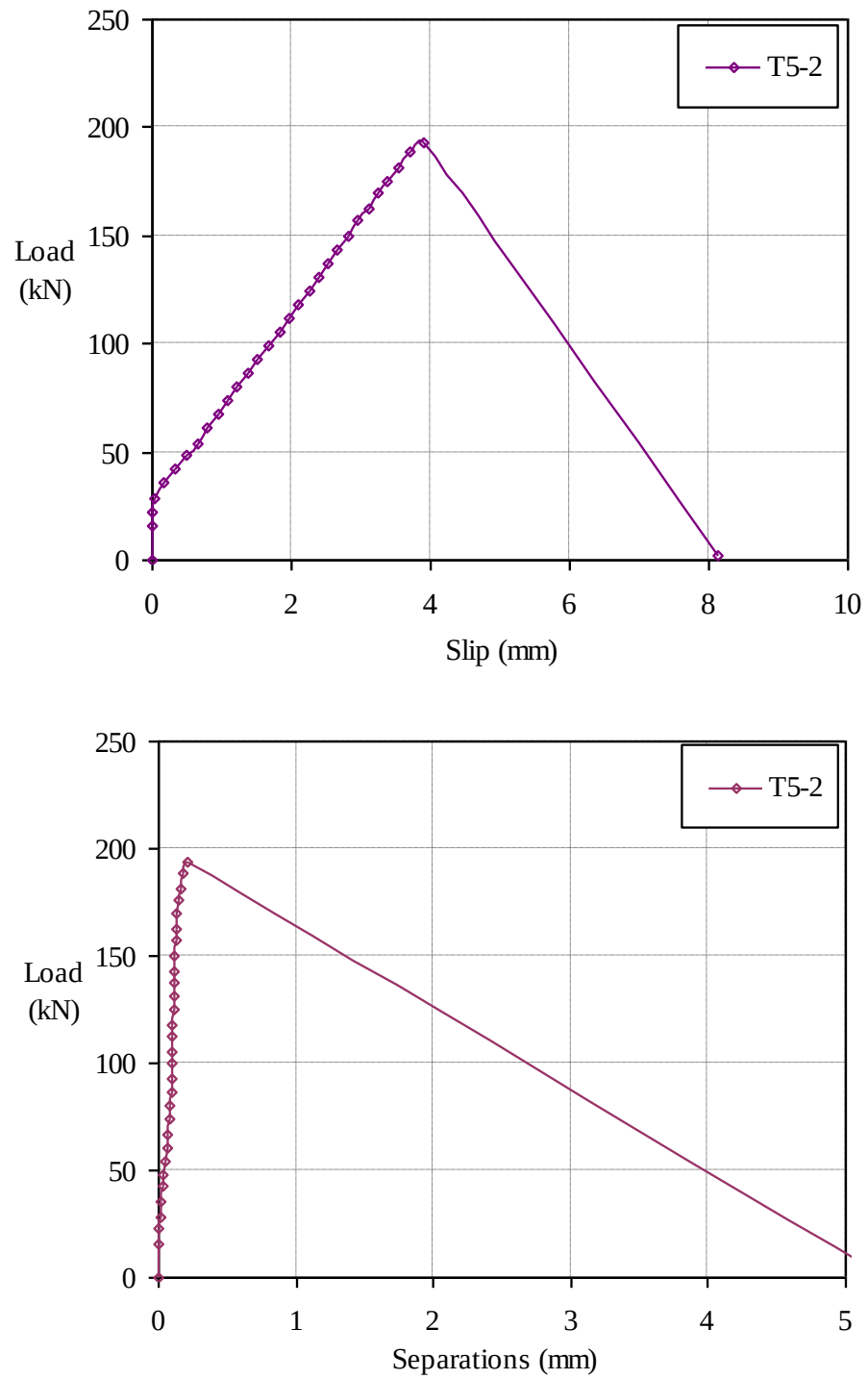
Figure 4.11 Load-slip and load-separation curves of specimen T5-2
