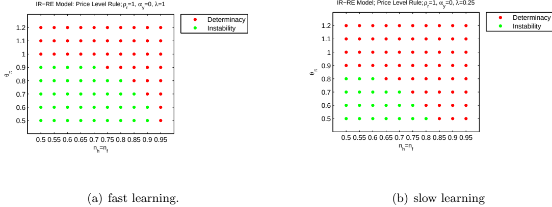
Figure 4: Stability of RE-IR heterogeneous-agent model with price-level rule under fast and slow learning.
