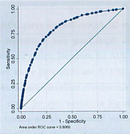
AUC = 0.8060 (a)
