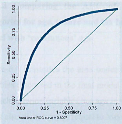
AUC = 0.8007 (a)
