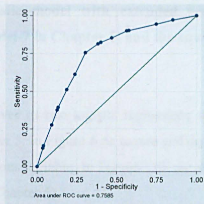
AUC = 0.7585 (b)
