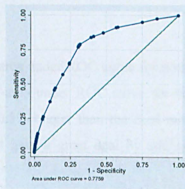
AUC = 0.7759 (b)
