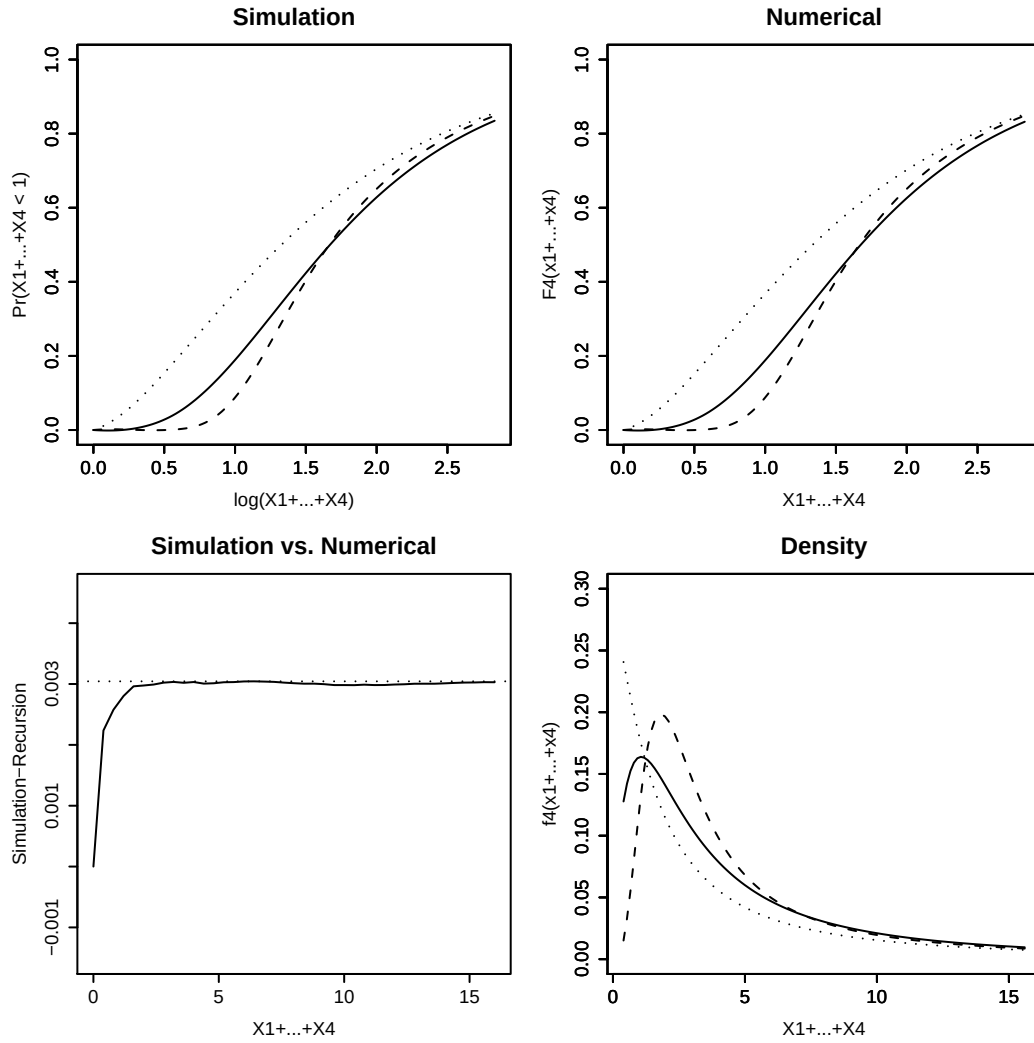
Figure 3.4 \rho = -0.7 (dashed), \rho = 0 (solid), \rho = 0.7 (dotted). Top left: aggregate distributions of X_1 + \dots + X_4 with Gaussian copula and Pareto( \alpha = 0.9, \beta = 0.4 ) marginal distributions by simulation. Top right: aggregate distributions with Gaussian copula and Pareto( \alpha = 0.9, \beta = 0.4 ) marginal distributions by Theorem 3.2. Bottom left: difference between simulation and Theorem 3.2. Bottom right: aggregate density functions by Theorem 3.2.
