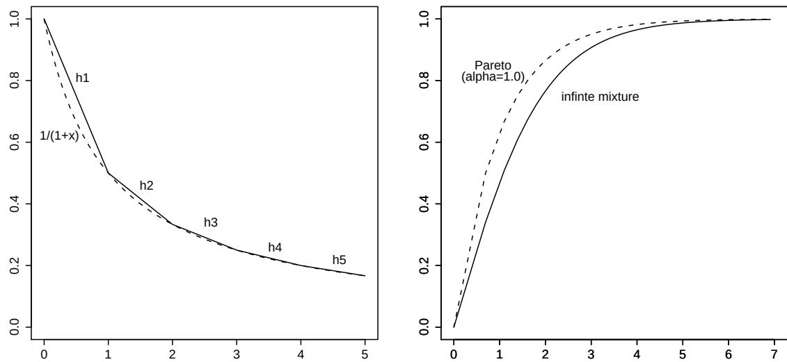
Figure 2.3 Hazard rate functions and the distribution functions of the infinite mixture(solid) and Pareto with \alpha = 1 (dotted).
