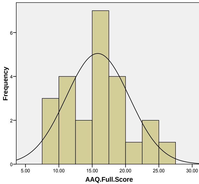
AAQ.Full.Score
