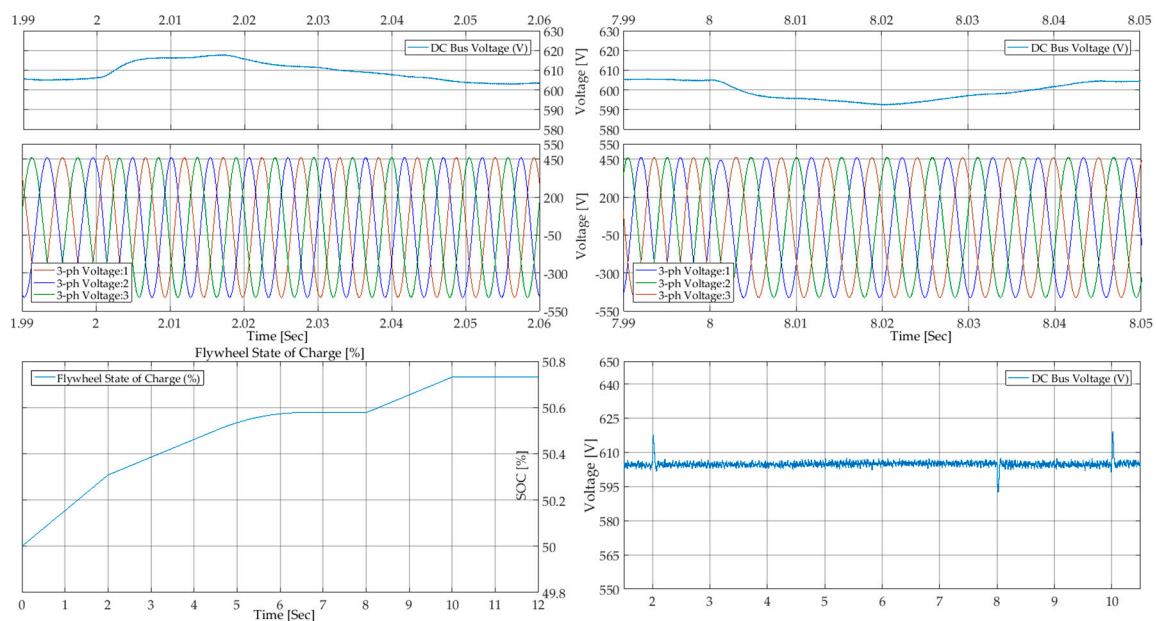
Figure 15. FESS in step-charging mode: Inverter output voltage and DC-bus voltage at ( t = 2 s) (top left); Inverter output voltage and DC-bus voltage at ( t = 8 s) (top right); FESS state-of-charge (bottom left); DC-bus voltage at ( t = 2, 8, \& 10 s) (bottom right).
