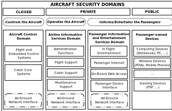
Figure 1. Onboard aircraft network domains (ARINC-811 [6])
