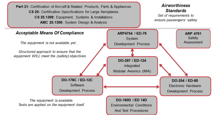
Figure 2. Overview of Safety-Related Development Assurance in Aerospace
