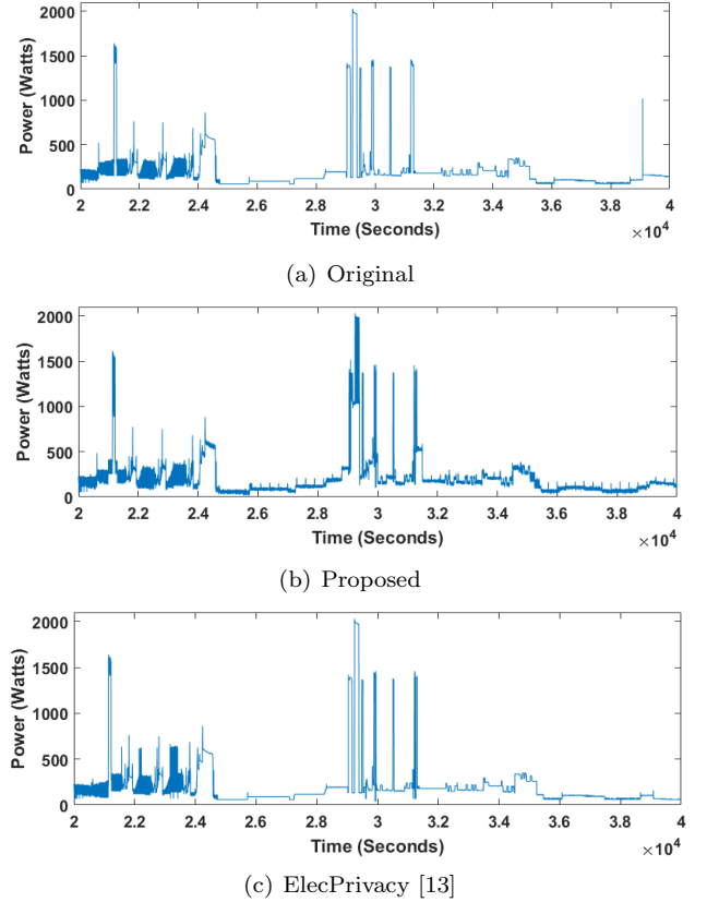
Figure 7: Smart meter reading of a household on 7/06/2012 for comparison between the a) original reading b) after scrambling using the proposed approach c) after scrambling using the existing ElecPrivacy approach.
