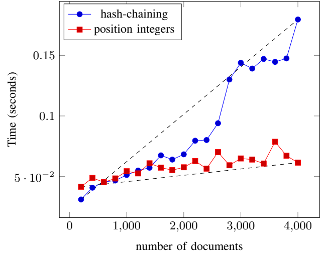
Fig. 2. Search time graph comparing the search time using hash chain technique with the search time using position integers
