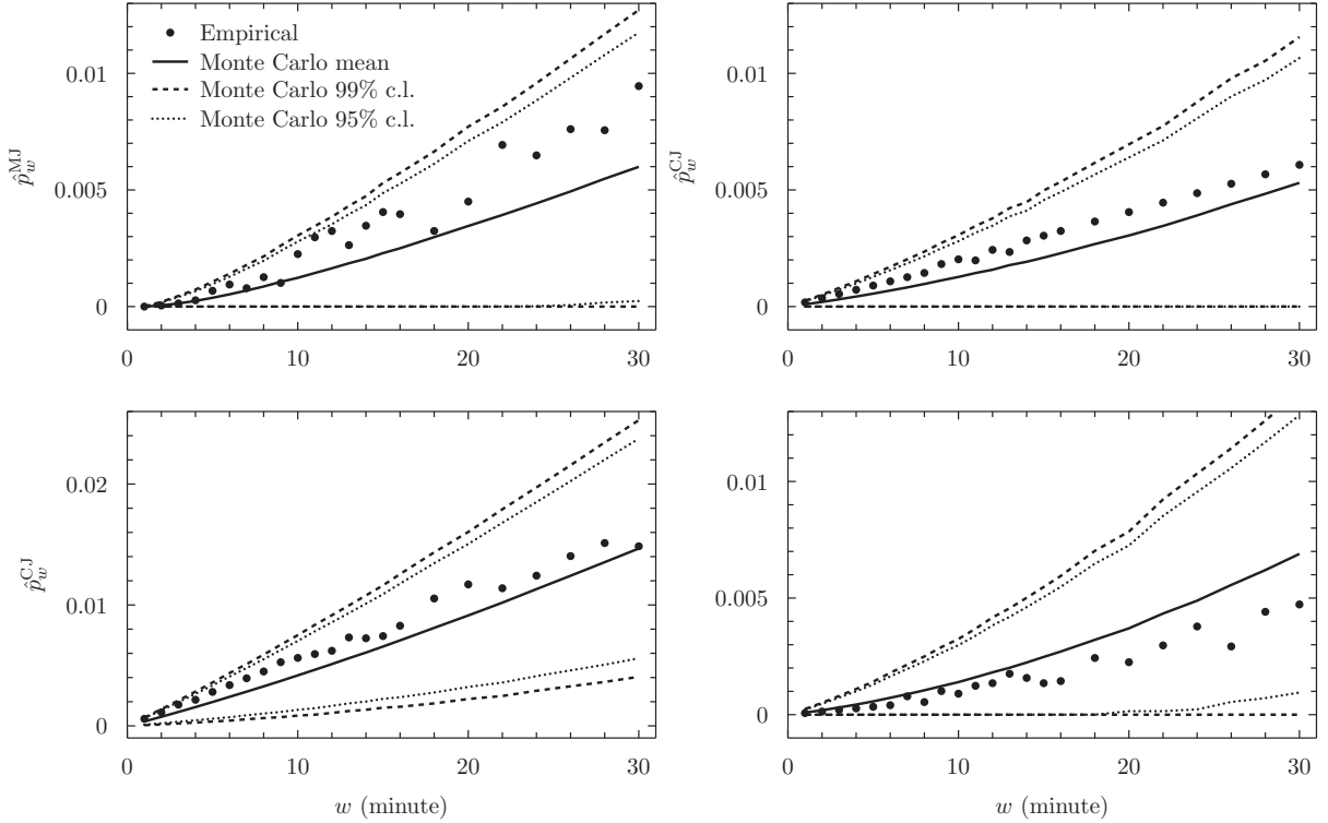
Figure 10: From the top left clockwise: MJ probability test under N factor model null for the asset Generali; CJ probability test for the pairs Generali-Mediobanca, Generali-Banca Popolare Milano, and Generali-Intesa Sanpaolo.
