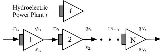
Fig. 1: Schematic representation of a hydroelectric power system.
