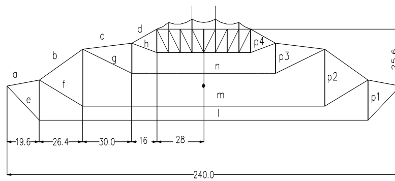
d. Section 1-1
