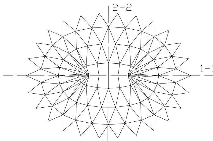
b. Plan of Diagonal and Hoop Cables
