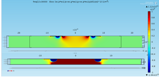
Fig.3: Simulated spatial sensitivity distribution for Prb1 (top) and Prb2 (bottom) indicating the regions of positive (red) and negative contributions (blue).
