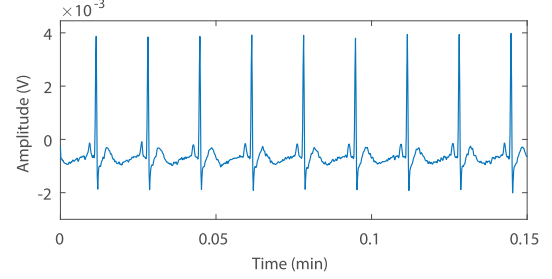
Fig. 10. ECG signal acquired from the ECG amplifier. The ECG leads were attached to a simulator configured to provide a simulated sinus rhythm of 60 beats per minute.
