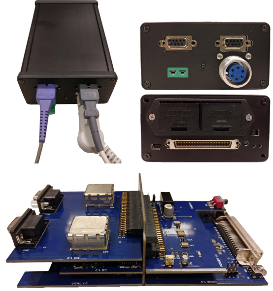
Fig. 6. Photographs showing the front and back panel of the ZenPPG system along with the PCB assembly.
