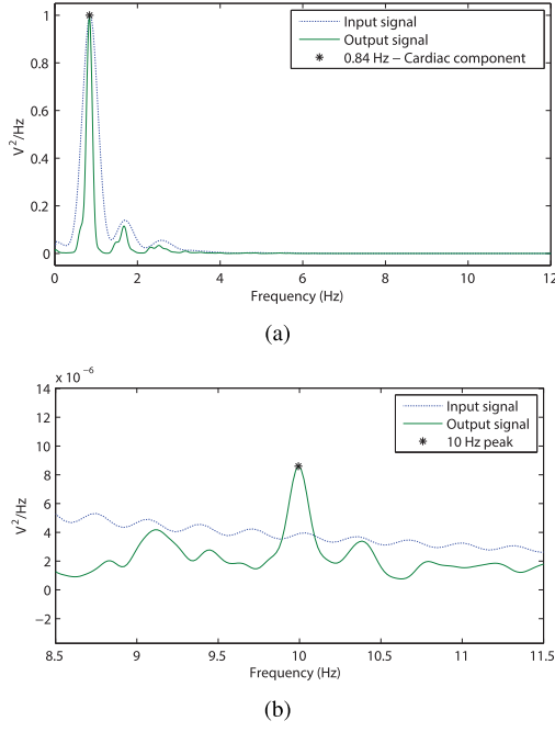
Fig. 8. Frequency spectrum of the input and the output PPG signals showing (a) cardiac and (b) noise components. The 10-Hz noise peak is used to calculate SNR.
