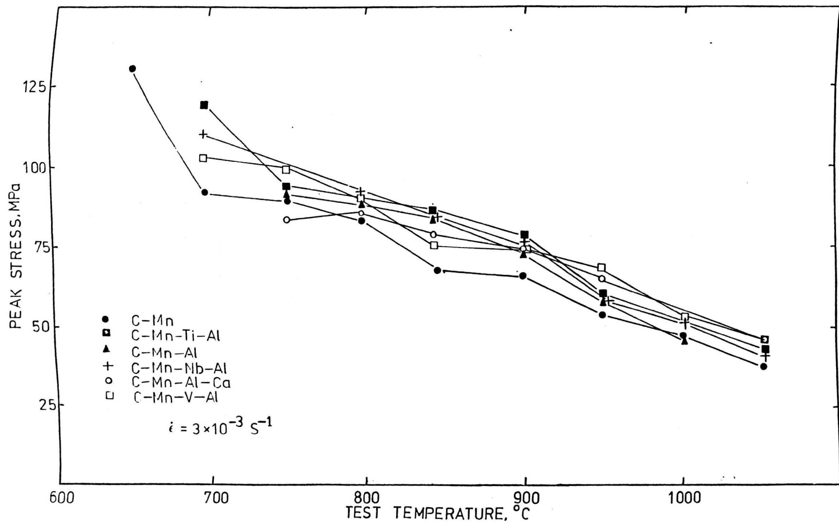
Fig. 10.1 Variation of peak stress with test temperature for six steels heated directly to test temperature
