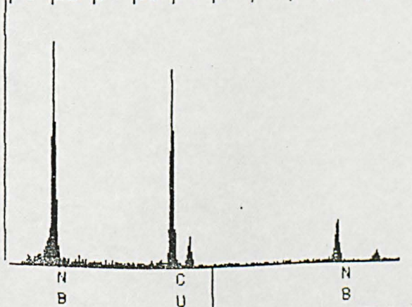
Fig.9.10 Coarse NbCN extracted from 'as cast' sample tested at 950°C, with associated X-ray spectrum.
