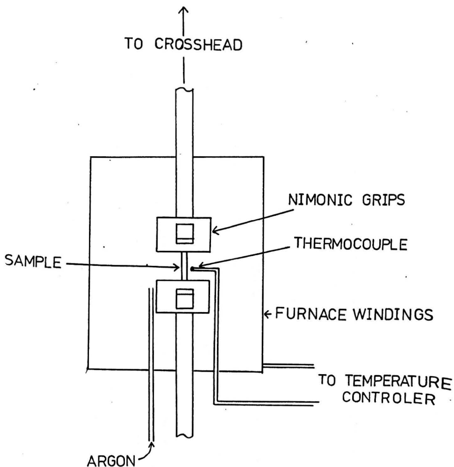
Fig.3.4 Schematic illustration of Instron high temperature testing equipment.
