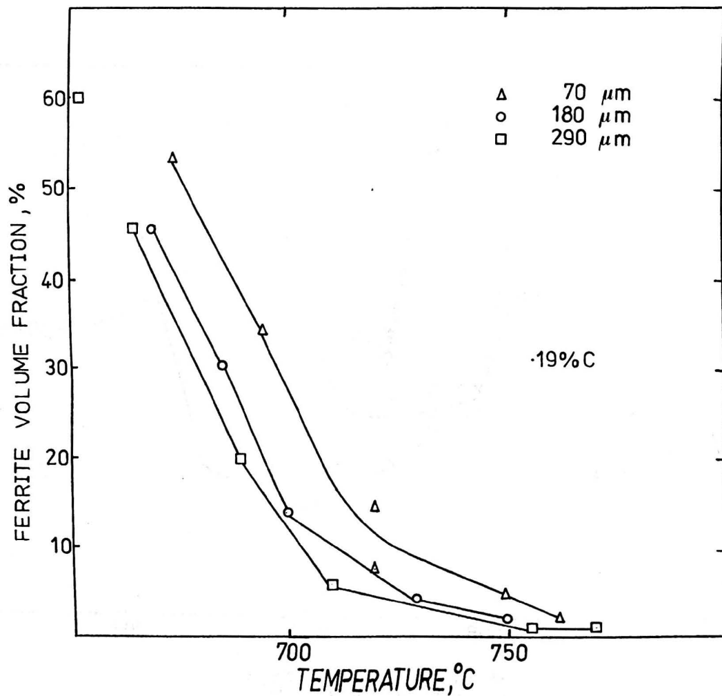
Fig. 5.1 Ferrite volume fraction after quenching small samples of varying initial grain size from various temperatures, .19% C steel.
