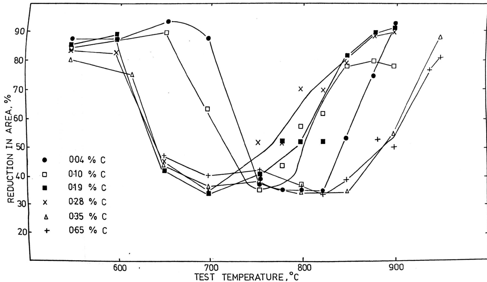
Fig. 4.1 Variation of reduction in area with test temperature for steels 1 - 6
