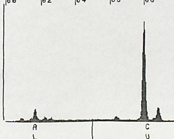
Fig.10.19 AlN precipitation in C-Mn-Al steel tested at 1050°C using a strain rate of 3 \times 10^{-3} \text{ s}^{-1} , with associated X-ray spectrum.
