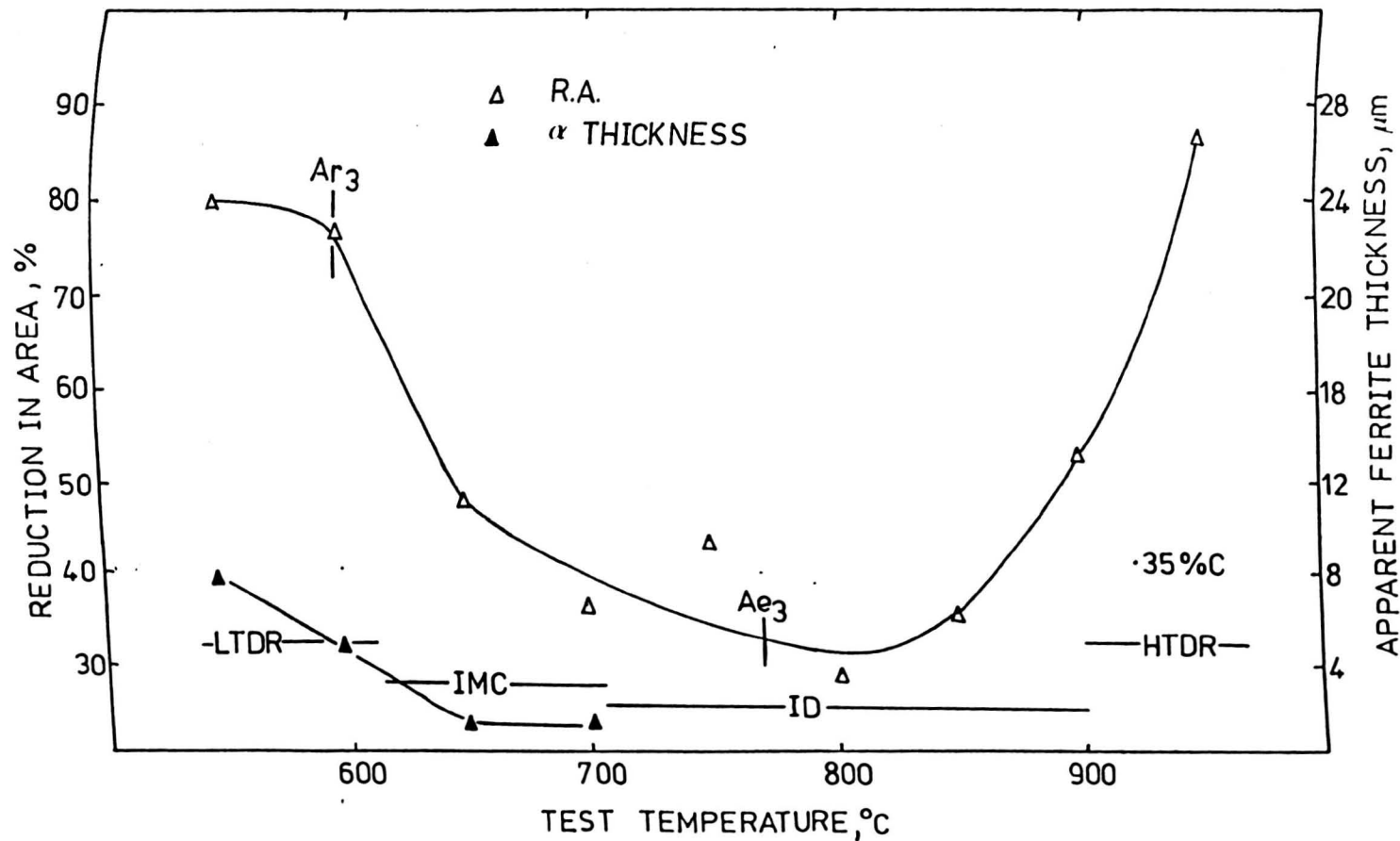
Fig. 4.10 Hot ductility, transformation and fracture data for the 0.35% C steel
