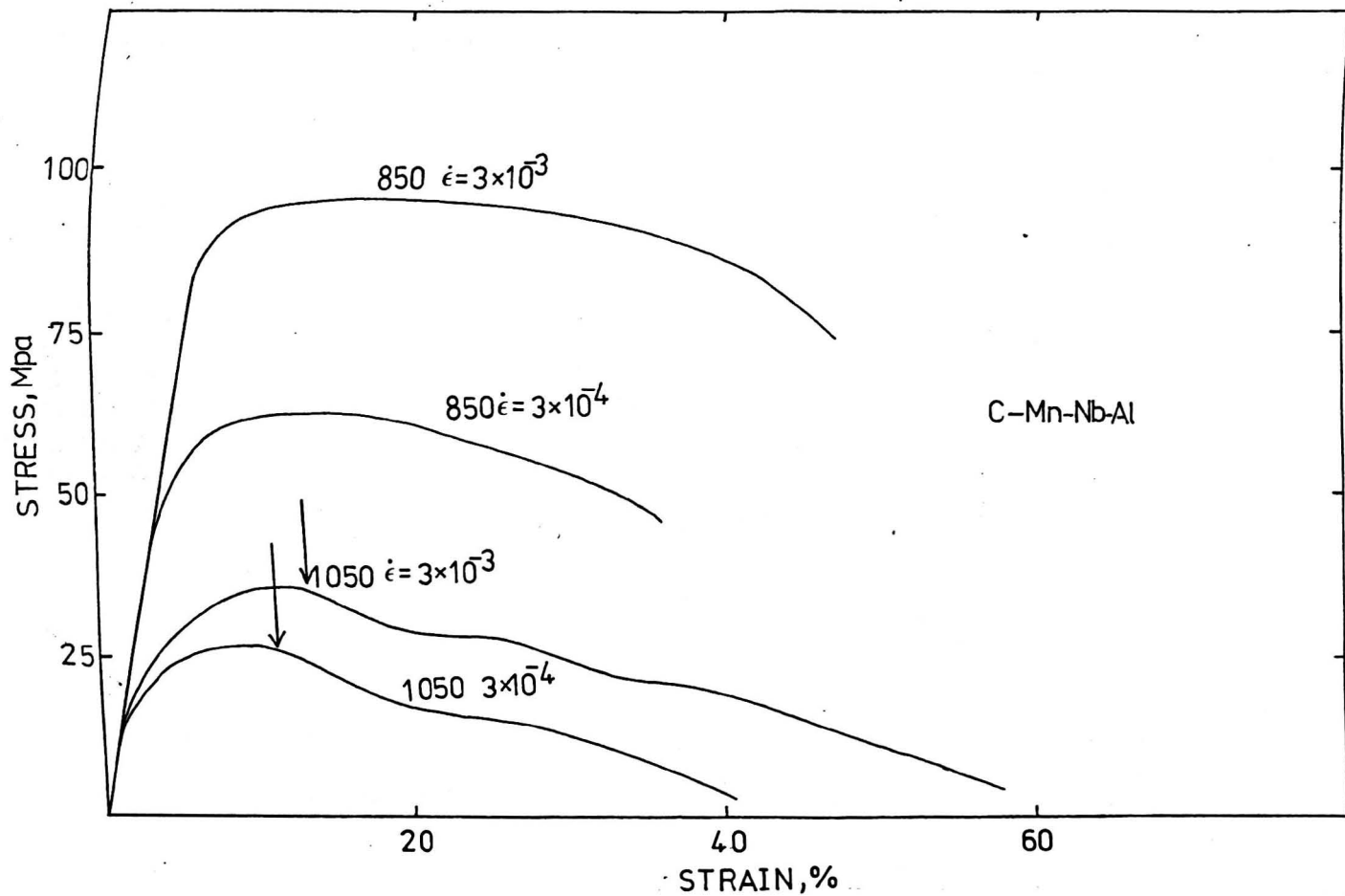
Fig. 10.11 Representative load-elongation curves at various temperatures and strain rates.
