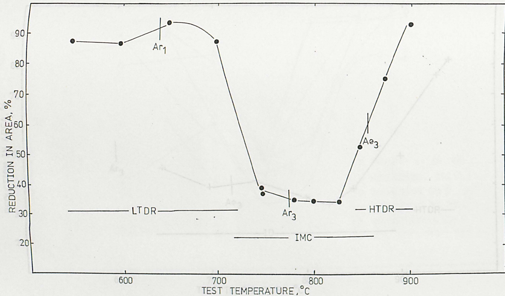
Fig. 4.20 Hot ductility, fracture and transformation data for the .05%C steel.
