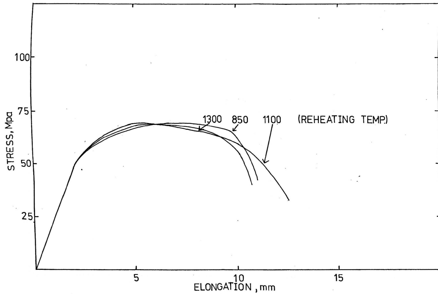
Fig. 6.5 Load-elongation curves for the C-Mn-V-Al steel
