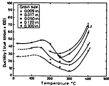
Fig. 2.10 Variation of ductility with temperature and grain size for Magnox A.180. (From Evans, 1969)
