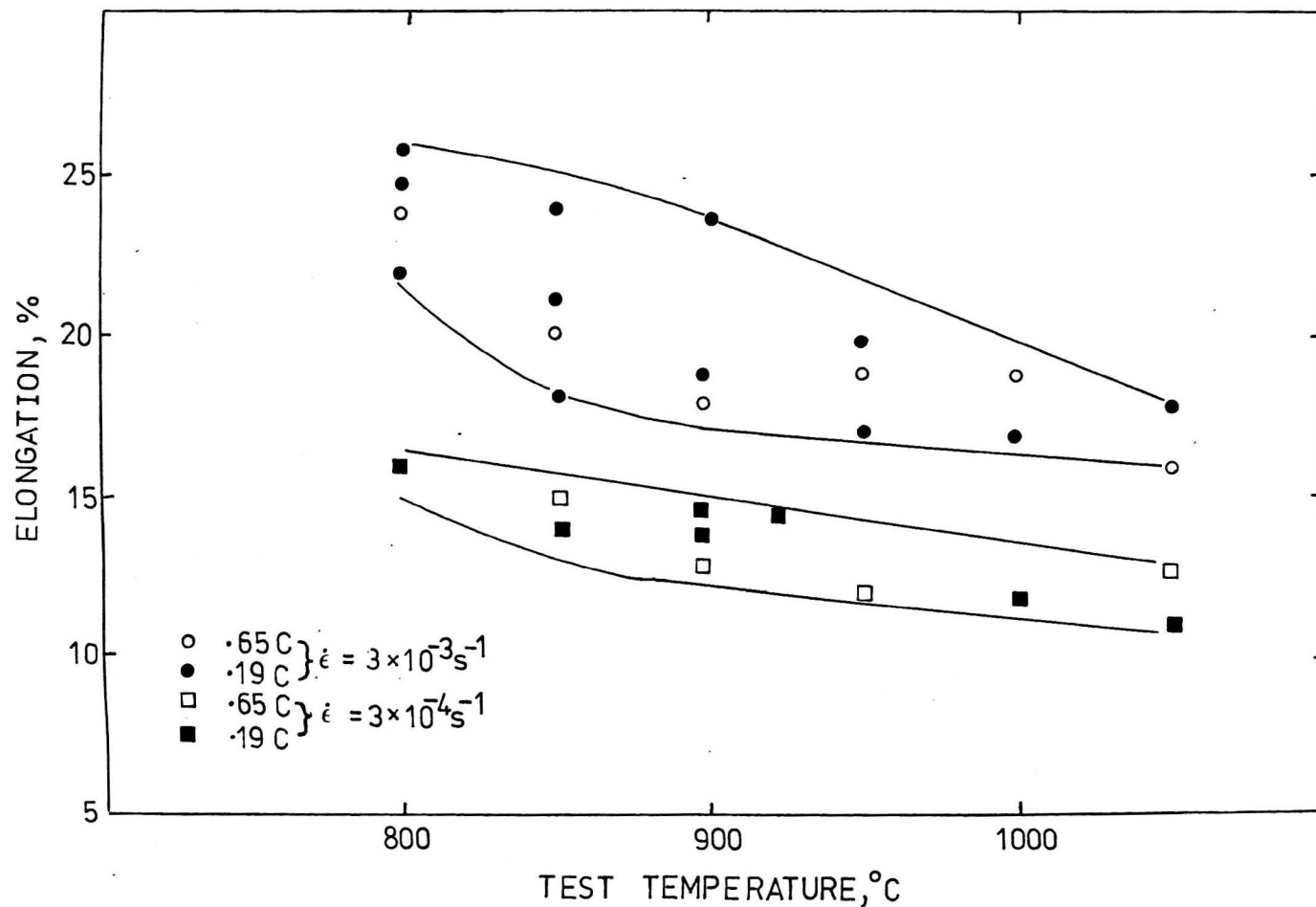
Fig. 4.30 Sample elongation at peak stress for the 0.19% C steel, and for the 0.65% C steel, at different temperature and strain rates.
