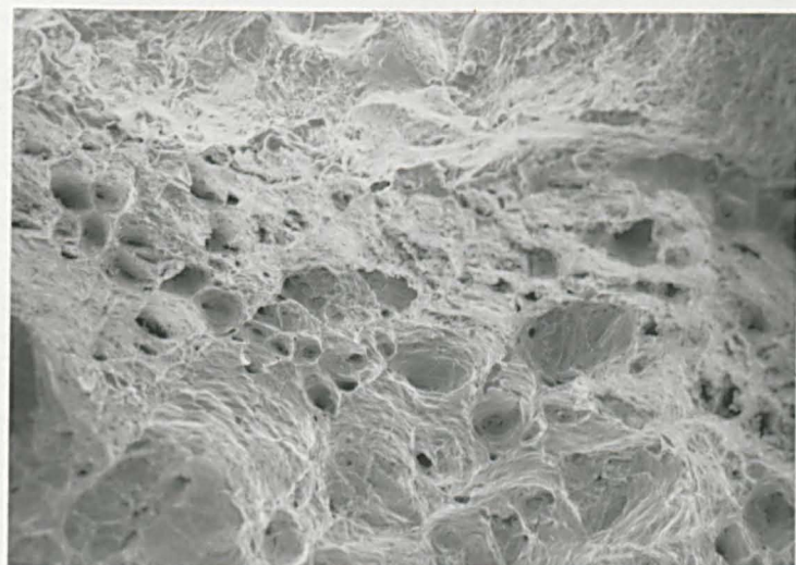
Fig.9.3 High temperature ductile rupture fracture mode, from 'as cast' samples fractured at 950°C.
