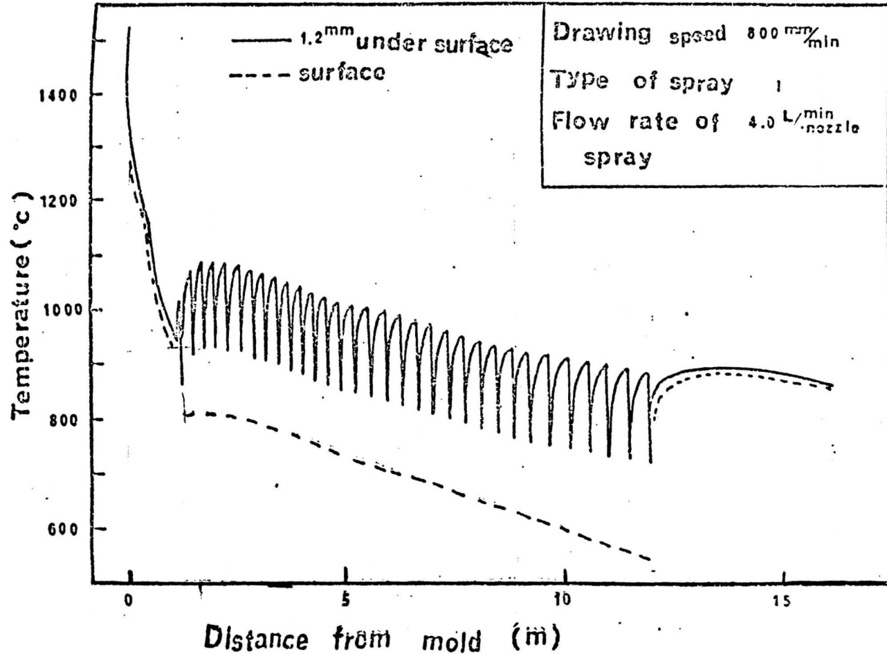
Fig. 2.5 Temperature oscillation in surface of continuously cast slab, from Tomono (1973)
