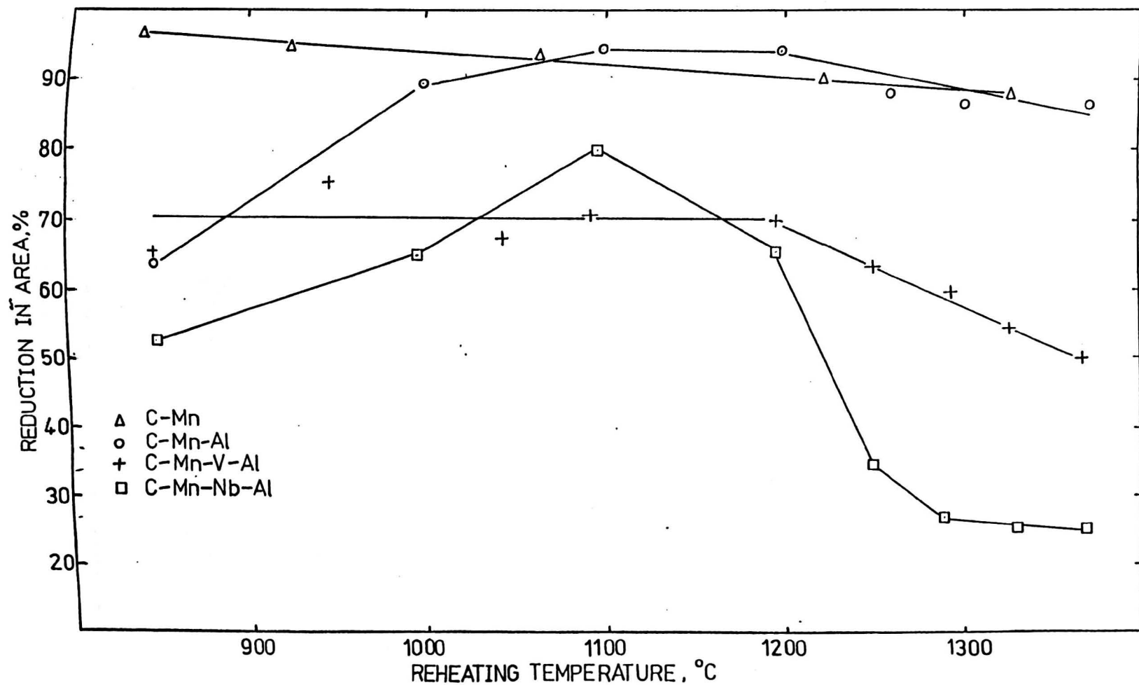
Fig. 6.2 Reduction of area values following tensile testing at 850°C after reheating to various temperatures, for C-Mn, C-Mn-Al, C-Mn-V-Al and C-Mn-Nb-Al steels.
