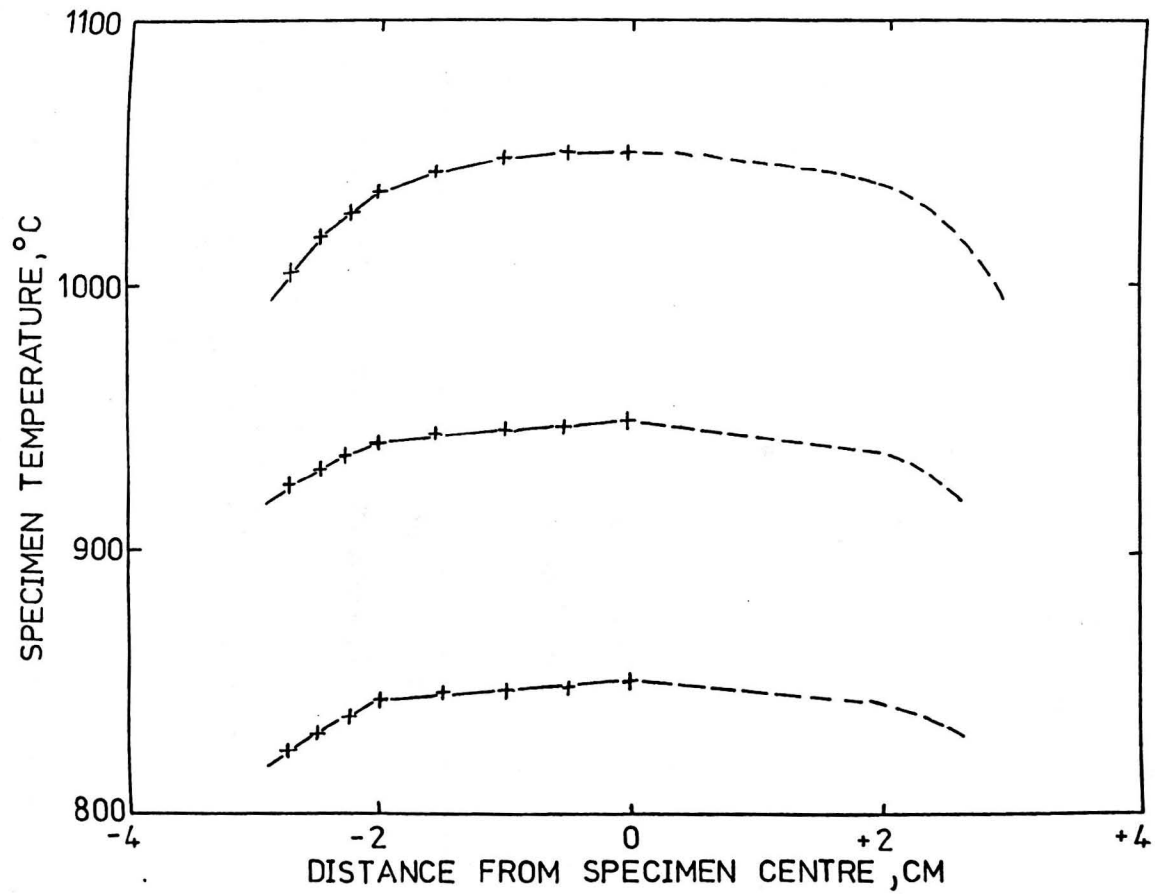
Fig. 3.7 Temperature distribution in Induction test piece at three different temperatures
