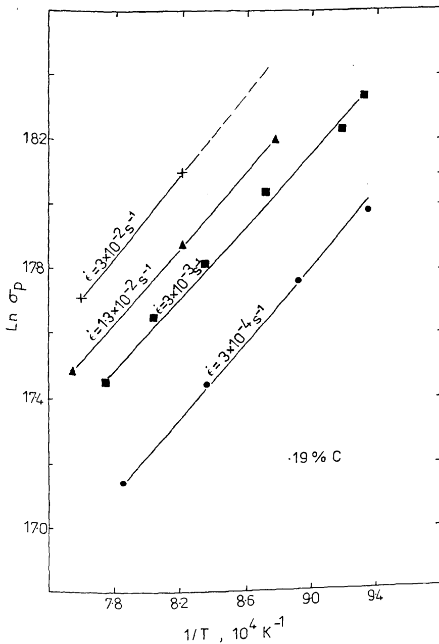
Fig. 4.23 Variation of peak stress, \sigma_p , with absolute temperature, T , at different strain rates for the 0.19% C steel
