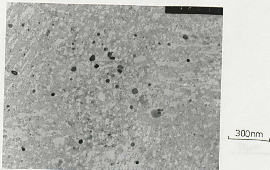
Fig. 6.10 NbCN precipitates extracted from fracture surface of C-Mn-Nb-Al steel after reheating to 1330°C
