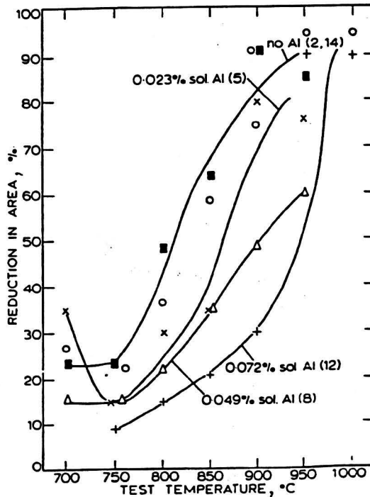
Fig. 2.15 Influence of Al on the hot ductility of C-Mn-Nb-Al steels. (After Mintz and Arrowsmith, 1979)
