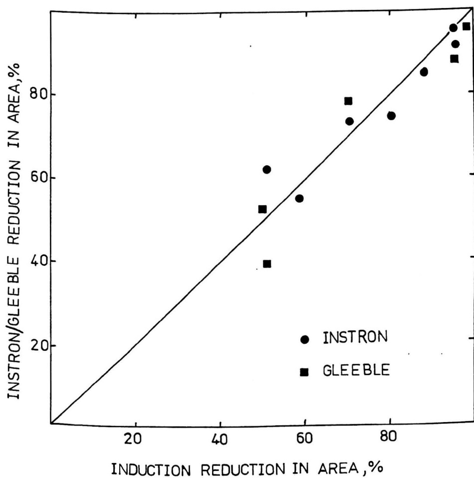
Fig. 3.8 Comparison of reduction in area values from different testing equipment, tests performed under identical conditions
