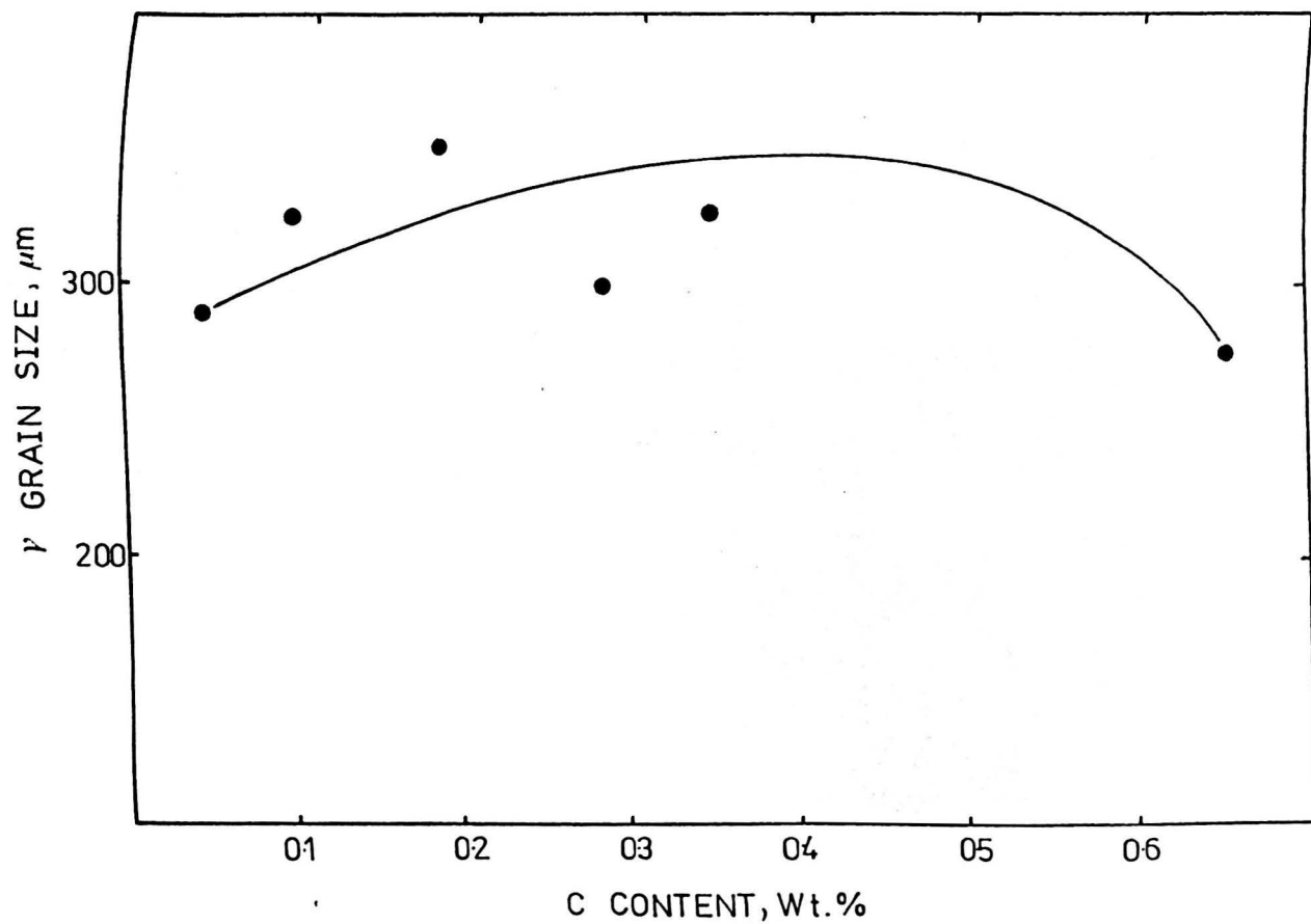
Fig. 4.5 Influence of C content on austenite grain size at 1330°C
