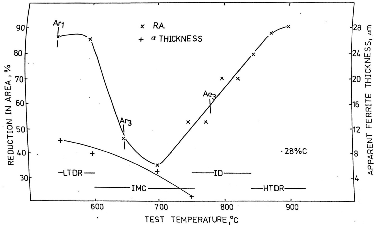
Fig. 4.9 Hot ductility, transformation and fracture data for the 0.28 C steel
