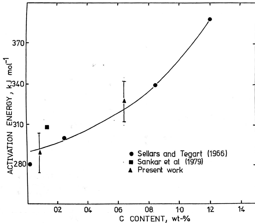
Fig. 4.29 Variation of activation energy for deformation with C content
