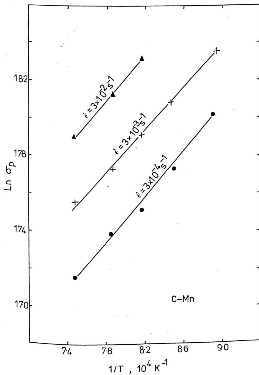
Fig. 10.2 Variation of peak stress with temperature and strain rate for the C-Mn steel.
