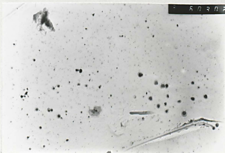
Fig.10.24 Precipitation in C-Mn-V-Al steel tested at 850°C using a strain rate of 3 \times 10^{-3} \text{ s}^{-1}
