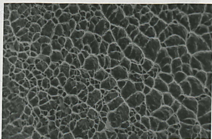
Fig.4.17 Intergranular micro void coalescence (IMC) fracture mode, showing void formation on grain facets. 0.10%C steel tested at 775°C.
