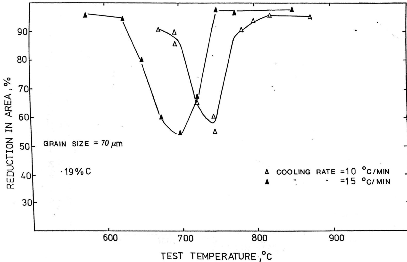
Fig. 5.7 Hot ductility curves for the .19% C steel following heating to 925 ^{\circ}\text{C} and cooling at either 10 ^{\circ}\text{C}/\text{min} or 15 ^{\circ}\text{C}/\text{min} . to test temperature.
