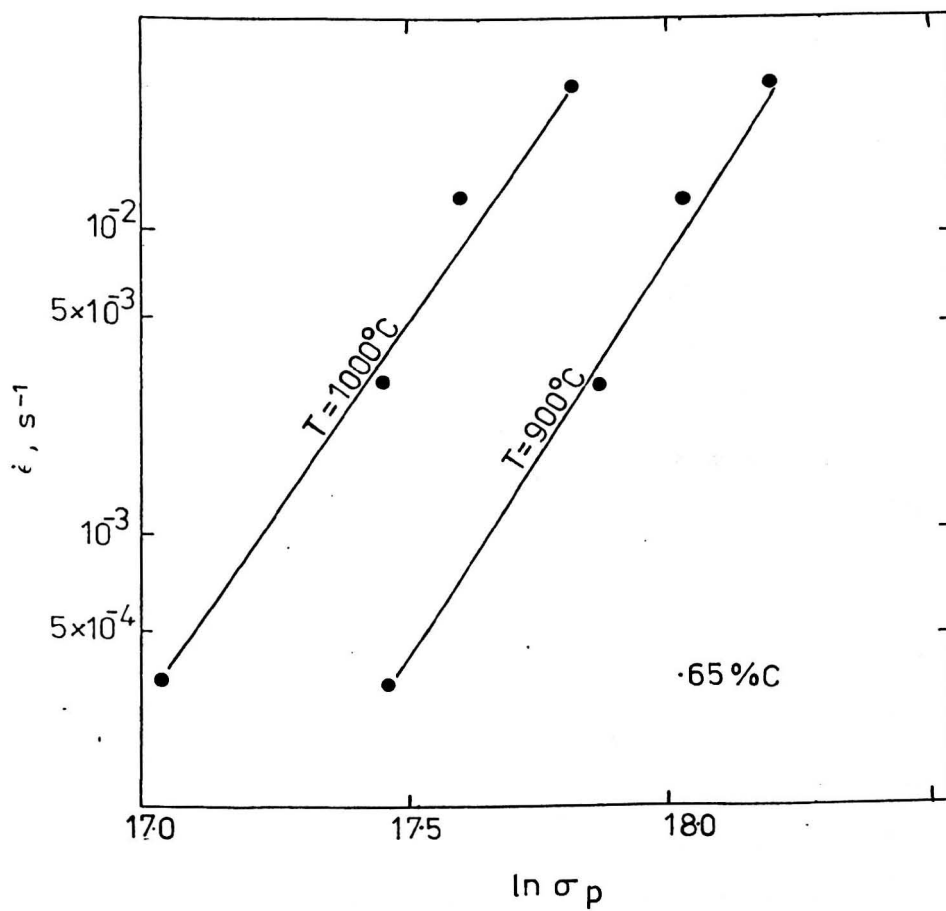
Fig. 4.28 Plot of \ln \dot{\epsilon} against \ln \sigma_p for the 0.65% C steel.
