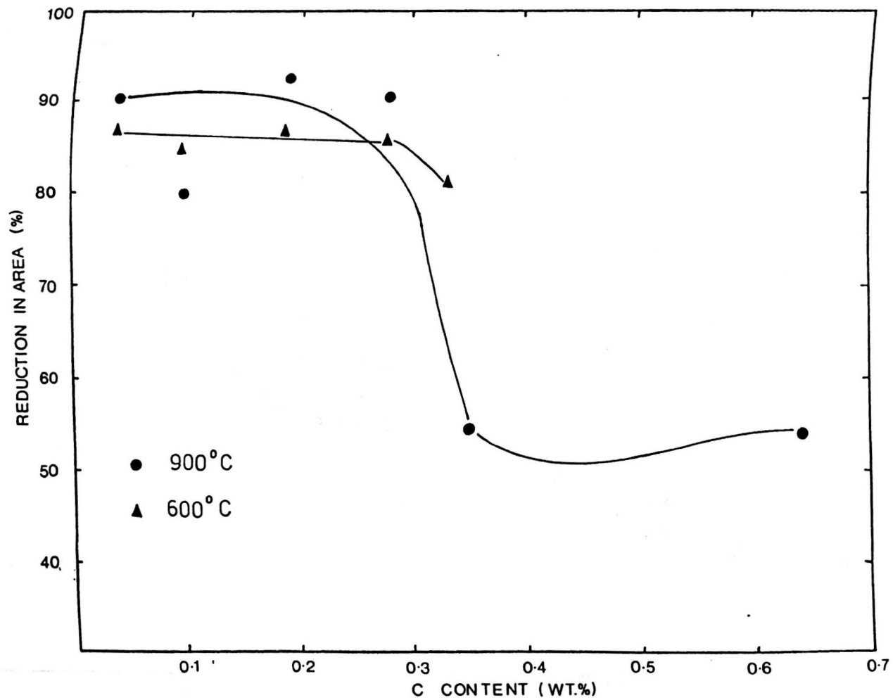
Fig. 4.2 Variation of reduction in area with C content at 900 and 600°C
