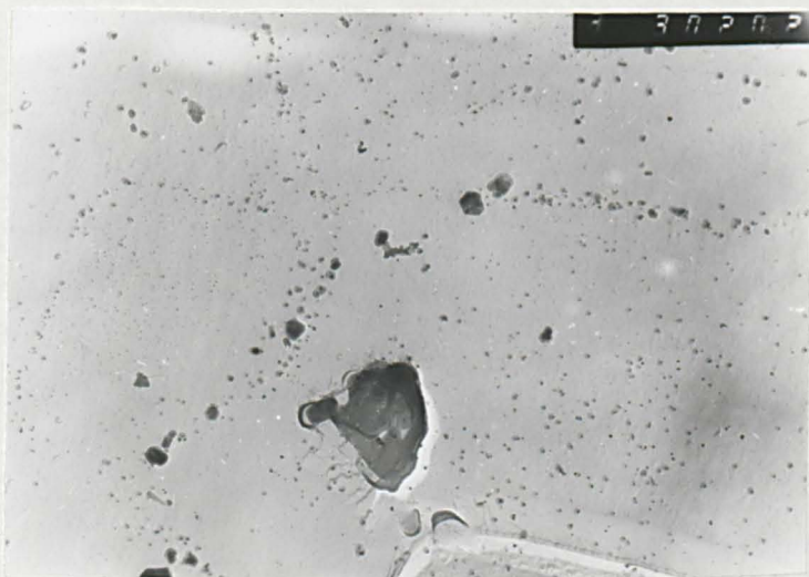
Fig. 6.15 Precipitation in C-Mn-Nb-Al steel heated to 850°C and tested, showing AlN and NbCN precipitation.
