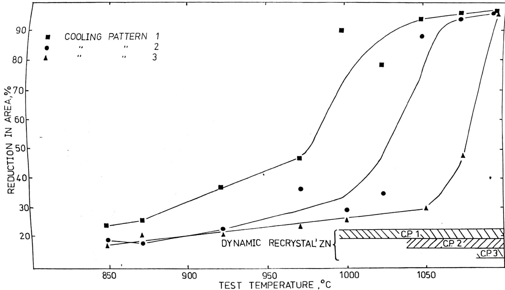
Fig. 8.3 Hot ductility curves for each cooling pattern, occurrence of dynamic recrystallization indicated by shaded regions.
