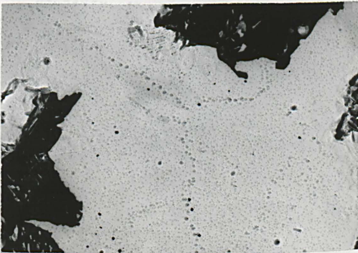
Fig.9.9 Precipitation in 'as cast' sample tested at 950°C.
