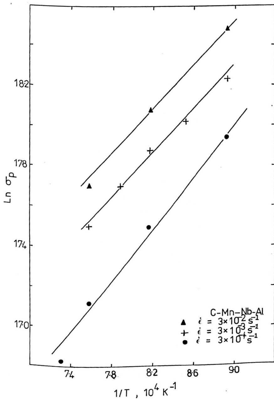
Fig. 10.4 Plot of \ln peak stress versus 1/T , where T is the absolute test temperature, for the C-Mn-Nb-Al steel for strain rates in the range 3 \times 10^{-2} - 3 \times 10^{-4} \text{ s}^{-1}
