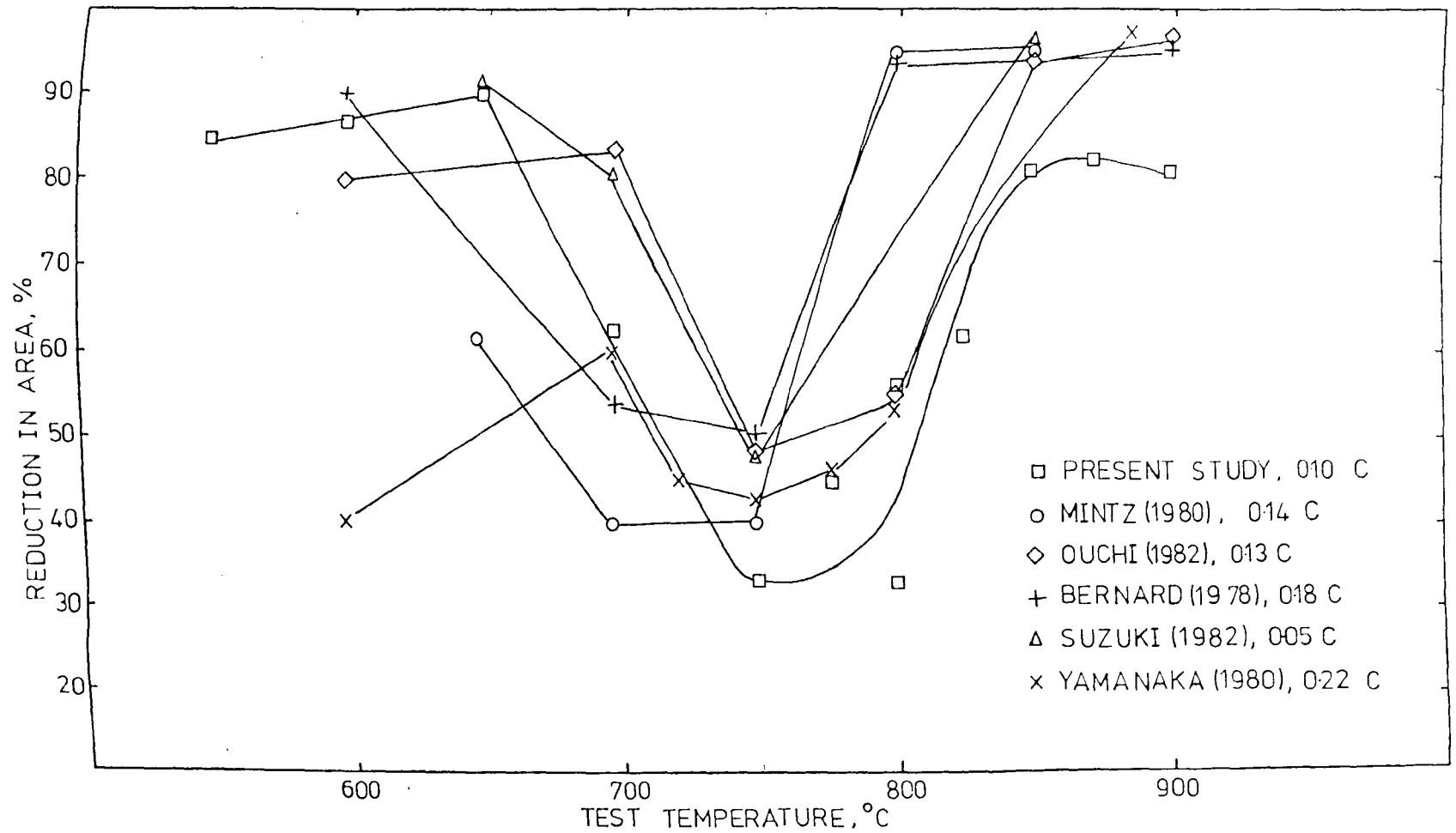
Fig. 4.22 Comparison of present hot ductility results with previous work
