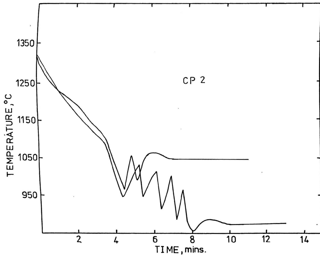
Fig. 8.2a Actual cooling curves for cooling pattern 2, test temperatures 870 and 1050°C
