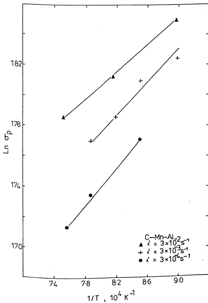
Fig. 10.3 Plot of \ln peak stress versus 1/T , where T is the absolute test temperature for the C-Mn-Al steel for strain rates in the range 10^{-2} - 10^{-4} \text{ s}^{-1}
