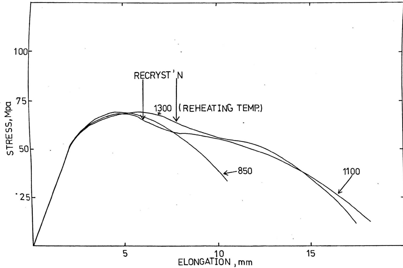
Fig. 6.4 Load-elongation curves for the C-Mn-Al steel
