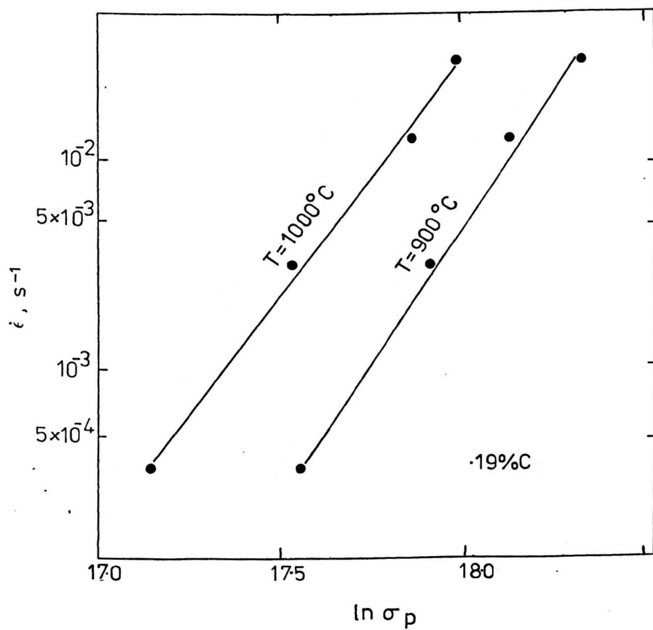
Fig. 4.27 Plot of \ln \dot{\epsilon} against \ln \sigma_p for the 0.19% C steel.
