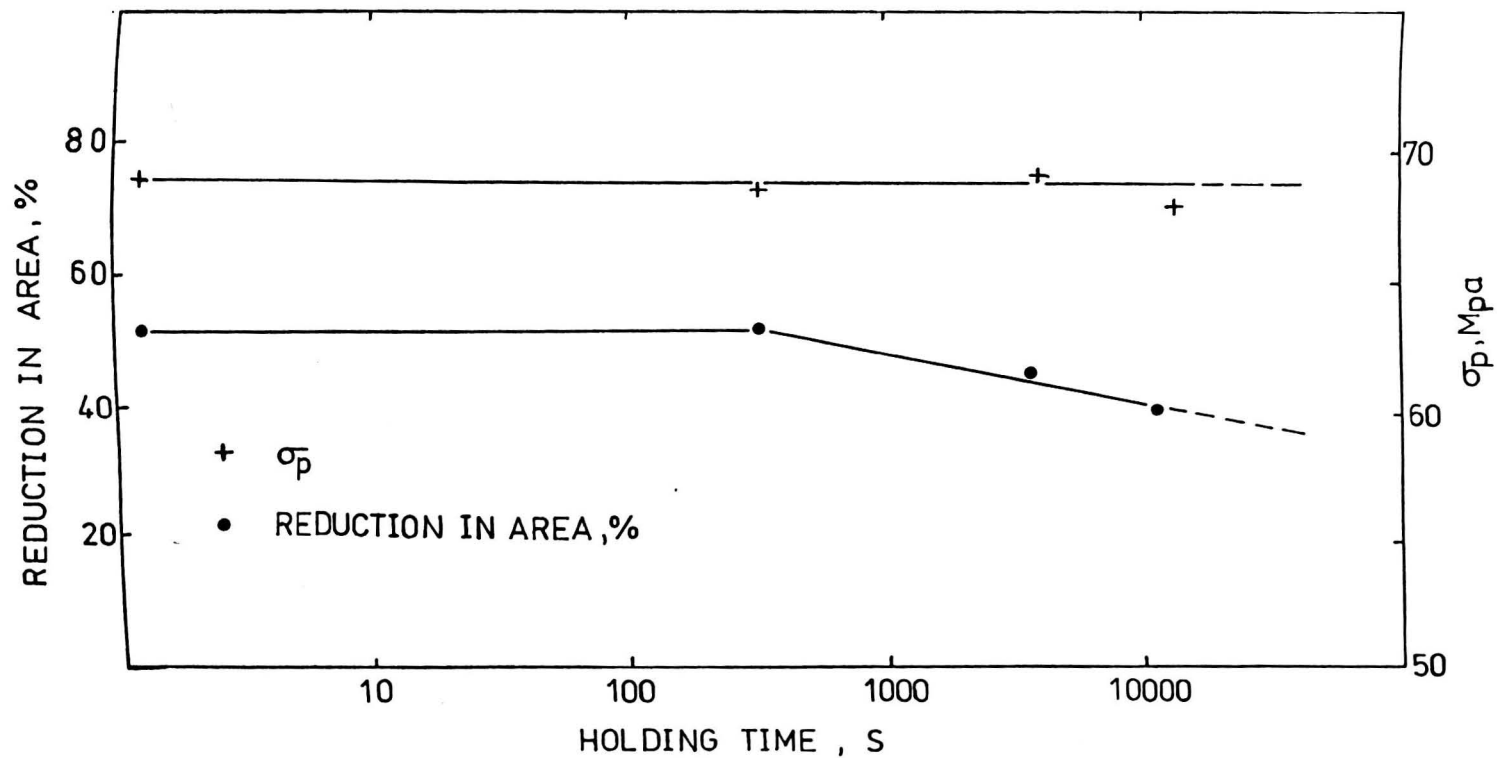
Fig. 7.3 Influence of holding time prior to testing on peak stress and hot ductility of the C-Mn-V-Al steel, tested at 50°C.
