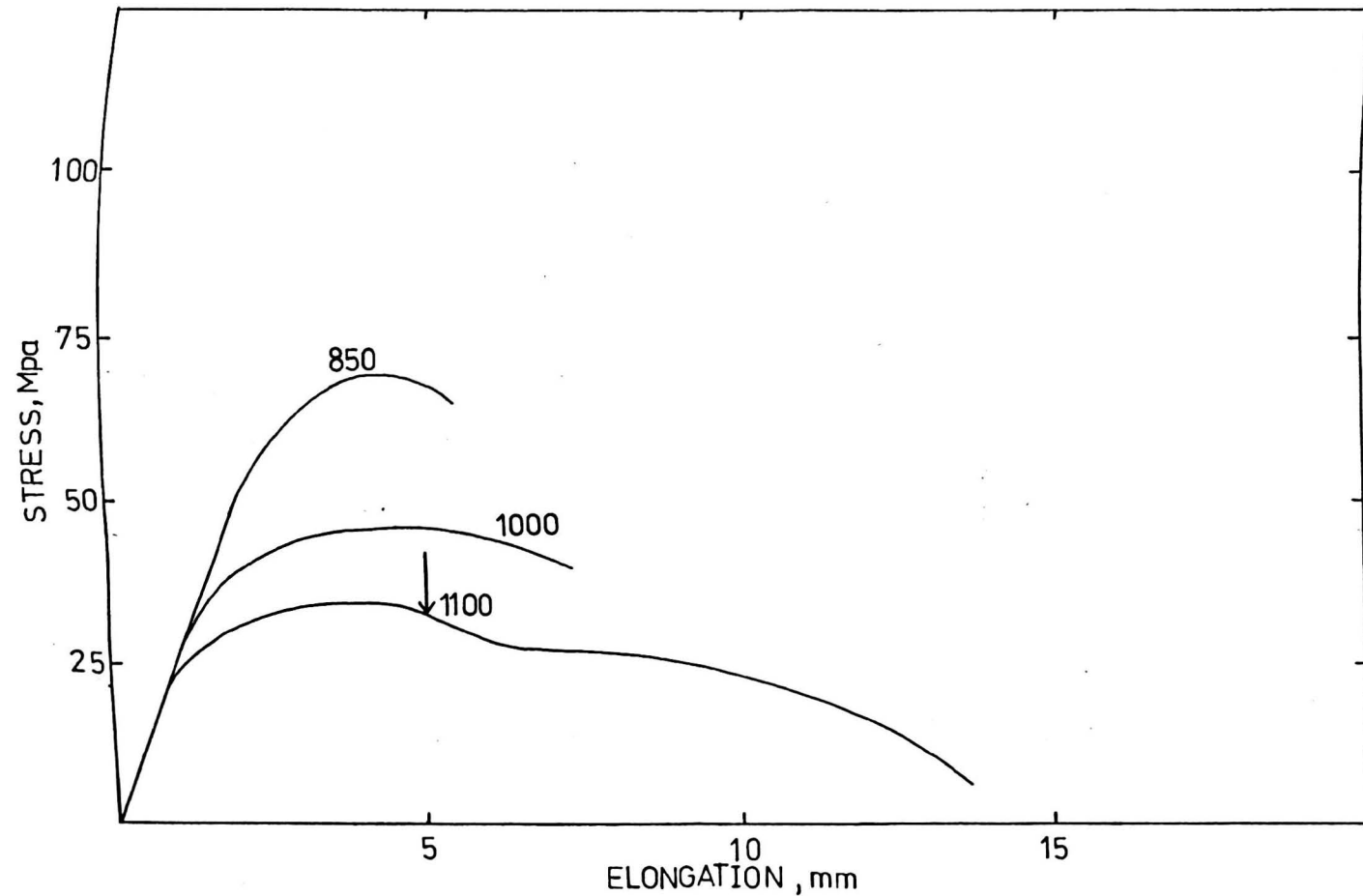
Fig.8.6 Representative load-elongation curves for cooling pattern 3.
