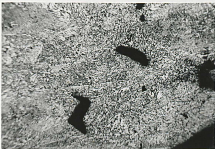
Fig. 4.13 Micrograph showing point of fracture of the 0.19%C steel tested at 650°C.
