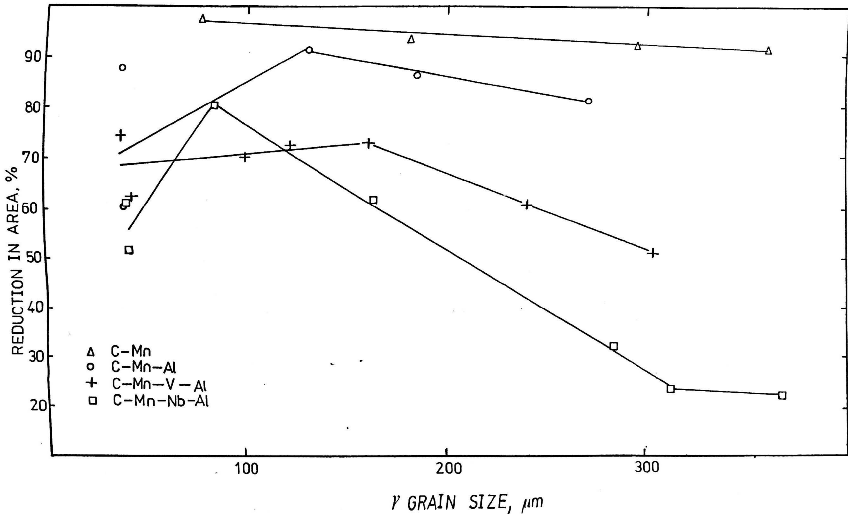
Fig. 6.3 Variation of reduction in area values with austenite grain size.
