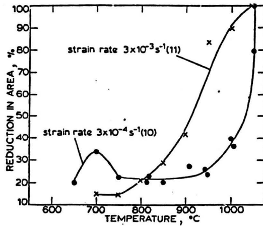
Fig. 2.8 Influence of strain rate on the hot ductility of a C-Mn-Nb-Al steel. (After Mintz and Arrowsmith 1979)
