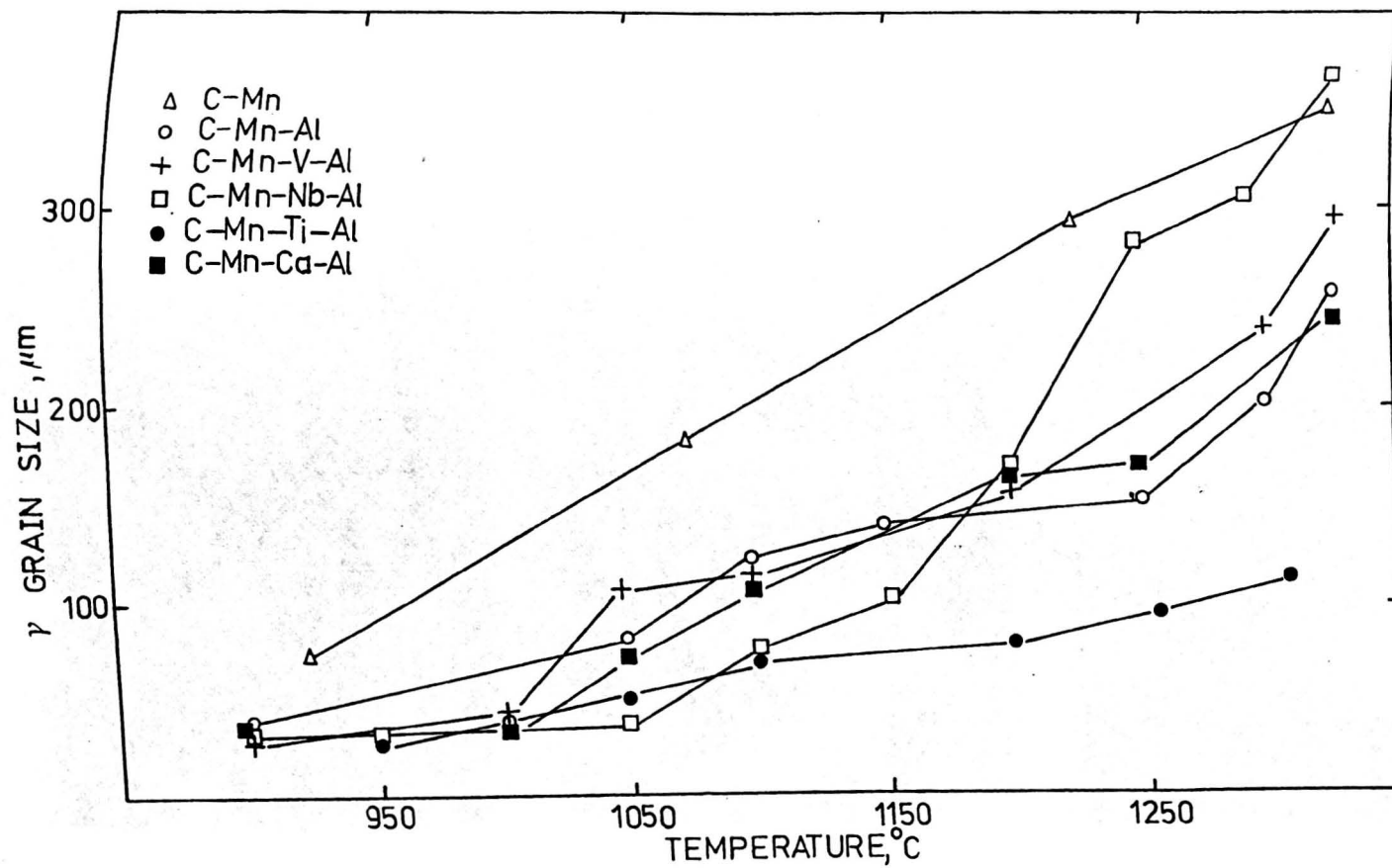
Fig. 10.16 Variation of austenite grain size with temperature.
