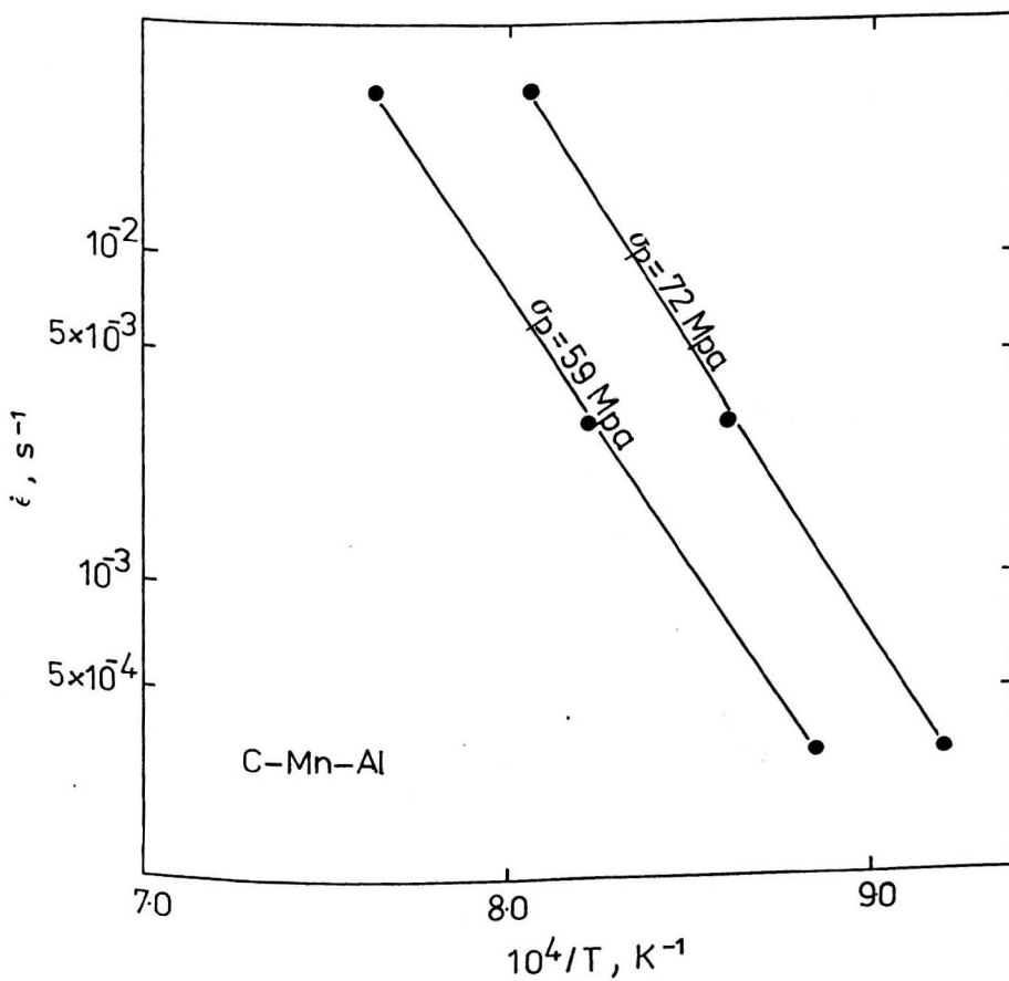
FIG. 10.6 Plot of \ln \dot{\epsilon} against 1/T at constant \sigma_p for the C-Mn-Al steel.
