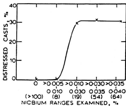
Fig. 2.13 Influence of Nb on the transverse cracking of continuously cast slabs. (From Mintz and Arrowsmith, 1979)
