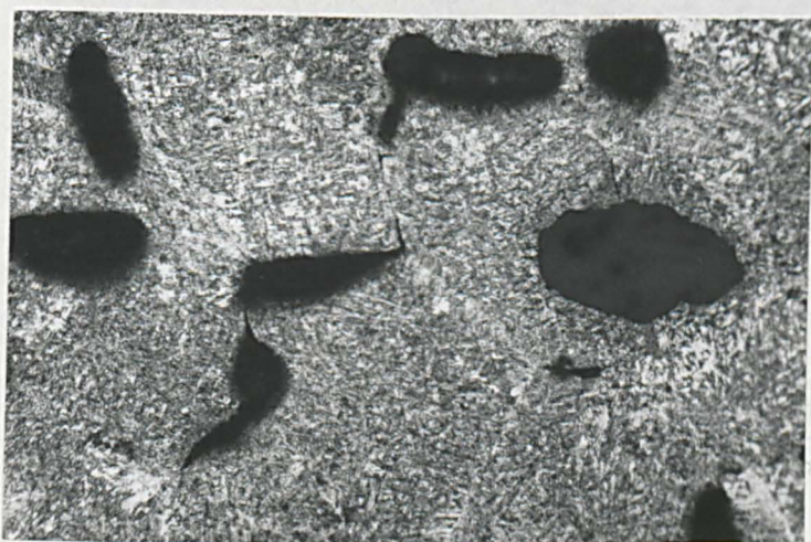
Fig. 4.15 Crack formation in the 0.35%C steel tested at 850°C.
