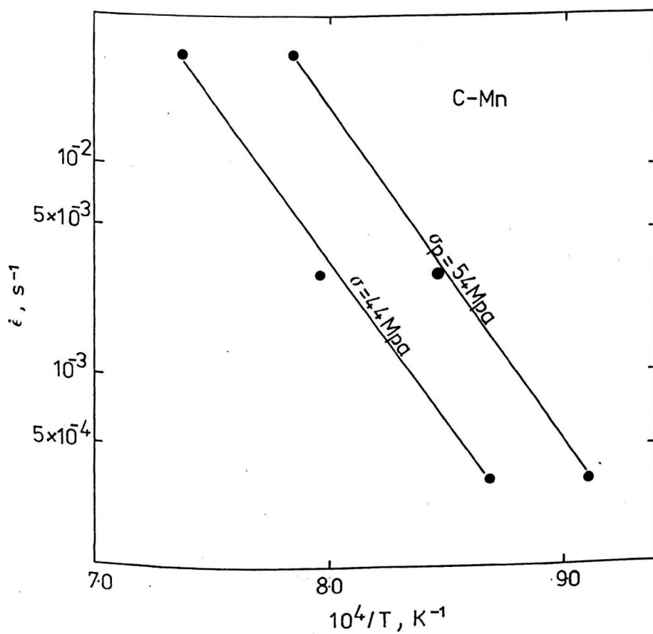
Fig. 10.5 Plot of \ln \dot{\epsilon} against 1/T at constant \sigma_p for the C-Mn steel.
