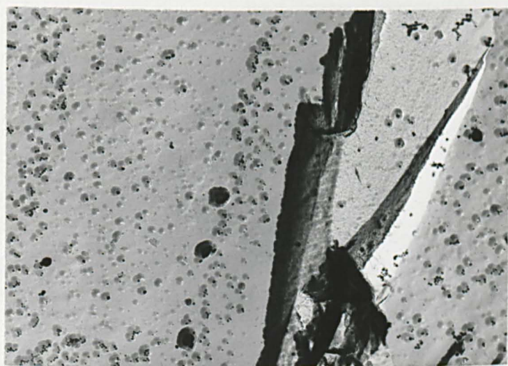
Fig.9.11 Precipitation in 'reheated Gleeble' sample tested at 950°C.
