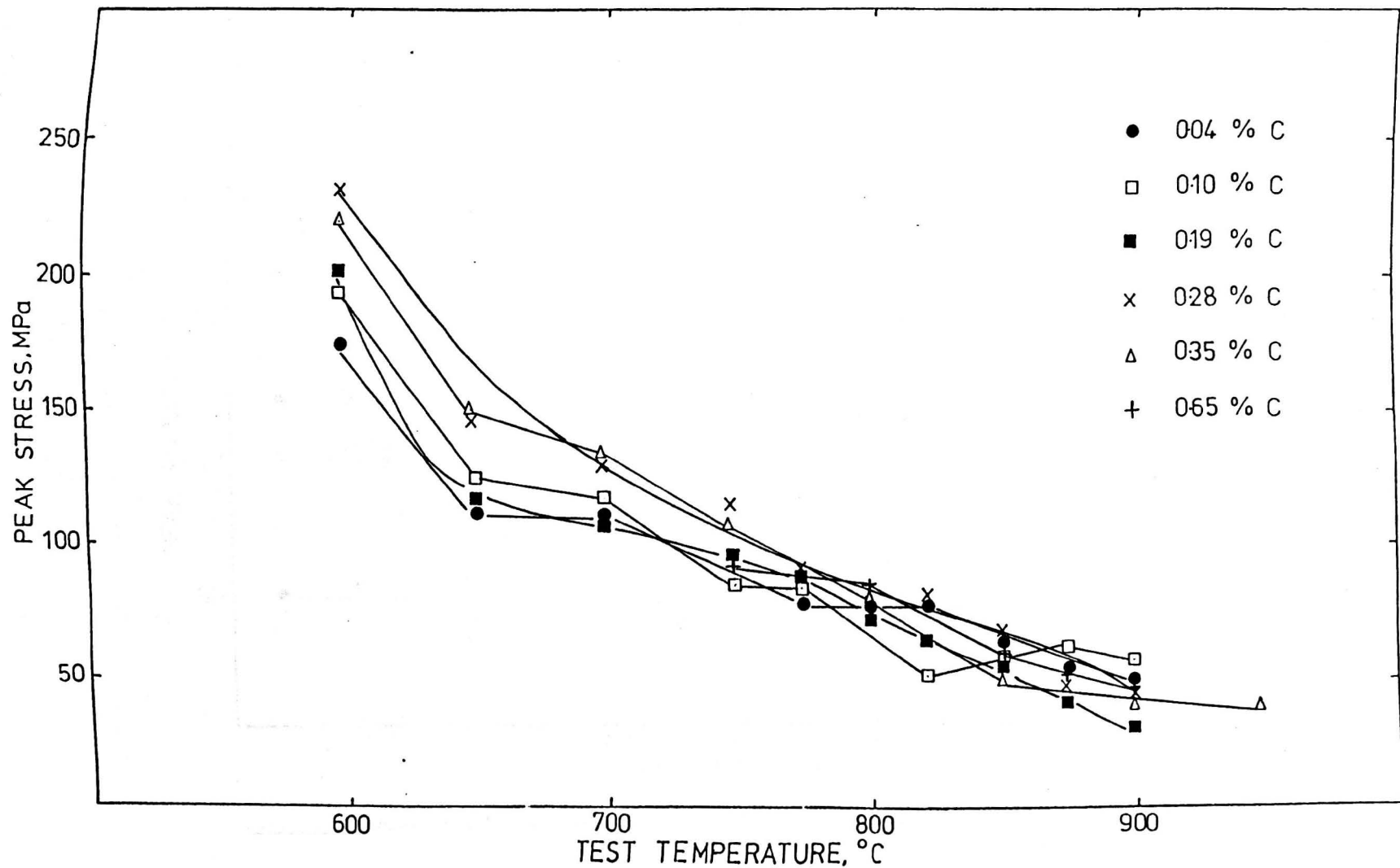
Fig. 4.3 Variation of peak stress with test temperatures for steels 1 - 6.
