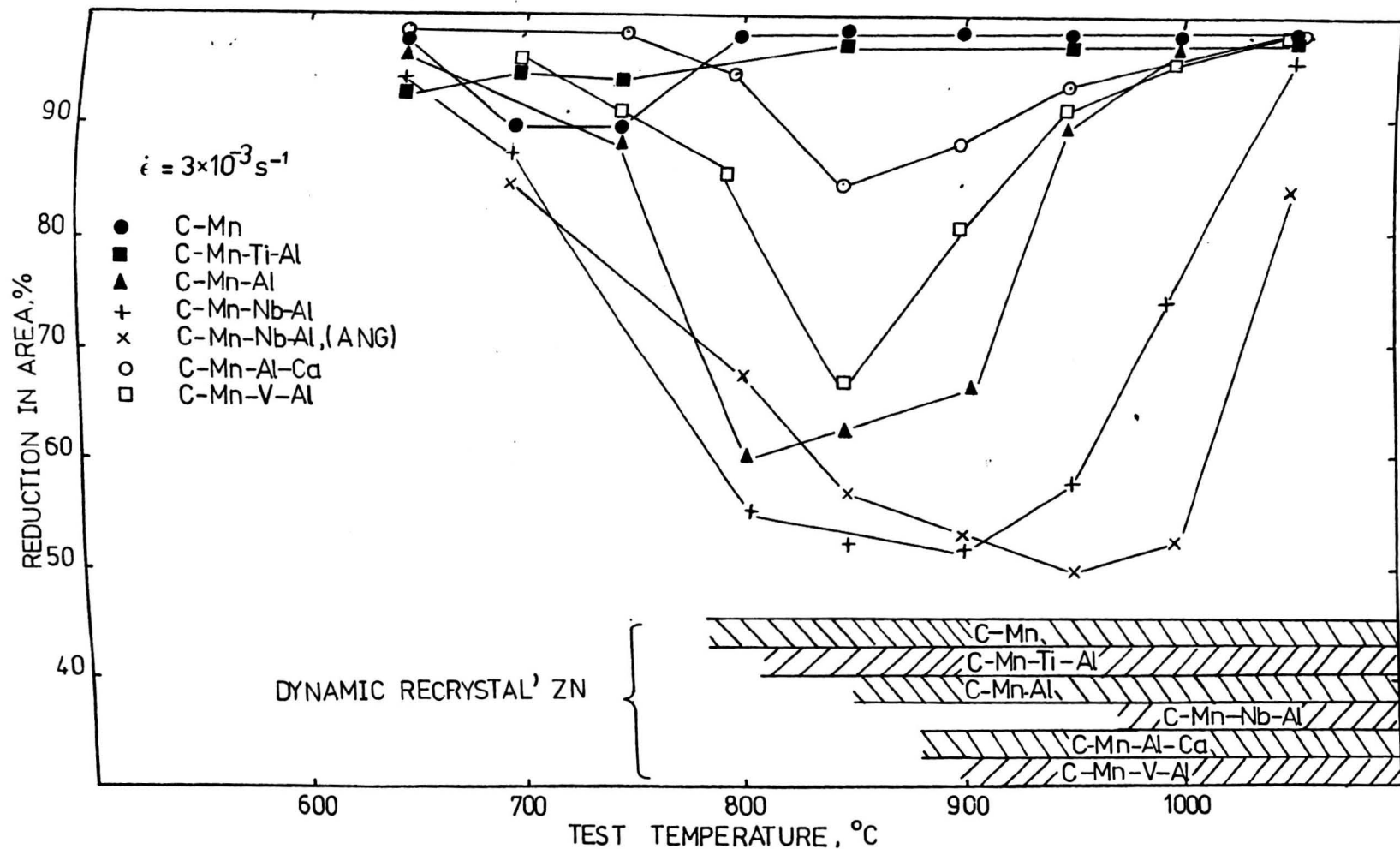
Fig. 10.12 Hot ductility curves for all six steels at \dot{\epsilon} = 3 \times 10^{-3} \text{ s}^{-1} , occurrence of dynamic recrystallization indicated by shaded regions.
