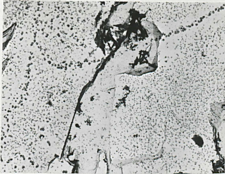
Fig.9.8 Precipitation in 'reheated' sample tested at 950°C. N.B. precipitate free zones.
