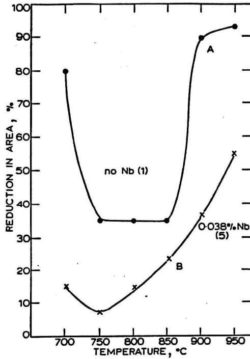
Fig. 2.14 Influence of Nb on the hot ductility of C-Mn-Nb-Al Steels. (After Mintz and Arrowsmith, 1979)
