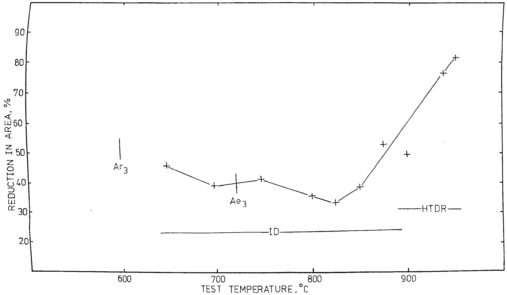
Fig. 4.21 Hot ductility, fracture and transformation data for the .65%C steel
