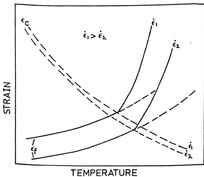
Fig. 11.2 Schematic illustration of variation of \epsilon_c and \epsilon_f with temperature and strain rate.
