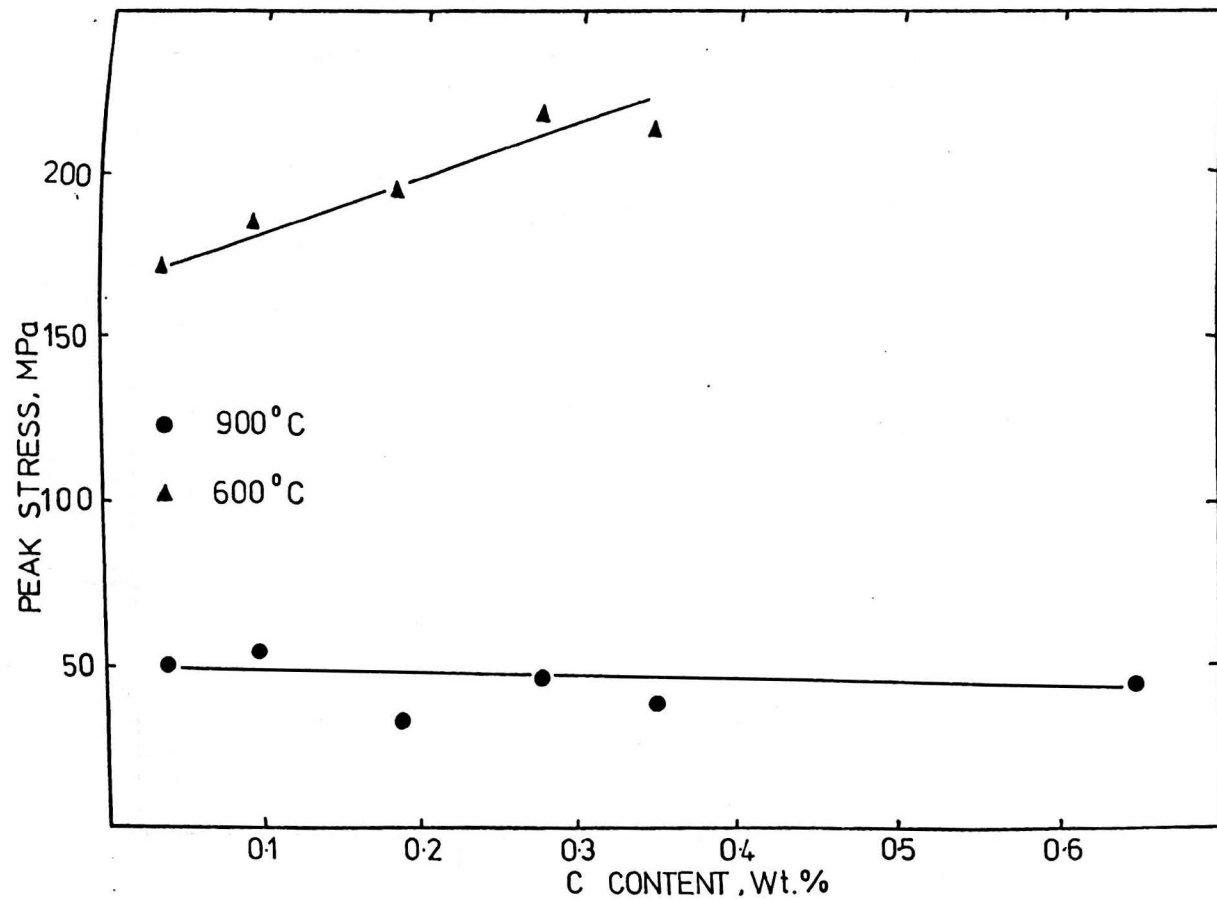
Fig. 4.4 Variation in peak stress with C content at 900 and 600°C
