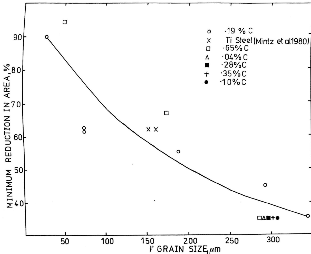
Fig. 5.8 Variation of minimum reduction in area values with austenite grain size following testing in the range 700 - 1000°C.
