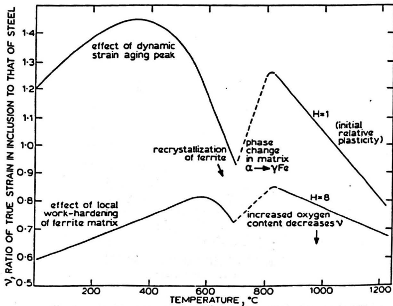
Fig. 2.9 Variation of relative plasticity of sulphide inclusions with deformation temperature and oxygen content. (After Charles, 1980)
