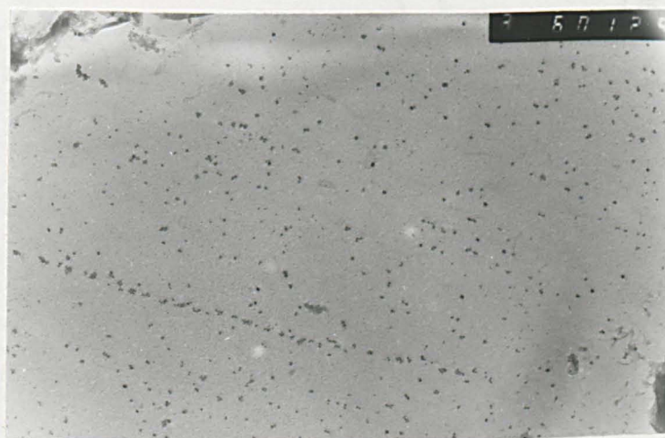
Fig.6.17 Precipitation in C-Mn-Nb-Al steel heated to 1330°C prior to testing at 850°C.
