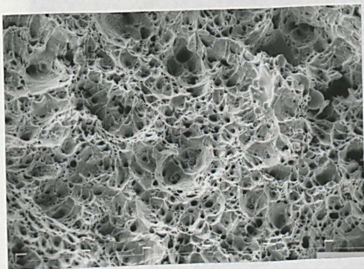
Fig. 4.16 Low temperature ductile rupture (LTDR) fracture mode, showing void formation at second phase particles. 0.04%C steel, tested at 550°C.
