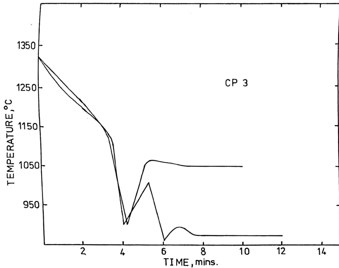
Fig. 8.2b Actual cooling curves for cooling pattern 3, test temperatures 870 and 1050°C.
