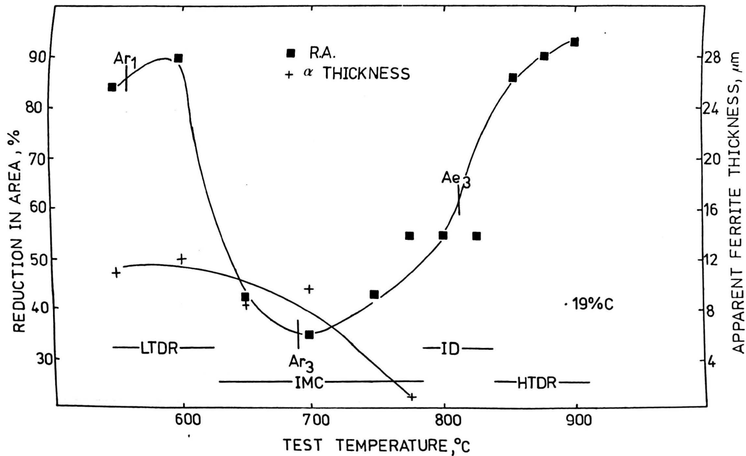
Fig. 4.8 Hot ductility, transformation and fracture data for the 0.19%C steel
