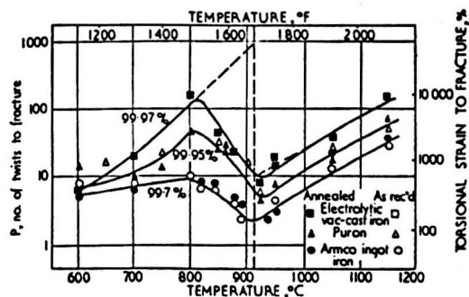
Fig. 2.12 Hot ductility of irons tested in hot torsion. (From Robbins et al, 1961)
