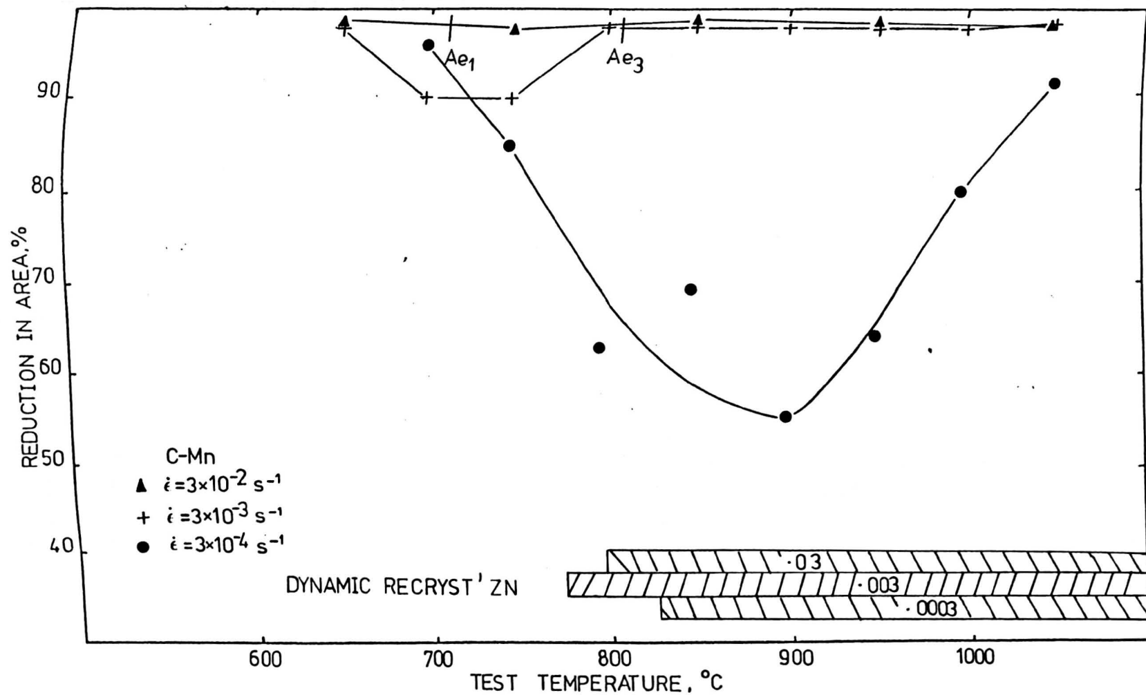
Fig. 10.13 Influence of strain rate on the hot ductility of C-Mn steel, occurrence of dynamic recrystallization indicated by shaded regions.
