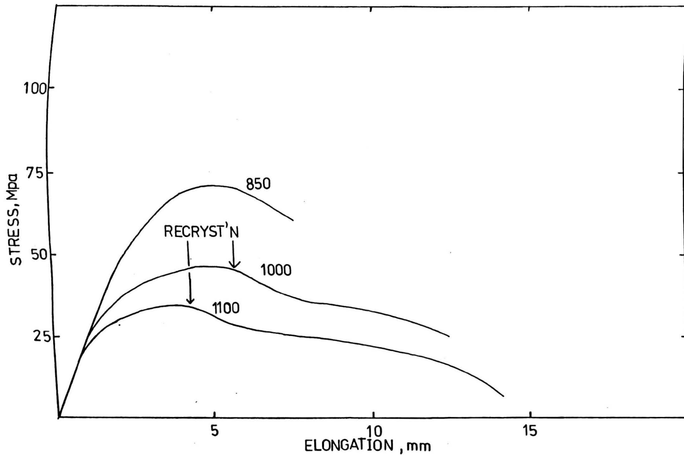
Fig. 8.4 Representative load-elongation curves for cooling pattern 1.
