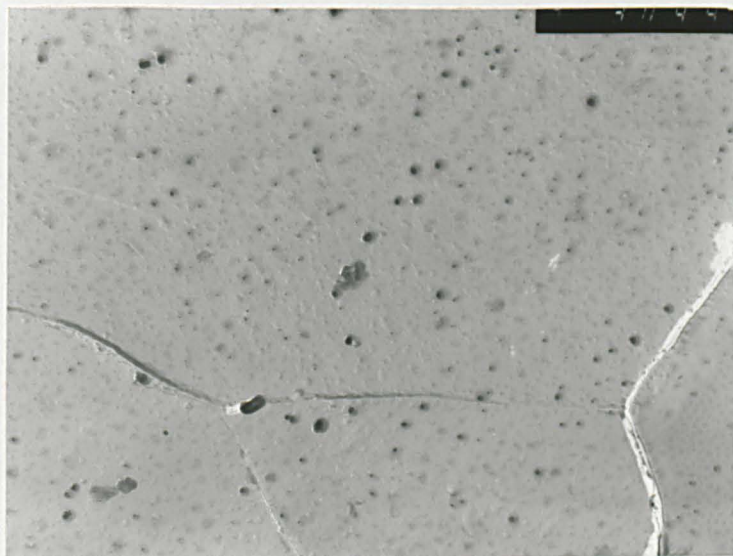
Fig. 6.16 Precipitation in C-Mn-Nb-Al steel heated to 1100°C prior to testing at 850°C
