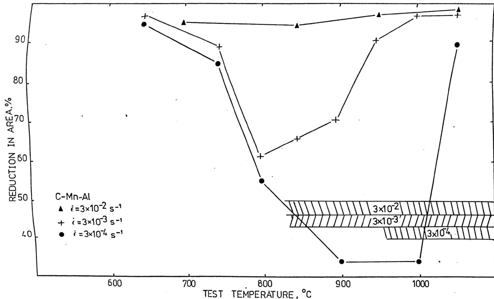
Fig. 10.14 Influence of strain rate on the hot ductility of C-Mn-Al steel, occurrence of dynamic recrystallization indicated by shaded regions.
