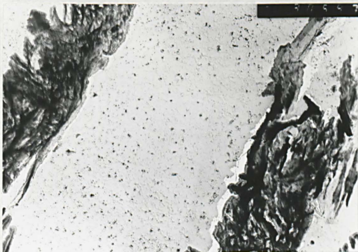
Fig. 6.14 Precipitation in C-Mn-V-Al steel after reheating to 1050°C and testing at 850°C.
