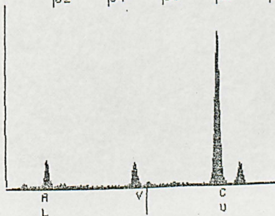
Fig.6.13 Precipitation in C-Mn-V-Al steel heated to 850°C and tested, showing VCN and AlN precipitation and associated X-ray spectra.
