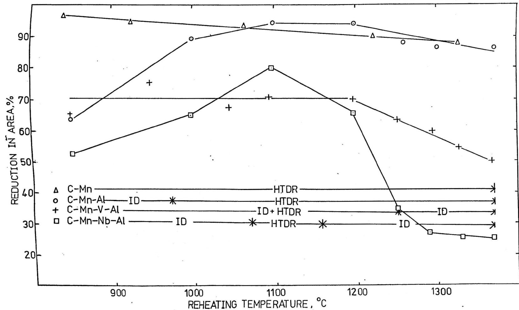
Fig. 6.7 Extent of fracture mode for each steel.
