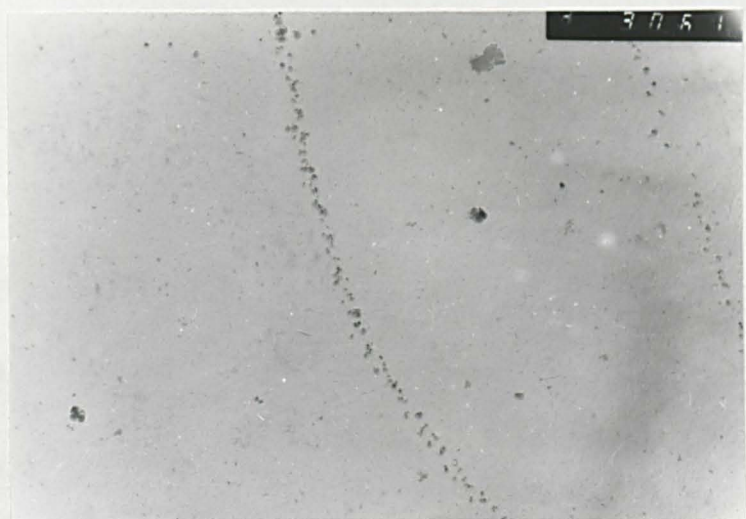
Fig.10.20 AlN precipitation in C-Mn-Al-Ca steel tested at 850°C using a strain rate of 3 \times 10^{-3} \text{ s}^{-1} .
