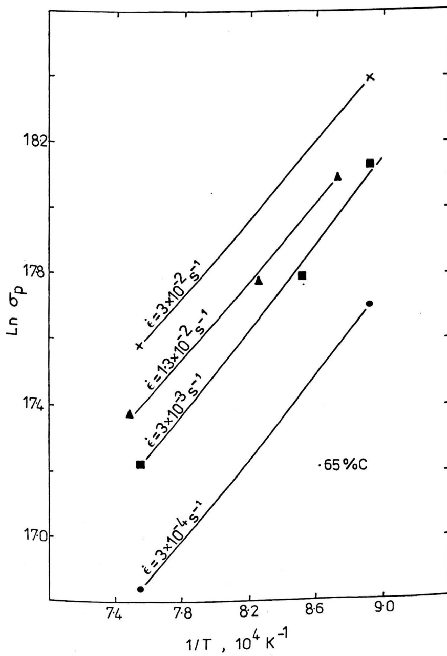
Fig. 4.24 Variation of peak stress, \sigma_p , with absolute temperature, T , at different strain rates for the 0.65% C steel
