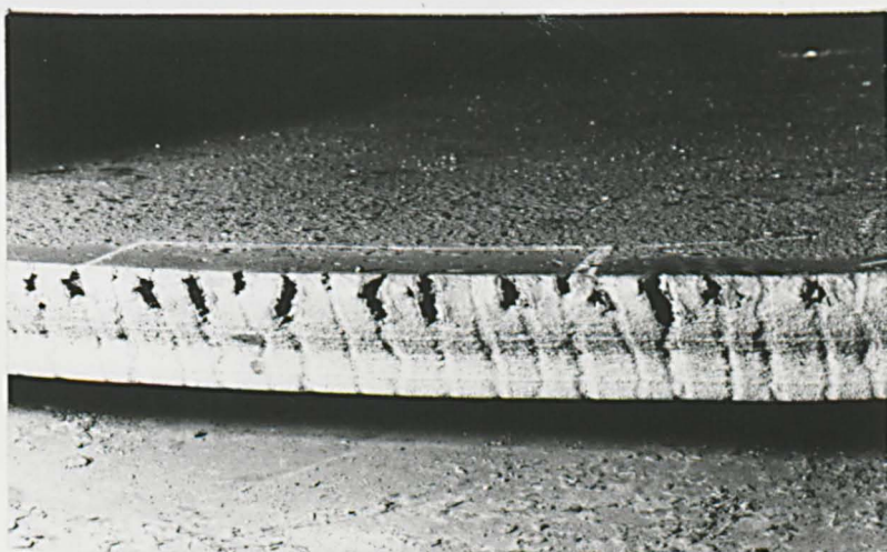
Fig.2.2 Slab which had been partially rolled showing severe transverse edge cracking.
