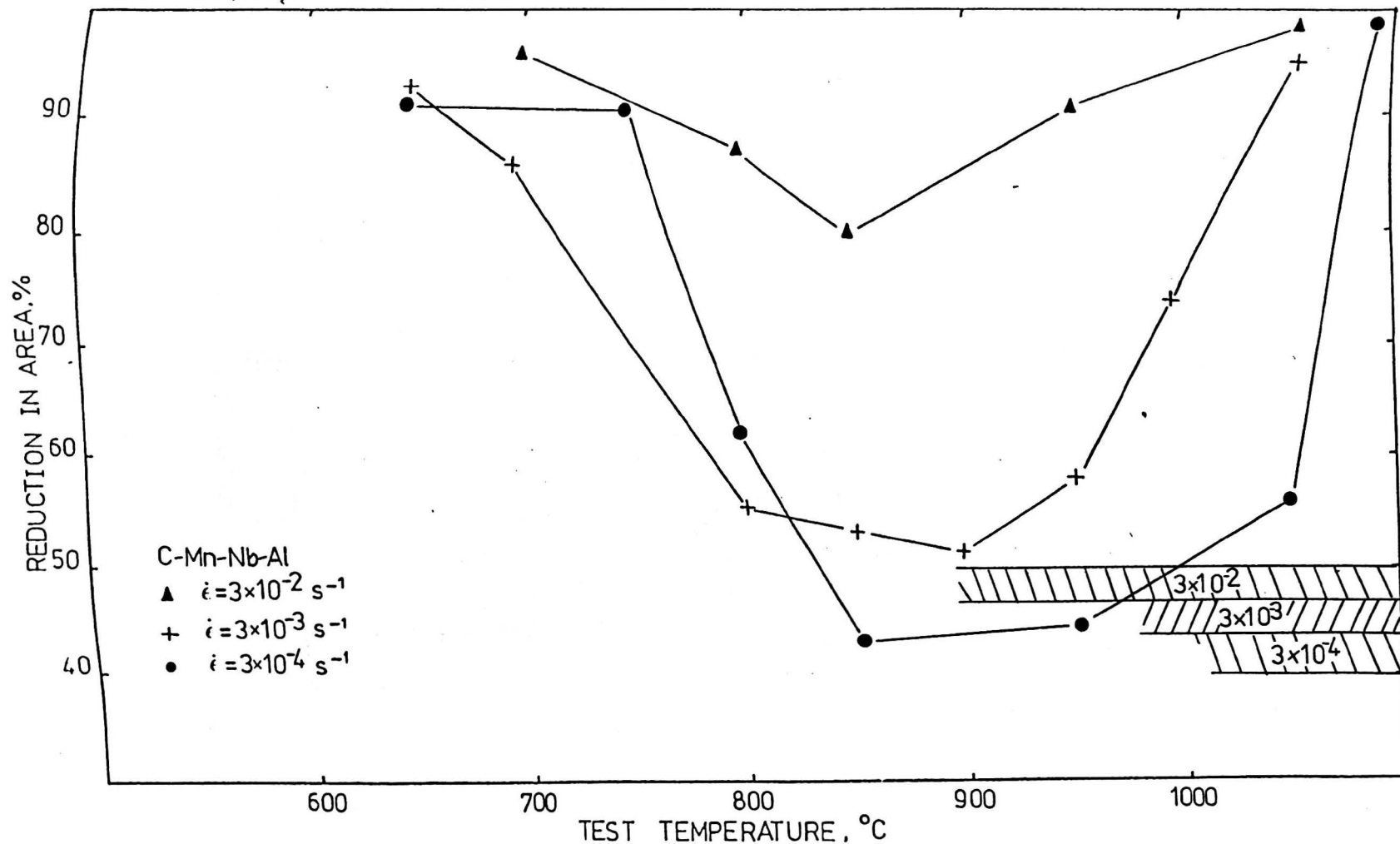
Fig. 10.15 Influence of strain rate on the hot ductility of C-Mn-Nb-Al steel, occurrence of dynamic recrystallization indicated by shaded regions.
