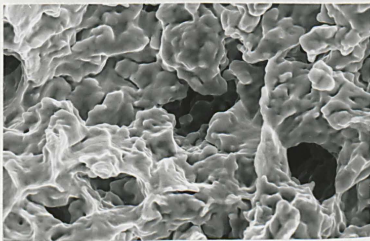
FIG.10.17 Fracture surface of C-Mn-Nb-Al fractured at 850°C using a strain rate of 3 \times 10^{-3} \text{ s}^{-1}
