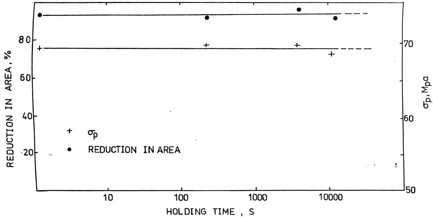
Fig. 7.2 Influence of holding time prior to testing on peak stress and hot ductility of the C-Mn-Al steel tested 850°C.
