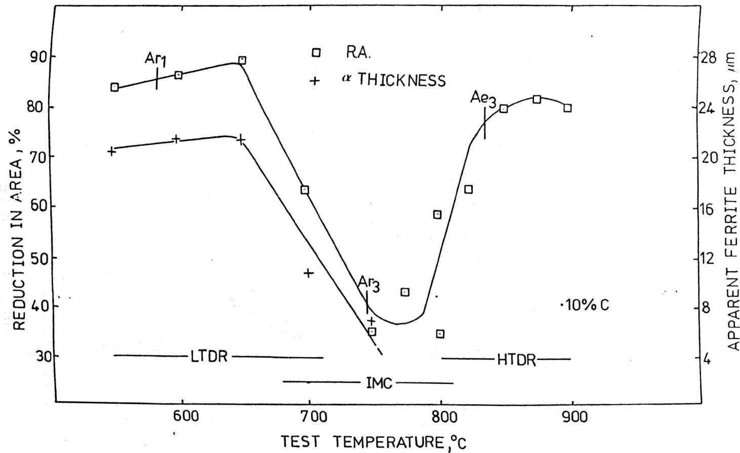
Fig. 4.7 Hot ductility, transformation and fracture data for the 0.10% C steel
