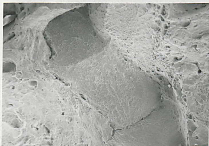
Fig.9.4 Intergranular microvoid coalescence fracture mode, from 'as cast' sample fractured at 950°C.
