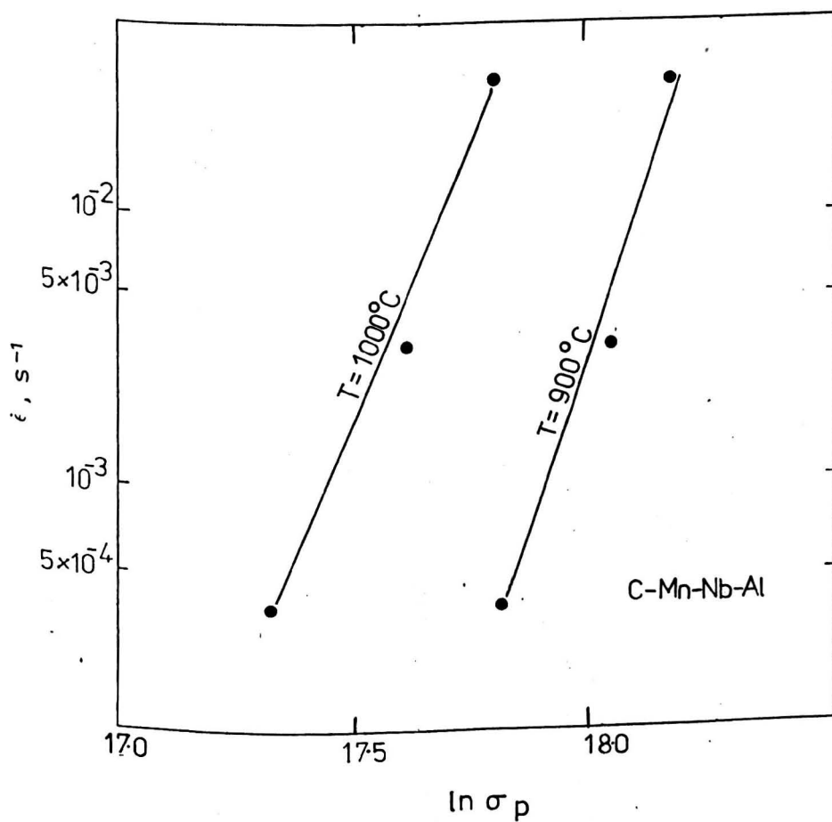
Fig. 10.10 Plot of \ln \dot{\epsilon} against \ln \sigma_p at constant temperatures for the C-Mn-Nb-Al steel.
