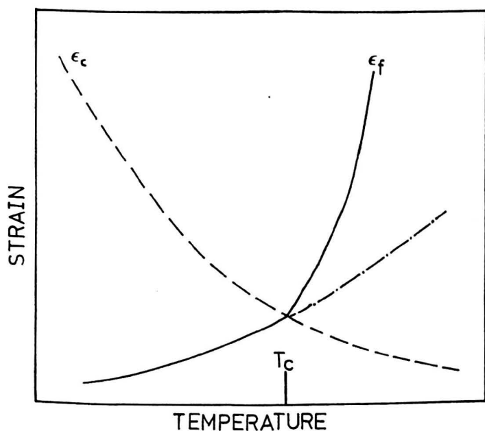
Fig. 11.1 Schematic illustration of variation of fracture strain ( \epsilon_f ) and strain for the nucleation of dynamic recrystallization, ( \epsilon_c ) with temperature.
