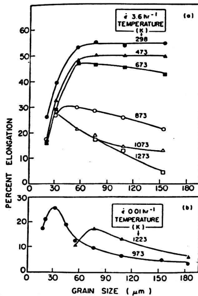
Fig. 2.11 Variation of ductility with temperature and grain size for a Cr-Mn-N Austenitic steel, showing decrease in ductility at fine grain sizes. (From Kutumba-RaO et al, 1975)
