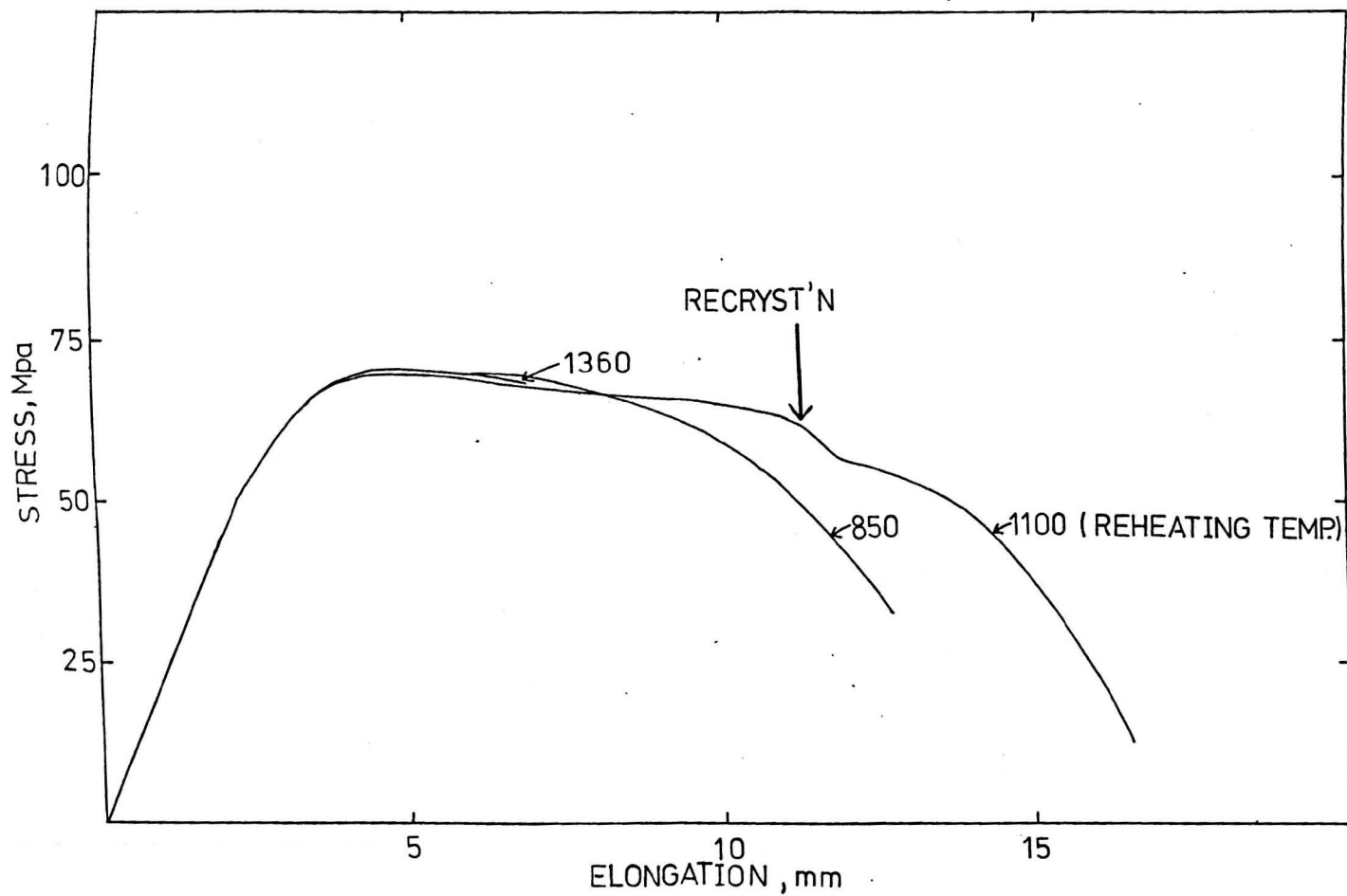
Fig. 6.6 Load elongation curves for the C-Mn-Nb-Al steel
