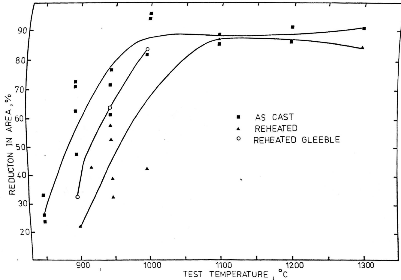
Fig. 9.2 Variation of Reduction in area with test temperature for samples in 'as cast', 'reheated' and 'reheated Gleeble' samples.
