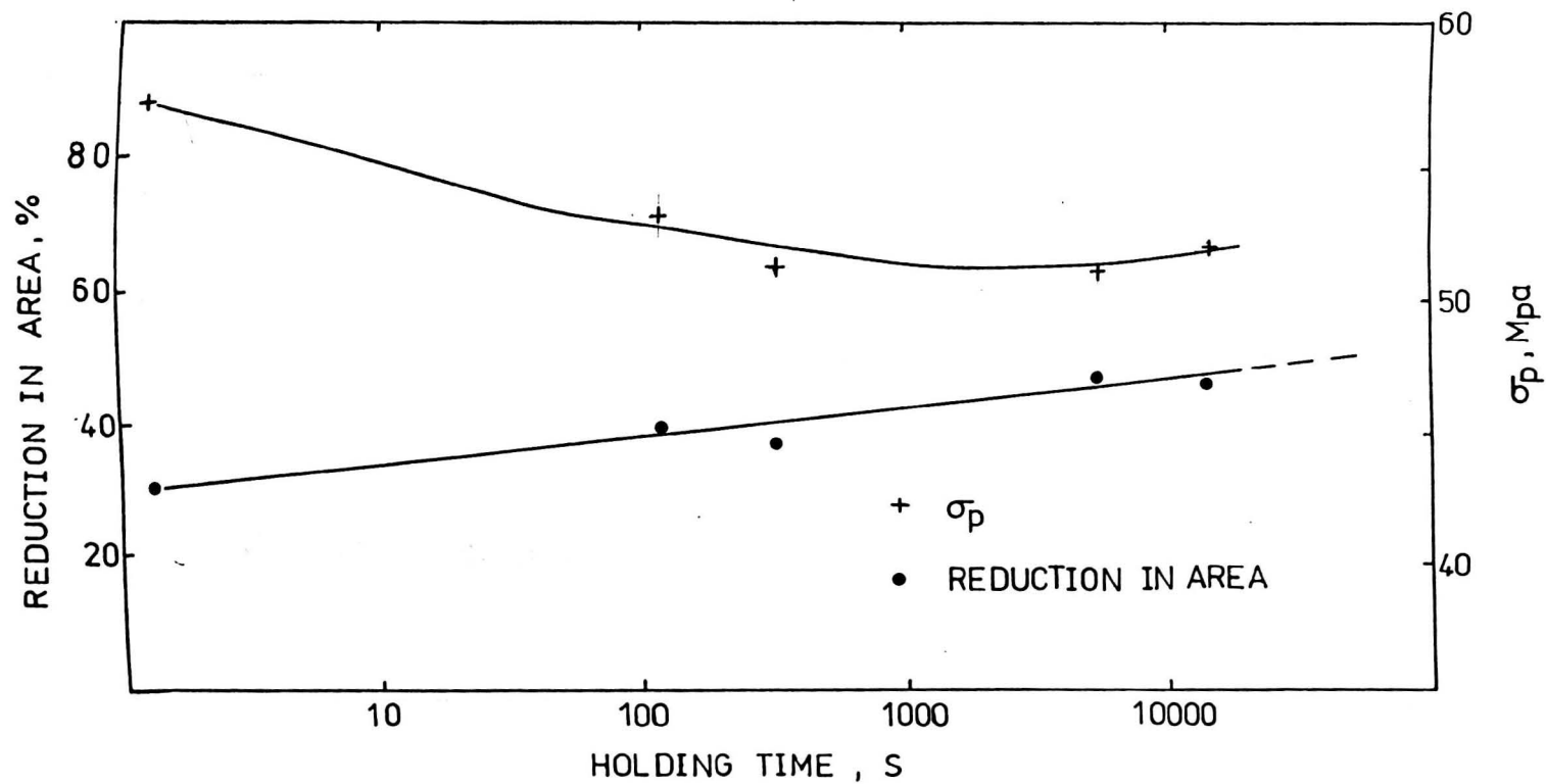
Fig. 7.1 Influence of holding time prior to testing on peak stress and hot ductility of the C-Mn-Nb-Al steel, tested at 50°C.
