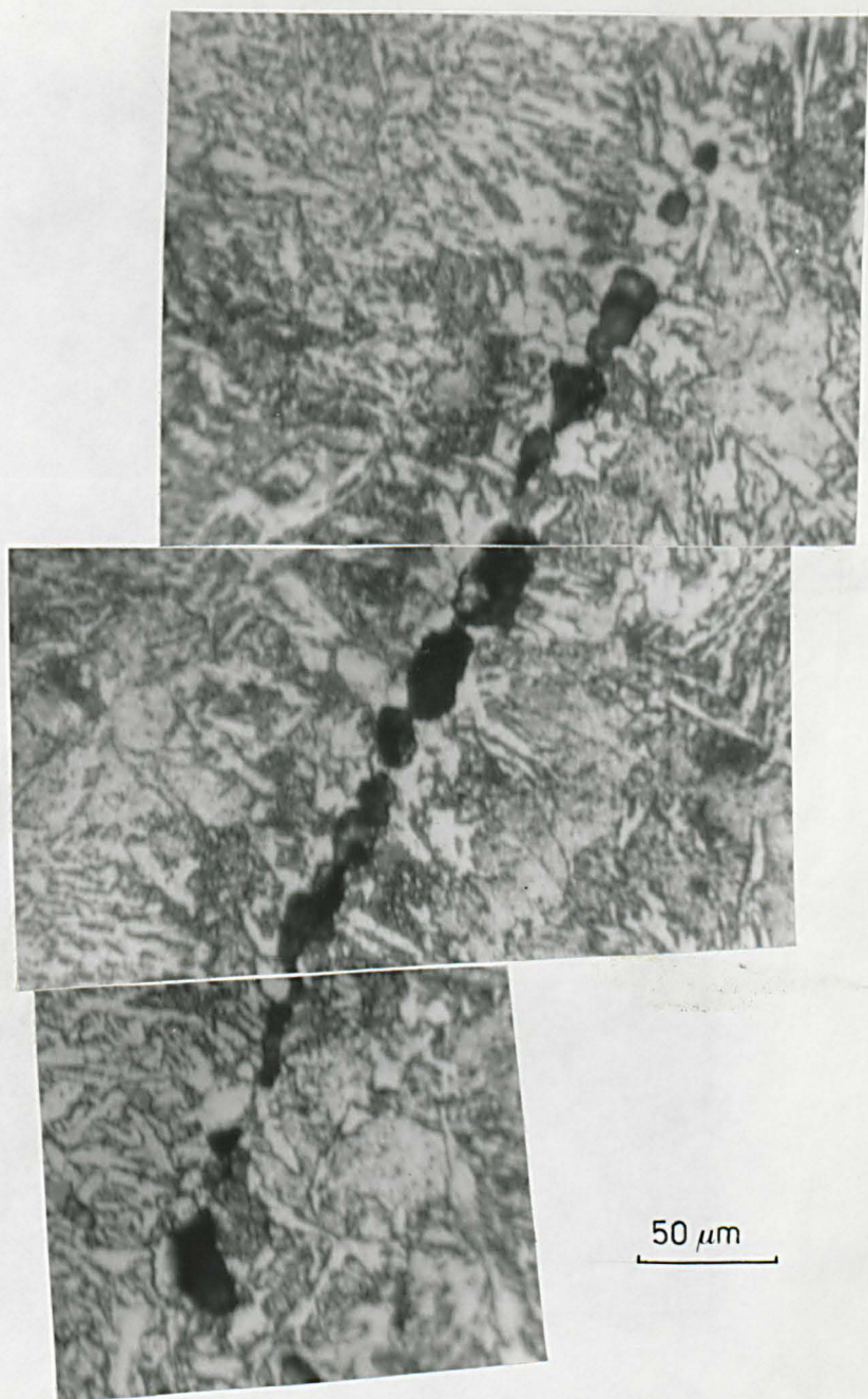
Fig. 4.14 Detail of crack formation in .19%C steel tested at 650°C
