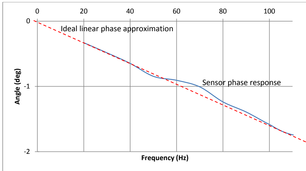
Figure 3.33 Sensor phase response magnified segment
