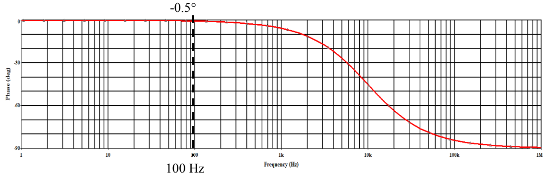
Figure 3.52 RC filter phase over frequency characteristic
