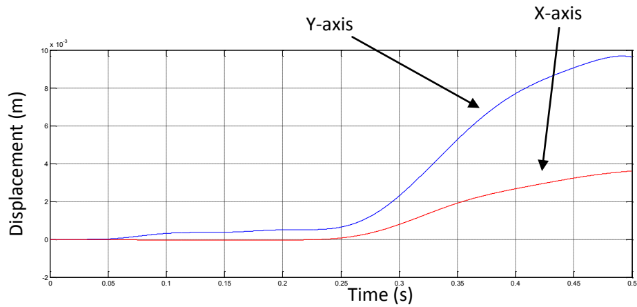
Figure 5.43 HPAGS x and y-axis displacement data in gyro mode.
