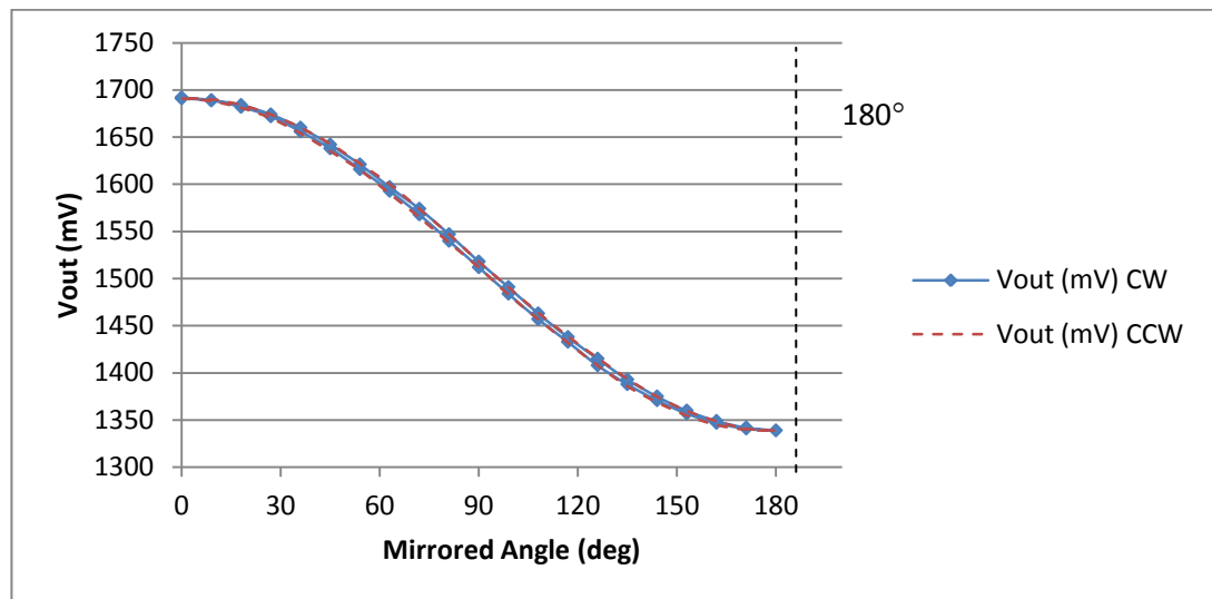
Figure 3.38 Folded y-axis output along the 180^\circ line
