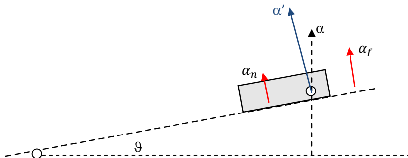
Figure 1.4 Non sensor-concentric rotation due to acceleration.
