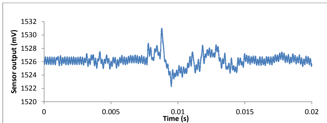
Figure 3.29 Mechanical vibration with 6.1KHz dithering injected via the test pin
