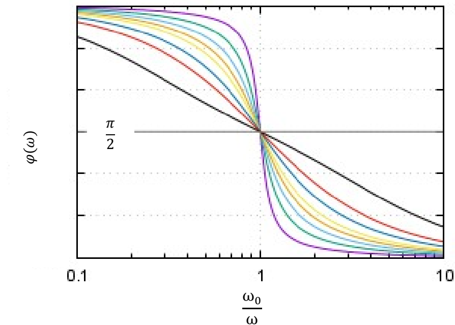
Figure 2.8 Phase response of systems (public domain)
