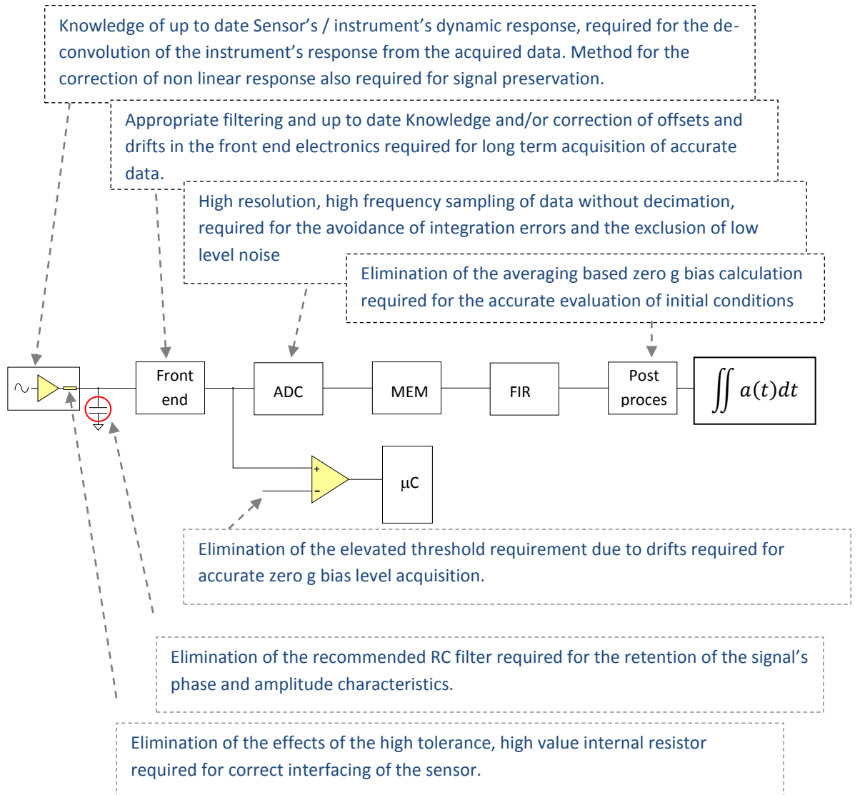
Figure 4 Specification diagram of HPAGS sensor base on error analysis
