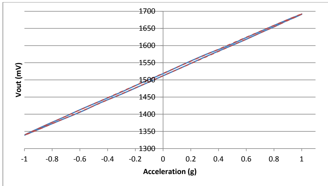
Figure 3.43 Mathematically derived y-axis output with added 2% cross-axial sensitivity
