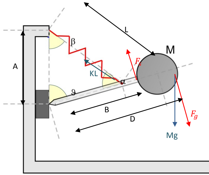
Figure 2.13 The “LACoste” seismometer arrangement
