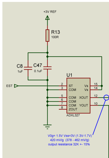
Figure 4.3 Detail of MEMS circuit
