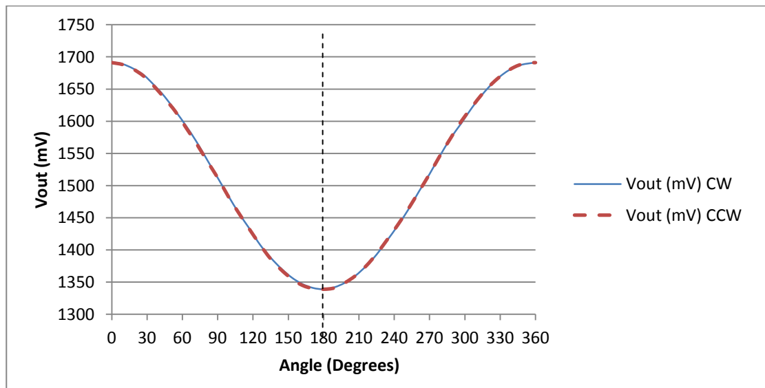
Figure 3.37 y-axis voltage output for 0 - 360° rotation and back to zero
