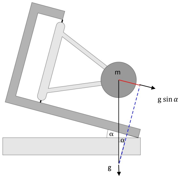
Figure 2.11 The “Garden gate” arrangement
