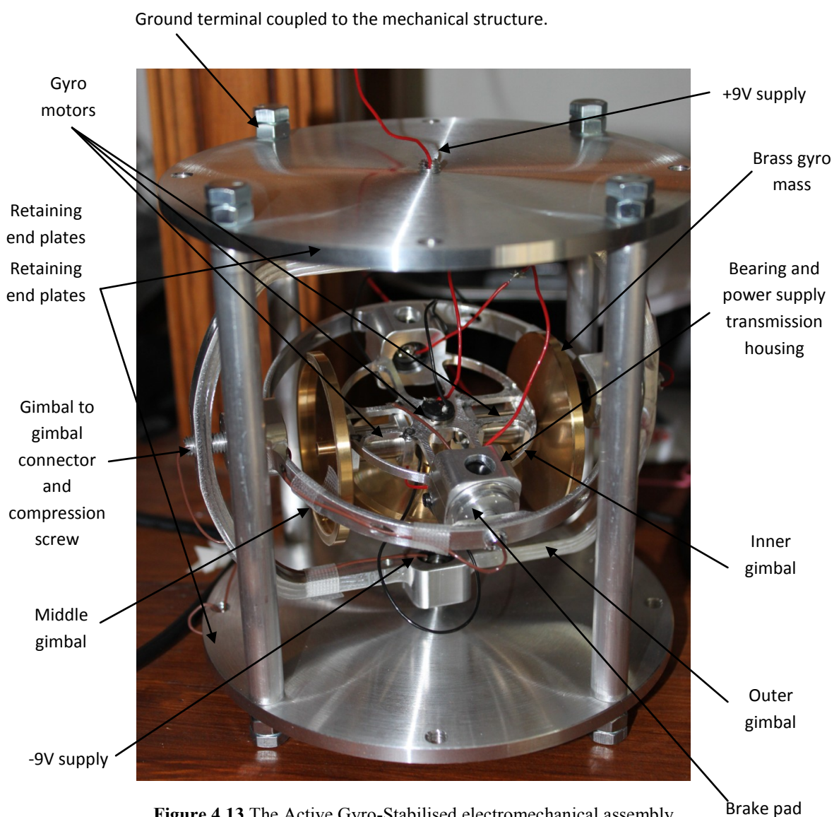
Figure 4.13 The Active Gyro-Stabilised electromechanical assembly
