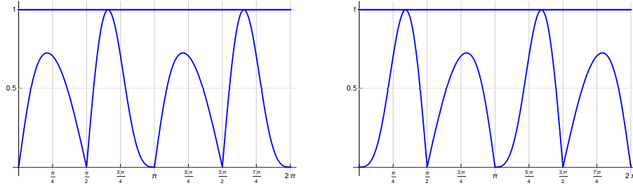
Figure 3: Standard deviations \sigma_{H_\theta} , \sigma_{E_\theta} (upper horizontal lines) and expectation values |\langle U_\theta/2 \rangle_{e_1}| (left panel), |\langle U_\theta/2 \rangle_{e_2}| (right panel), as functions of \theta .
