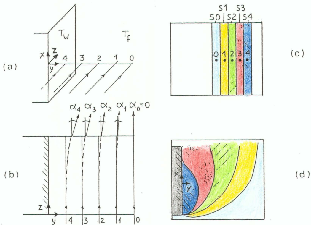
FIGURE 4.8 Colour schlieren method: (a) light beam entering the test section (a vertical heated wall), (b) angular deflections on the z - y plane, (c) positions of 0-1-2-3-4 rays at the focal plane where the colour filter is held, (d) colour schlieren image.
