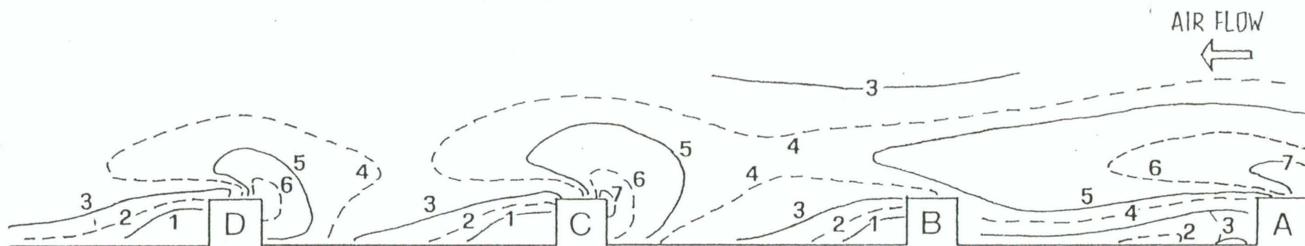
FIGURE 3.30 Contours of lines at equal Nu number, Re=10000 . 1, (Nu=) 52; 2, 61; 3, 72; 4, 85; 5, 93; 6, 112; 7, 131.
