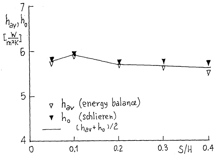
FIGURE 4.22 Overall heat transfer coefficients h_{av} (energy balance) and h_o (optical data) against S/H , smooth channel configuration, Ra=1.8 \cdot 10^7 .
