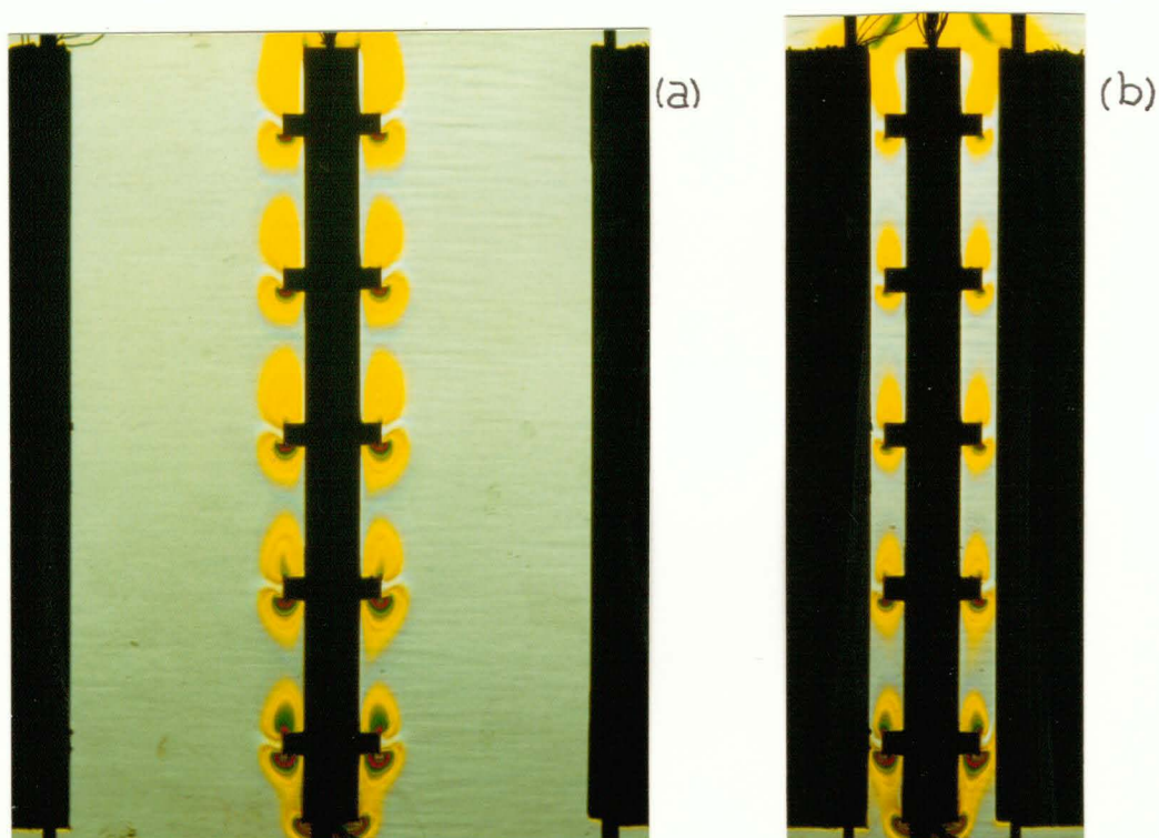
FIGURE 4.26 Colour schlieren images of the rough channel assembly, filter mounted horizontally, Ra=1.8 \cdot 10^7 : (a) S/H=0.3 , (b) S/H=0.05 .
