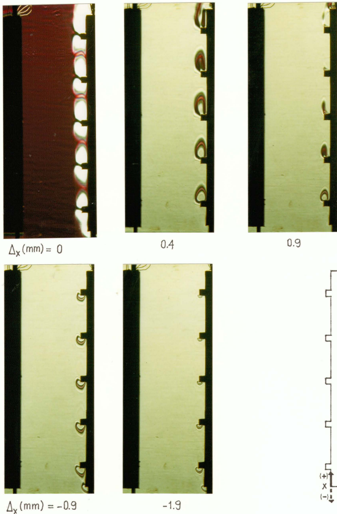
FIGURE 4.28 Schlieren images (focal filament method) of the rough channel configuration, filter mounted horizontally, Ra=1.8 \cdot 10^{-7} , S/H=0.3 . \Delta_x from 0 to 0.9 mm (top) and to -1.9 mm (bottom).
