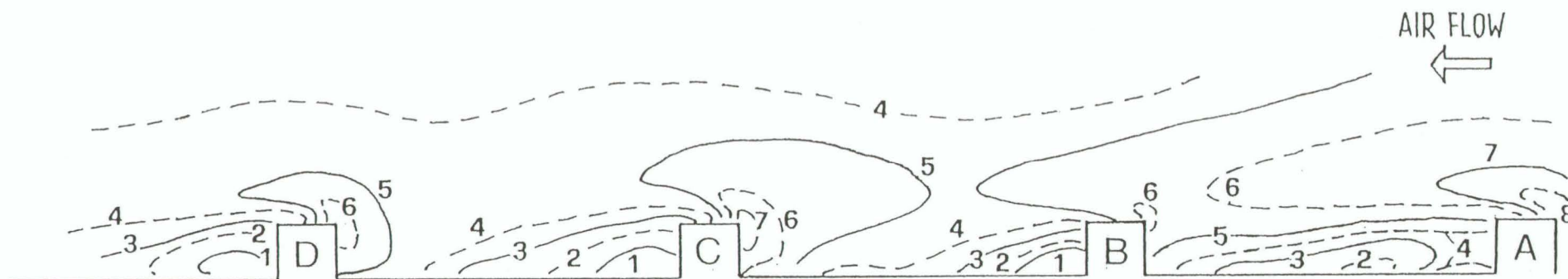
FIGURE 3.31 Contours of lines at equal Nu number, Re=6000 . 1, ( Nu= ) 40; 2, 44; 3, 49; 4, 56; 5, 62; 6, 74; 7, 91; 8, 100.
