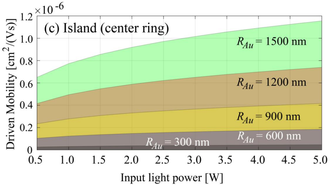
Figure 3: The plots of the mobility outputs, the gold and graphene layer parameters are w = 0.5 \text{ }\mu\text{m} , thickness = 0.5 \text{ }\mu\text{m} , the gold and graphene island thickness = 0.5 \text{ }\mu\text{m} .
