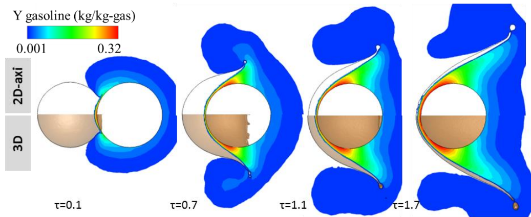
Figure 5.3: Effect of CFD simulation dimensions on collision outcome for a DTP=1, U_o=15\text{m/s} , T_p=1,000\text{K} impact, Case2 (top), Case2* (bottom). Contour of the produced gasoline mass fraction (kg-gasoline/kg-gas). The iso-surface of \alpha=0.5 is depicted for the 3D case (bottom).
