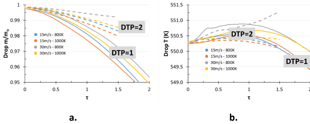
Figure 4.15: Droplet a) mass and b) temperature evolution for all cases, (solid lines-DTP1, dashed lines-DTP2).
