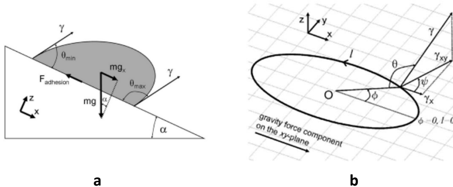
Figure 2.8: Adhesion force. a) Droplet sliding down an incline. At the moment it starts moving, f_{adh} = mg \sin \alpha . b) Projection of the contact area of the droplet on the incline. Reprinted with permission from [171] Copyright 2009 American Chemical Society.
