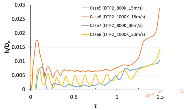
Figure 4.13: Temporal evolution of vapour layer thickness at impact point for cases 5-8.
