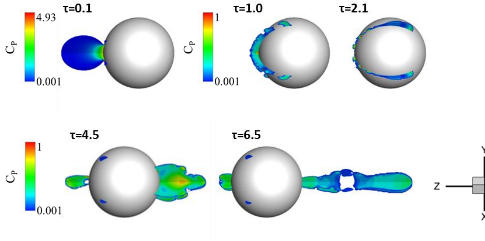
Figure 3.41: Temporal evolution of C_p for Case5 (DTP=0.62_We=40) at slices x=0 and symmetry plane y=0 .
