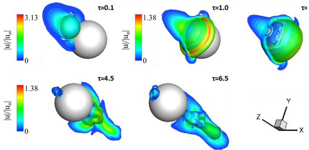
Figure 3.38: Temporal evolution of drop-particle collision for Case5 (DTP=0.62_We=40). Drop iso-surface ( \alpha=0.5 ) and symmetry plane y=0 coloured by the dimensionless velocity magnitude. Values below 0.15 are cut-off.
