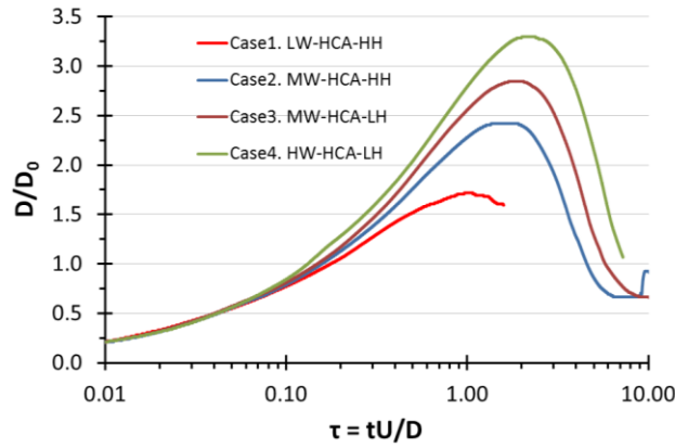
Figure 3.23: Non-dimensional spreading diameter from WFM simulation plotted against non-dimensional time for hydrophobic surfaces. \theta_{adv} = 105^\circ - 120^\circ . We=8 - 91 , x-axis, logarithmic scale.
