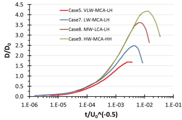
Figure 3.28: Non-dimensional spread factor from WFM simulation plotted against non-dimensional time for hydrophilic surfaces. \theta_{adv} = 10^\circ - 70^\circ . We = 0.2 - 117 , x-axis, logarithmic scale.
