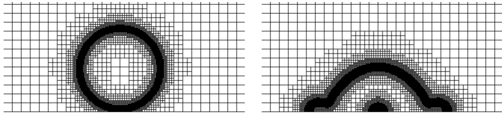
Figure 2.2: Dynamic local grid refinement applied at the case of a droplet impinging onto a solid flat surface.
