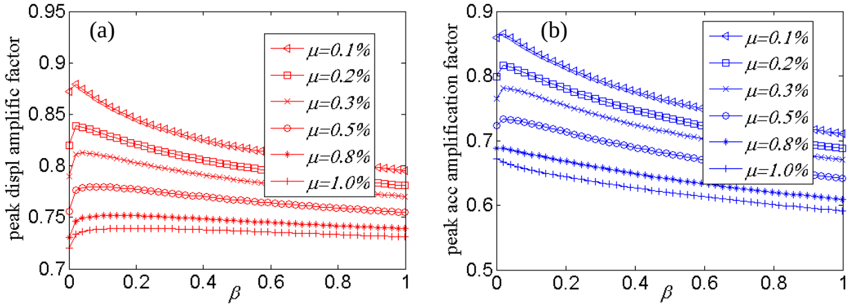
Figure 4- Peak top floor displacement (a) and acceleration (b) of TMDI equipped primary structure for different values of inertance ratio \beta=b/M and attached mass ratio \mu=m_{TMDI}/M and normalised by the corresponding peak values of the uncontrolled structure.
