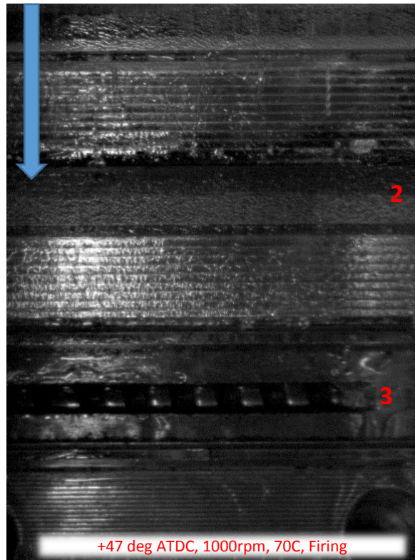
Figure 173 – 1000rpm, 70C, Firing
