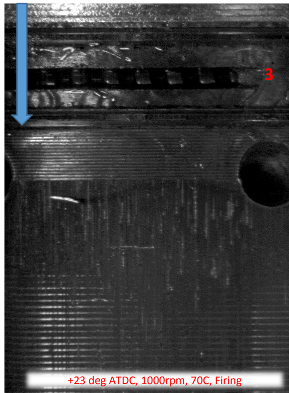
Figure 172 – 1000rpm, 70C, Firing
