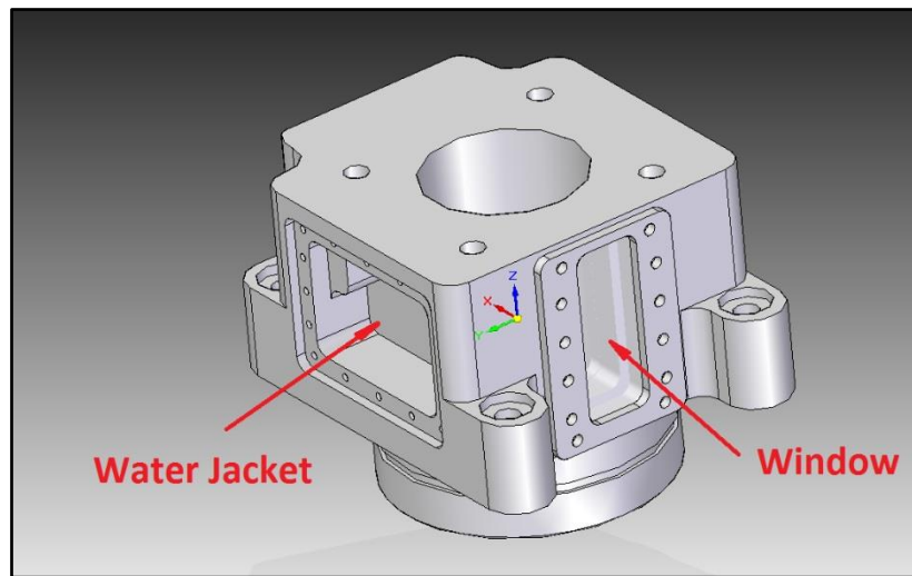
Figure 49 - Ricardo Hydra optical-engine 3D final design
