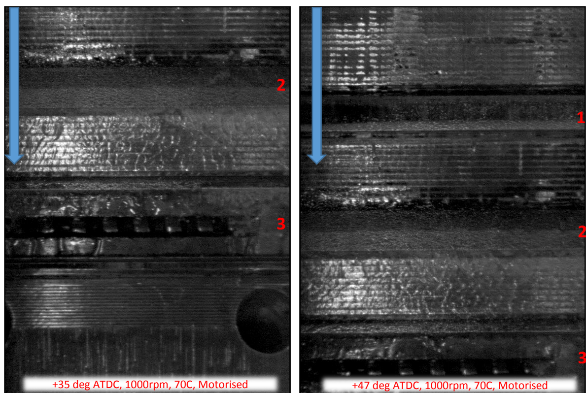
Figure 150 - ATDC, 1000rpm, 70C, Motorised
