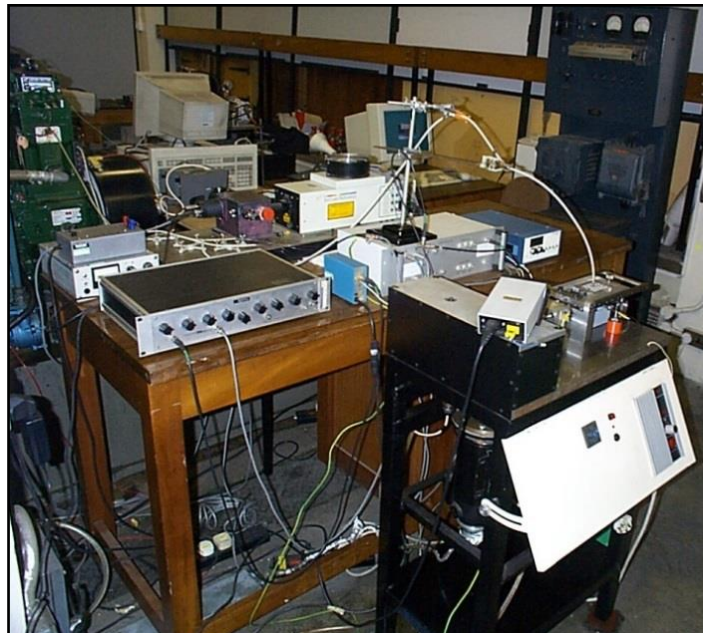
Figure 23 - Optical test-rig as used by Ostovar (Ostovar, 1996)
