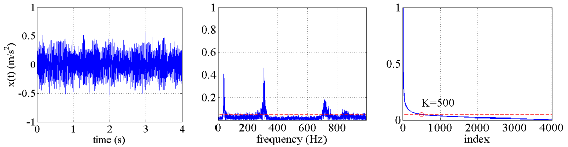
Figure 1: Typical noisy acceleration response signal with \text{SNR}=10\text{dB} ; (left panel): time history; (middle panel): normalized single-sided Fourier spectrum magnitude; (right panel): Normalized magnitude Fourier coefficients in descending order. The red broken line signifies an arbitrary threshold at normalized Fourier spectrum of 0.05.
