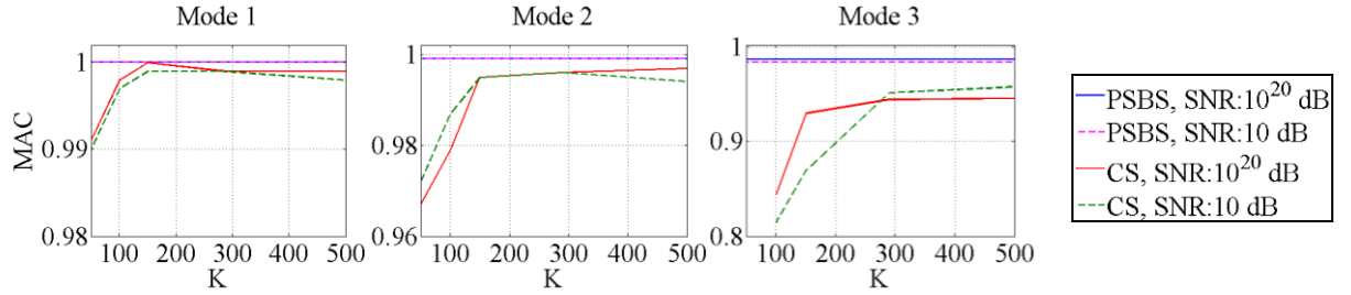
Figure 4: MAC versus reconstruction sparsity level K_T , obtained from the two considered approaches, PSBS-based and CS-based FDD, for CR=31\% and SNR=\{10^{20}, 10\} dB.
