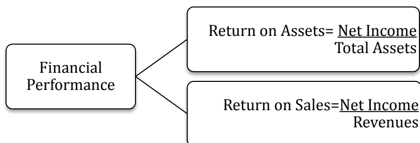
Figure 26. Metrics for financial performance used in this study
