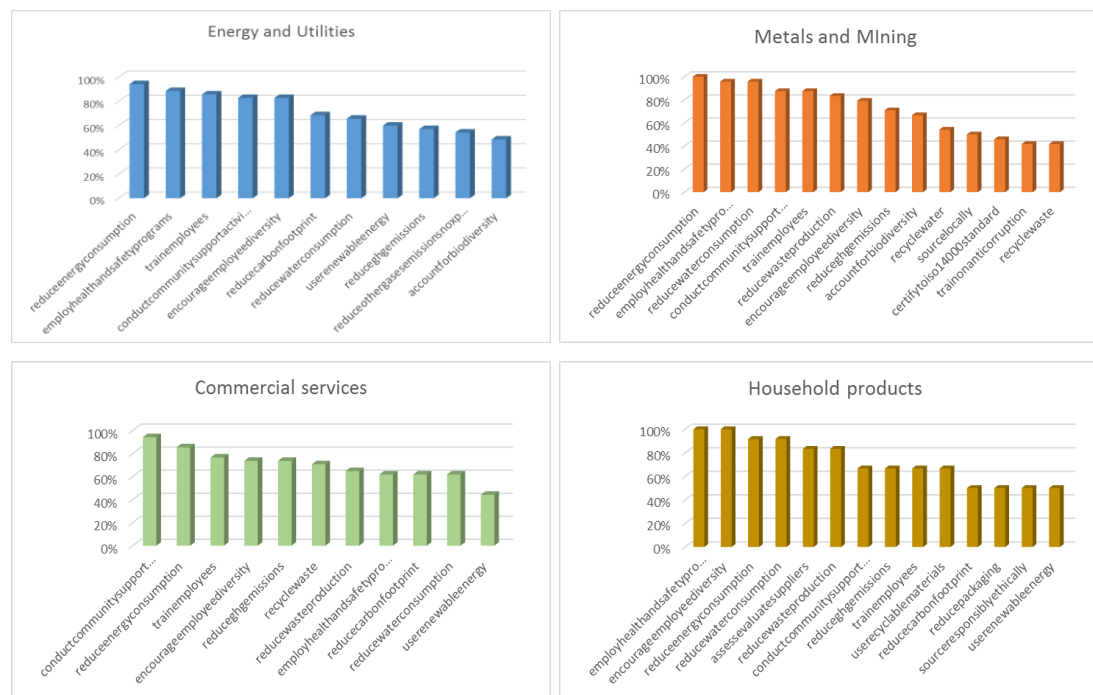
Figure 19. Frequency analysis of social and environmental indicators across the four selected industrial sectors
