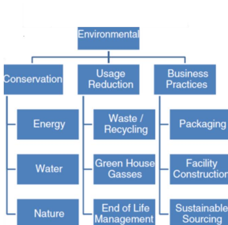
Figure 5. Categories and indicators underpinning environmental sustainability (Closs et al., 2011)
