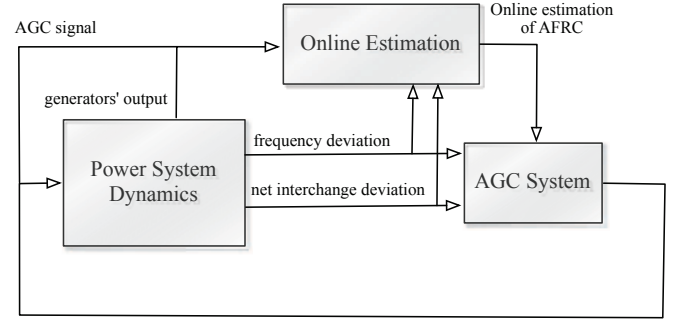
Fig. 1: Block diagram of the adaptive AGC system.
