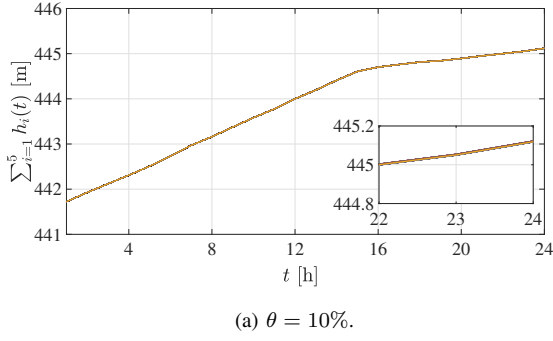
Fig. 6: Sum of head levels of the Tana River cascade for different uncertainty levels \theta for a one-day period.
