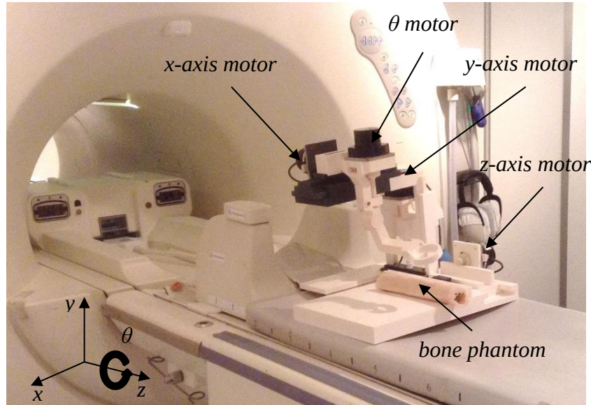
Figure 7.1: Setup of HIFU bone treatment positioning device on the MRI table with notations pointing the PUM motors that control motion in the xyz axes and theta ( \theta ) rotation..
