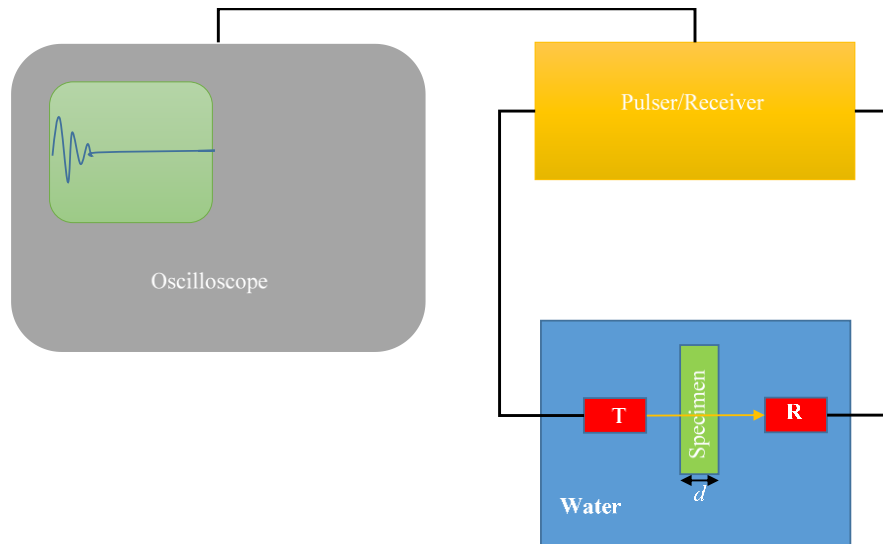
Figure 3.4: Experimental setup for the transmission through measurements of a specimen of thickness ( d ) in between the transmitter ( T ) and receiver ( R ) all immersed in a tank filled with degassed water.
