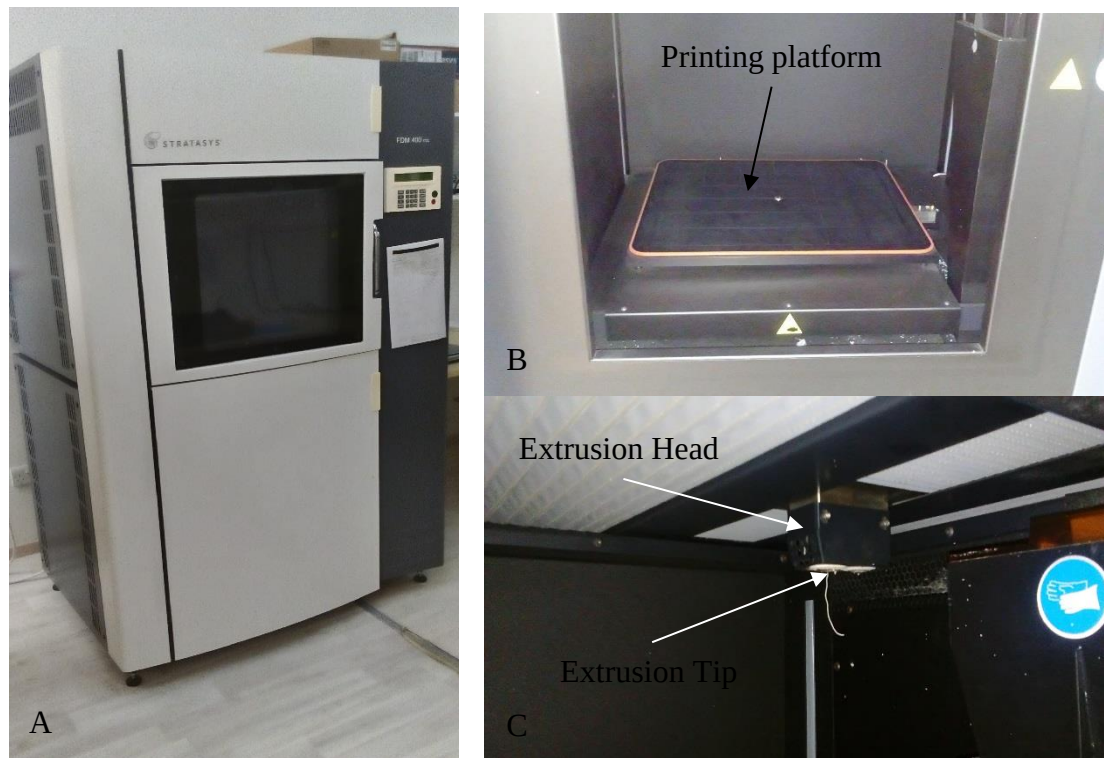
Figure 4.5: A) Stratasys Fortus FDM 400mc, B) 3D Printer's oven with platform, C) Extrusion head.
