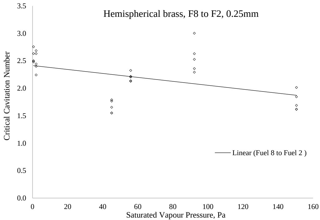
Figure A 8 - 2 Ca variation due to Saturated Vapour Pressure, 0.25 mm nozzle Hemispherical, F8 to F2f2
