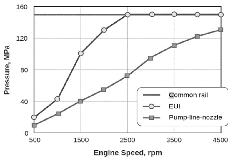
Figure 9 Pressure variations for corresponding changes in Engine Speed – Common Rail, Electronic Controlled Unit Injector (EUI), Pump-Line Nozzle [140]
