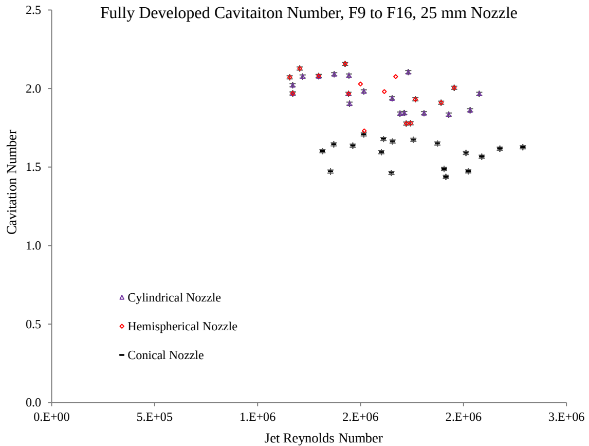
Figure 64 Fully Developed Cavitation Number as a function of Jet's Reynolds Number 0.25mm
