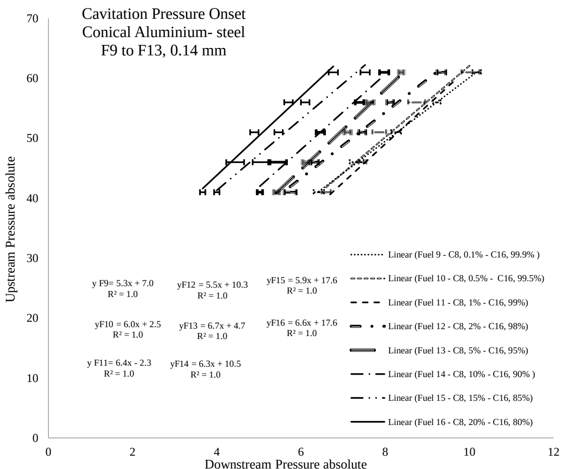
Figure 39 Cavitation Pressure Onset Conical 0.14mm: n-Hexadecane- n-Octane
