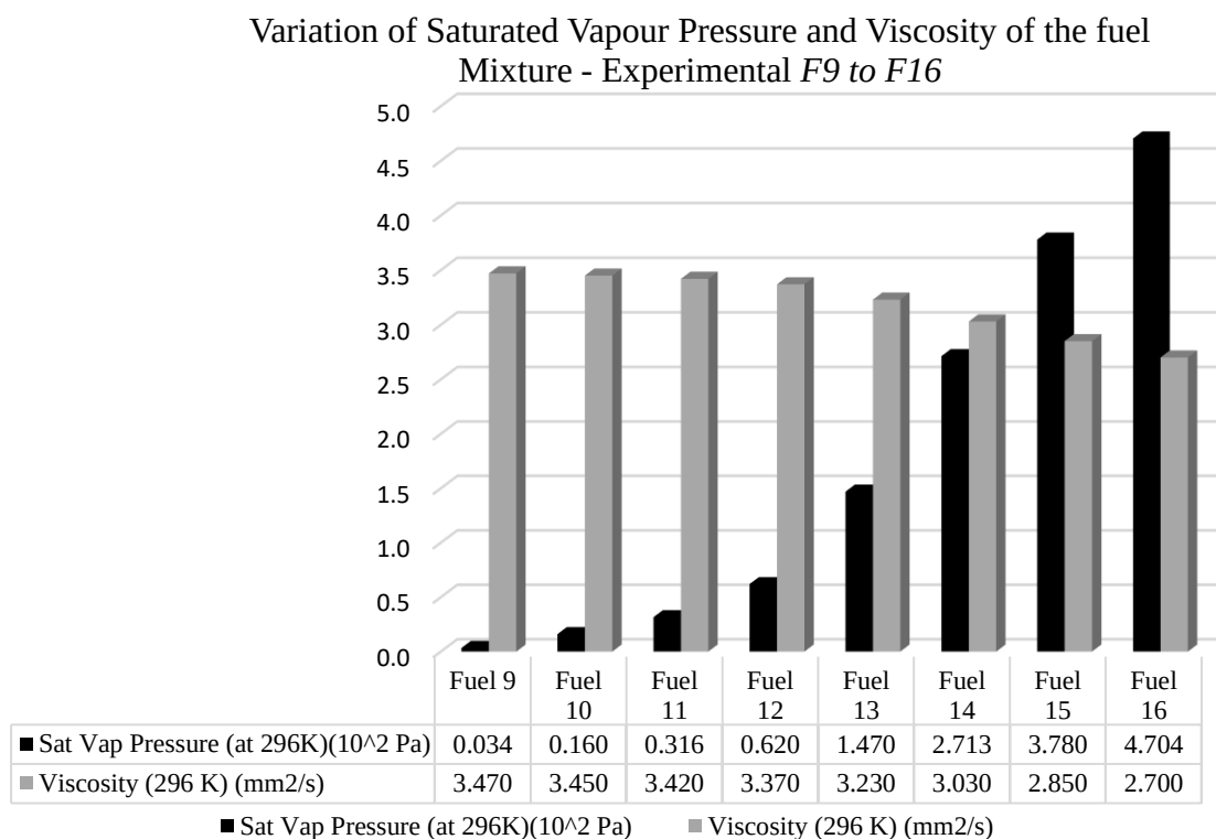
Figure 54 Comparison of the changes of Saturated Vapour Pressure to the Changes of Viscosity of the fuel mixture – Experimental F9 to F16
