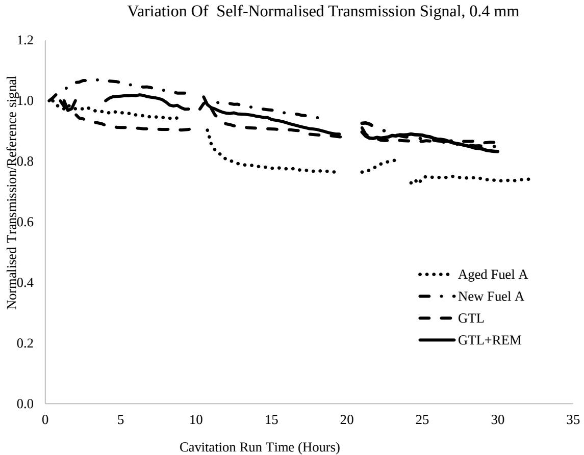
Figure 85 Self-Normalised Transmission Signal of all tested fuels
