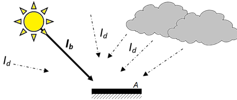
Figure 2.6 beam and diffuse solar radiations
