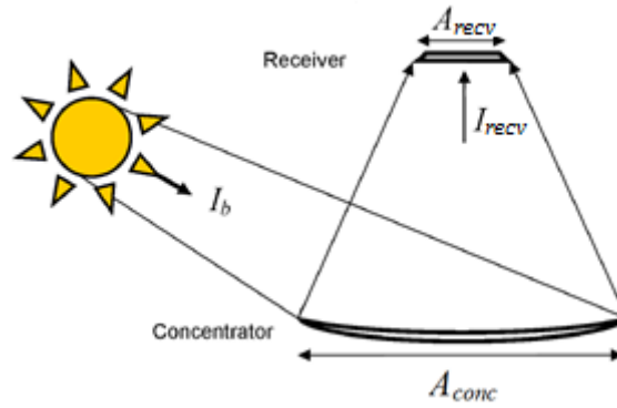
Figure 2.11 Concentration ratio
