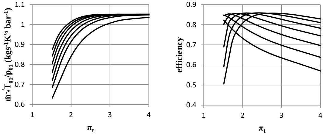
Figure 3.12 turbine performance maps, non-dimensional mass flow rate (left) and efficiency (right) against the pressure ratio
