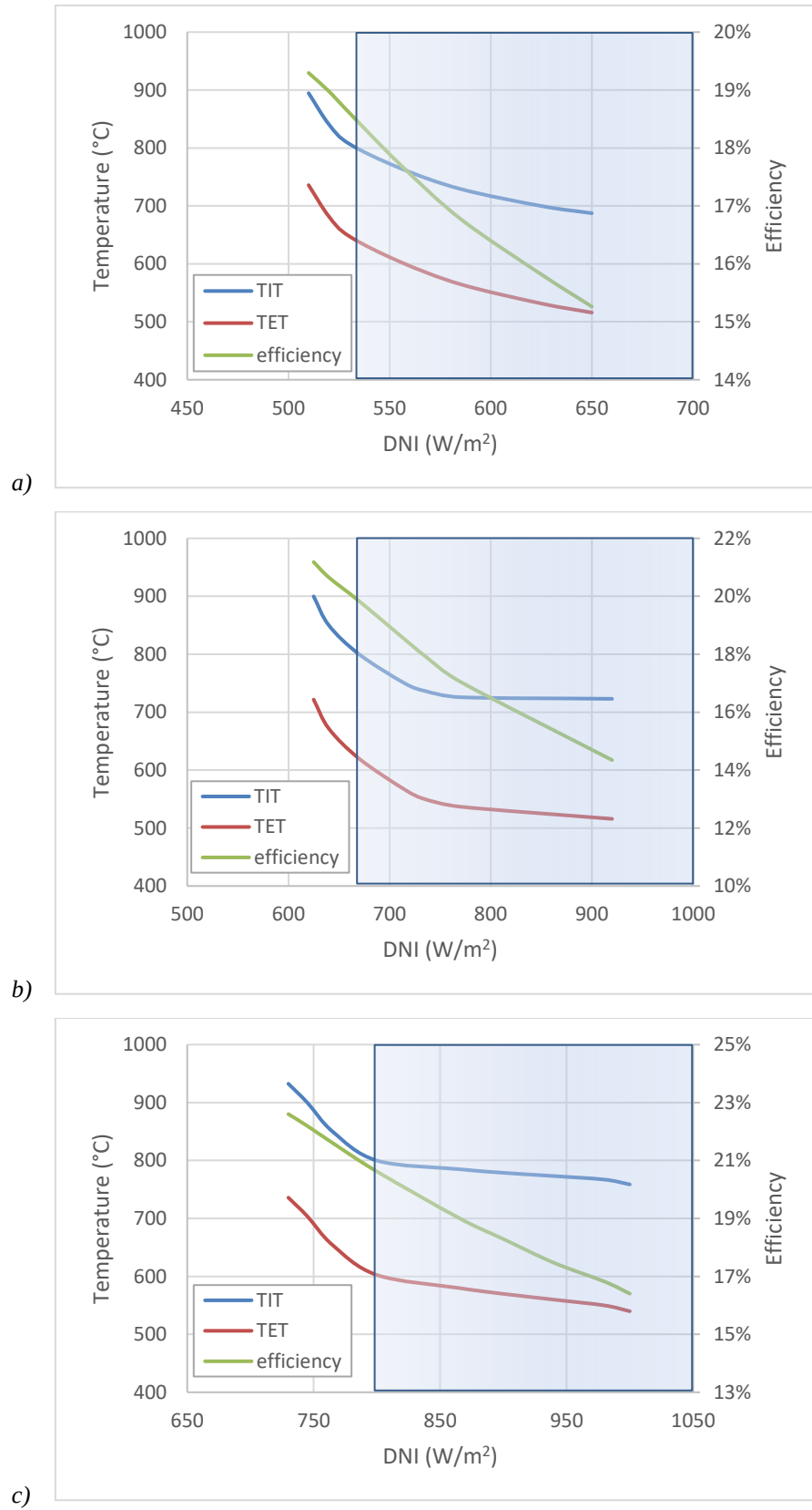
Figure 4.14 performance of the dish-MGT system when operated on fixed output power (a) P_{We}=3kWe , (b) P_{We}=4kWe and (c) P_{We}=5kWe . The shaded area shows the safe operation region.
