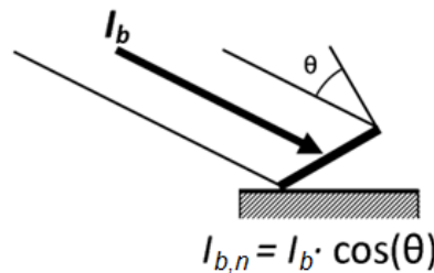
Figure 2.7 cosine effect in direct radiation
