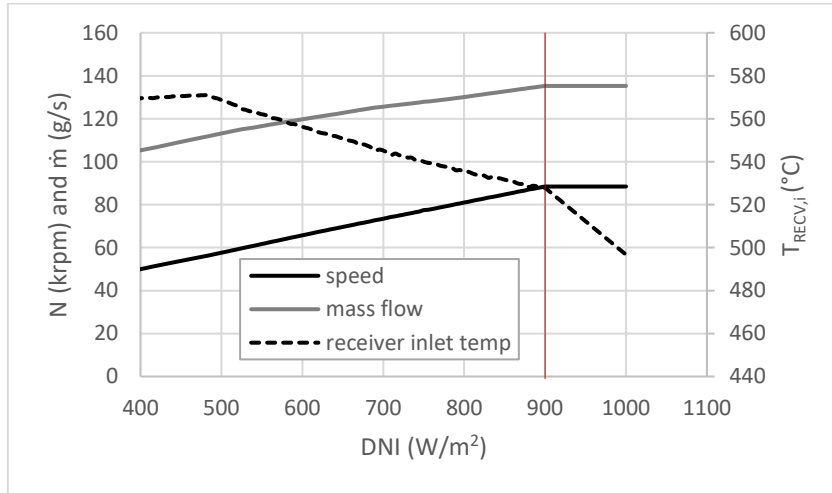
Figure 4.27 variation of speed, mass flow rate and inlet temperature of the receiver recuperation control applied for DNIs above 900W/m 2
