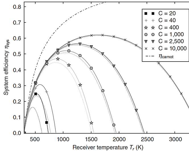
Figure 2.12 Ideal system efficiency as a function of receiver temperature. The dotted lines include the effect of convective heat losses (Lovegrove & Wes, 2012)
