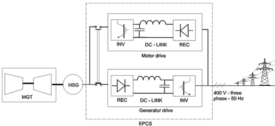
Figure 4.22 schematic of EPCS. Generation mode is activated (Ghavami, et al., 2017)
