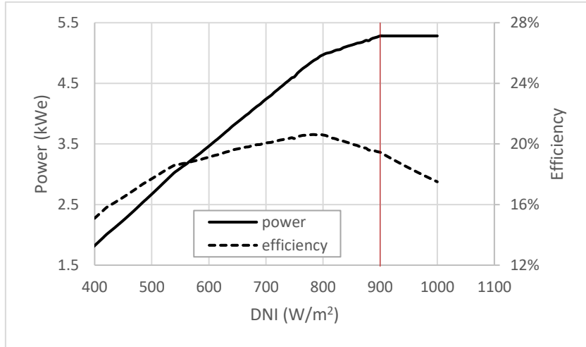
Figure 4.26 performance of the dish-MGT system with the recuperation control strategy applied for DNIs above 900W/m 2
