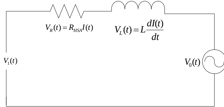
Figure B.2 single phase equivalent circuit of the HSA
