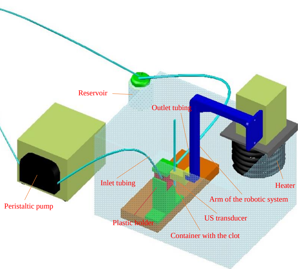
Figure 7.1: The experimental set up for in vitro sonothrombolysis, using a planar rectangular transducer.
