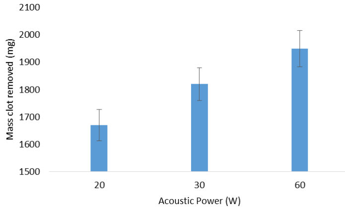
Figure 6.4: The effect of AP on clot lysis. Experimental parameters: f = 1.18 MHz, DF = 10\% , pulse duration = 1 ms, PRP = 10 ms and PRF = 100 Hz. treatment time = 30 min, flow rate = 50 mL/min, TNK-tPA concentration = 7.0 \mu\text{g/mL} , water bath temperature = 37^\circ\text{C} and no MBs.
