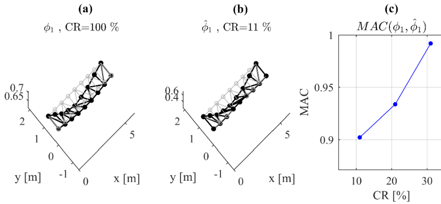
Figure 5.24: Estimation of the 1 st bending mode shape of the space truss; (a) conventional FDD at CR=100\% ; (b) PSBS-based FDD at CR=11\% ; and (c) MAC values versus CR
