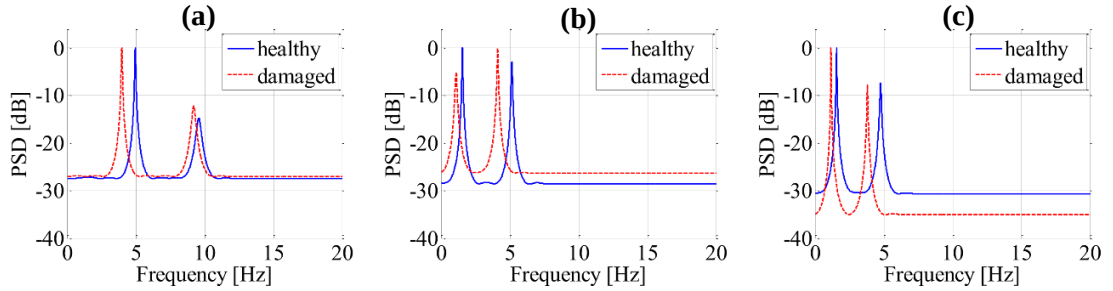
Figure 7.9: MUSIC pseudo-spectra with co-prime sampling of noisy acceleration response signals with SNR=10\text{dB} at the (a) first, (b) second, and (c) third floor for the healthy and the damaged state 2 structure in Figure 7.4
