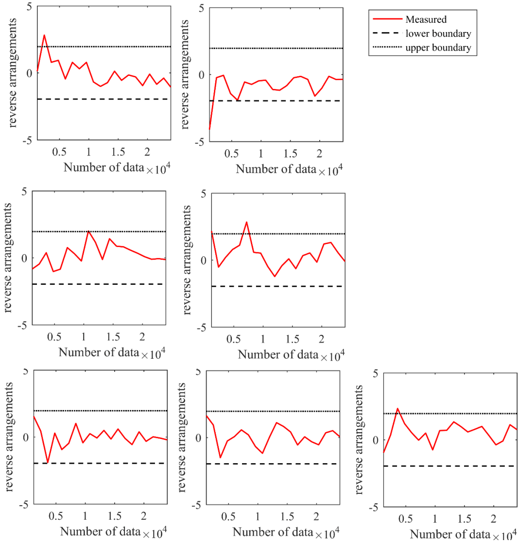
Figure 5.17: Reverse Arrangement method applied on acceleration response signal acquired from sensor at 80m height; signal is divided in 7 segments of 2min duration
