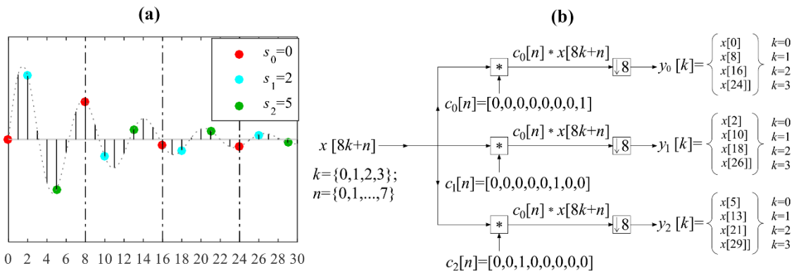
Figure 4.2: Multi-coset sampling pattern with \bar{M}=3 , \bar{N}=8 , K=4 , and sampling sequence \mathbf{s}=[0, 2, 5]^T applied on a signal of 32 samples
