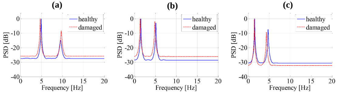
Figure 7.8: MUSIC pseudo-spectra with co-prime sampling of noisy acceleration response signals with SNR=10\text{dB} at the (a) first, (b) second, and (c) third floor for the healthy and the damaged state 1 structure in Figure 7.4
