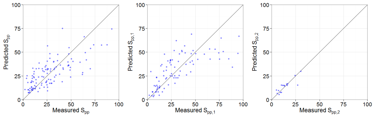
Figure 10: Values of post-peak descending branch slopes (dimensionless) measured experimentally (horizontal axes) against the ones predicted (vertical axes) using Eq. 7, 9 and 11 (from left to right).
