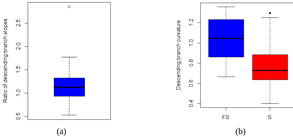
Figure 8: Ratio of descending branch slopes in two “directions” of the response of the database specimens (a). Curvature of the descending branch (c) of the response of flexure-shear critical (FS) and shear critical (S) specimens of the database (b).
