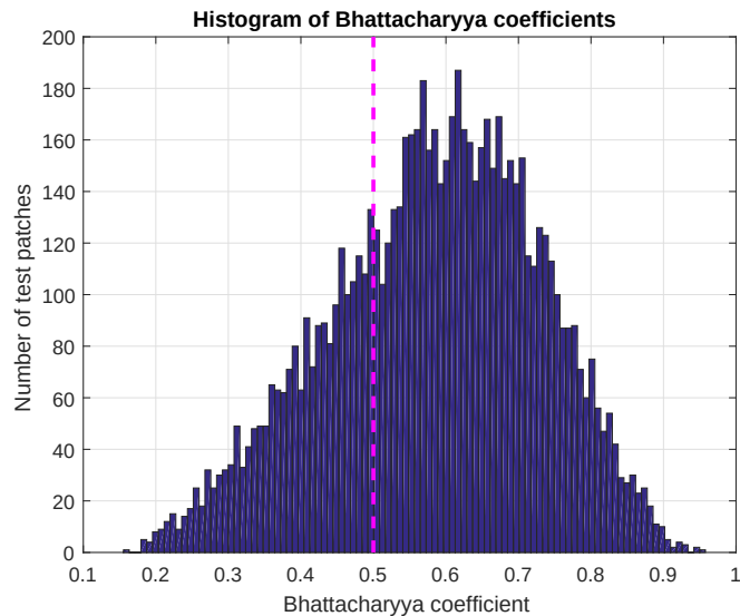
Fig. 4.9 Histogram of Bhattacharyya coefficients.
