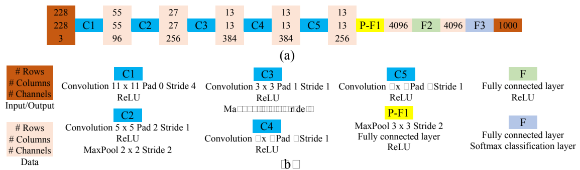
Fig. B.8 CNN (AlexNet) for large-scale image categorization (a) network architecture (b) legend.
