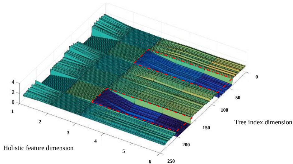
Fig. 4: A surface plot of the matrix \mathbf{A} (see Fig 3, used to weigh the expert trees based on the holistic hand feature). A higher value indicates more weight. Consider a hypothetical holistic hand feature vector, [0, 0, 0, 1, 1, 1] , which, when post-multiplied with \mathbf{A} will give less weighting to trees 40 to 80 and 160 to 200 based on their lower values (bluer colors), highlighted with red boxes.
