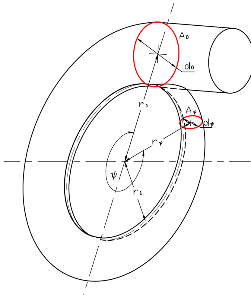
Figure 4.8: Turbine Volute
