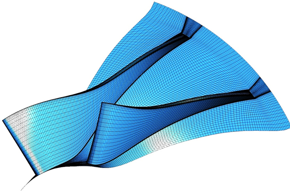
Figure 3.13: Impeller grid
