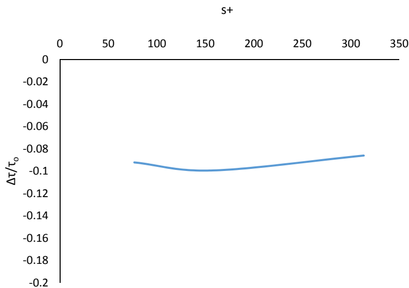
Figure 5.16: Drag reduction for different riblets spacing
