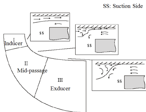
Figure 2.13: Schematic of flow in the tip clearance [43]
