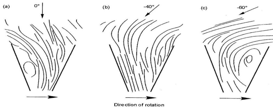
Figure 2.19: Flow baths for different incidence angle (a) zero incidence angle (b) -40^\circ incidence angle (c) -60^\circ incidence angle [32]
