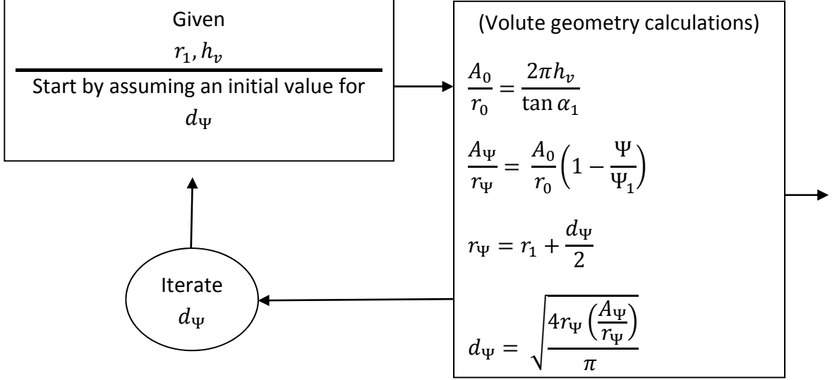
Figure 4.9: Volute design flow chart
