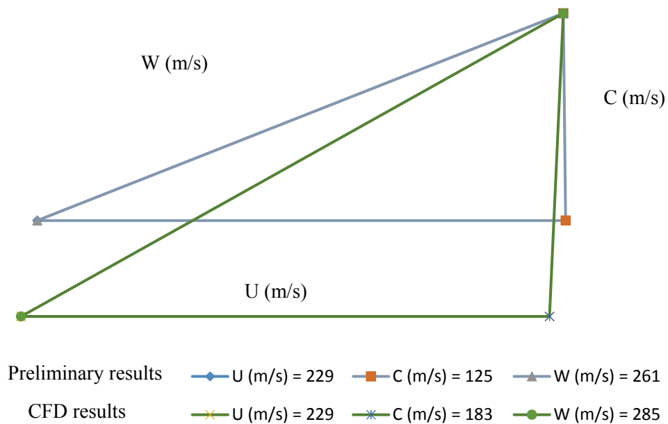
Figure 4.19: Velocity triangles at rotor outlet resulted from preliminary design and CFD results defined at RMS radius
