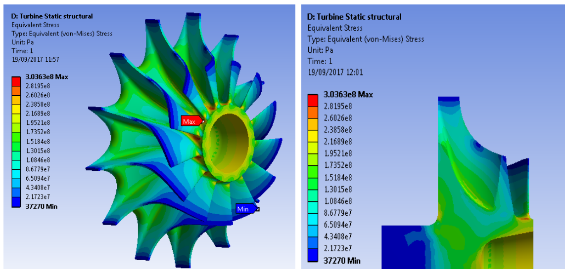
Figure 4.23: Equivalent stress in turbine operating at 130000 rpm and 698°C
