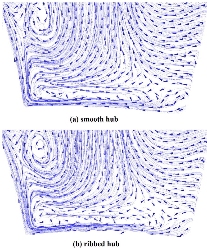
Figure 5.9: Effect of riblets on cross stream motion of the low energy fluids near the hub surface
