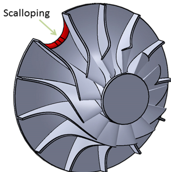
Figure 2.16: Rotor scalloping
