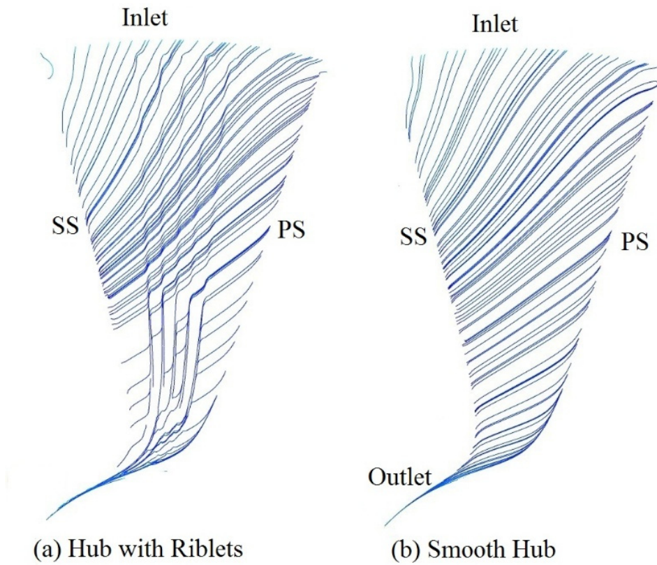
Figure 5.10: Limiting streamlines at the rotor hub
