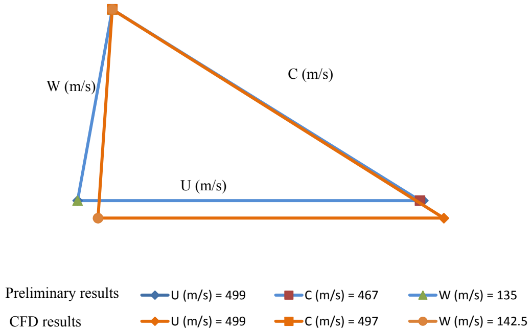
Figure 4.18: Velocity triangles at rotor inlet resulted from preliminary design and CFD results
