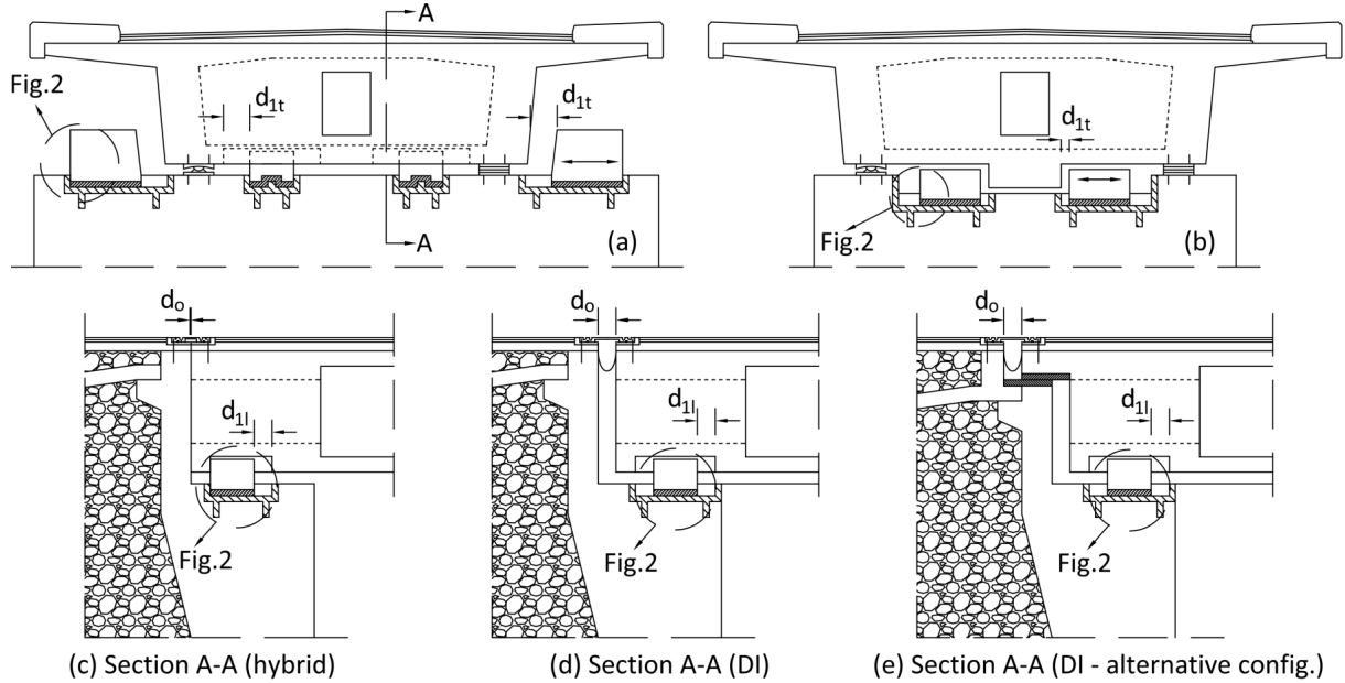
Figure 1: Possible configurations of bridges with adaptive boundary conditions: moveable shear keys in the transverse direction (top); in the longitudinal direction (bottom)
