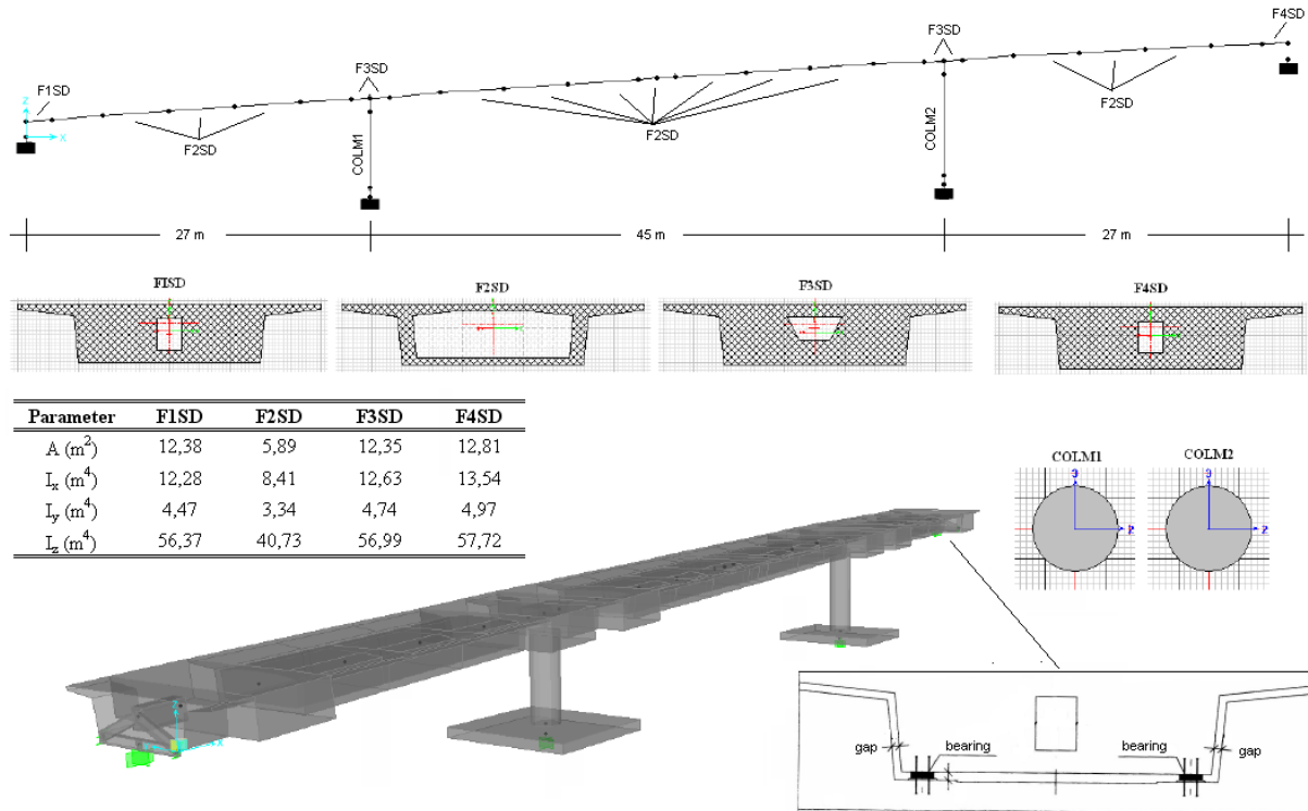
Figure 4: Layout of the bridge configuration and finite element modelling.
