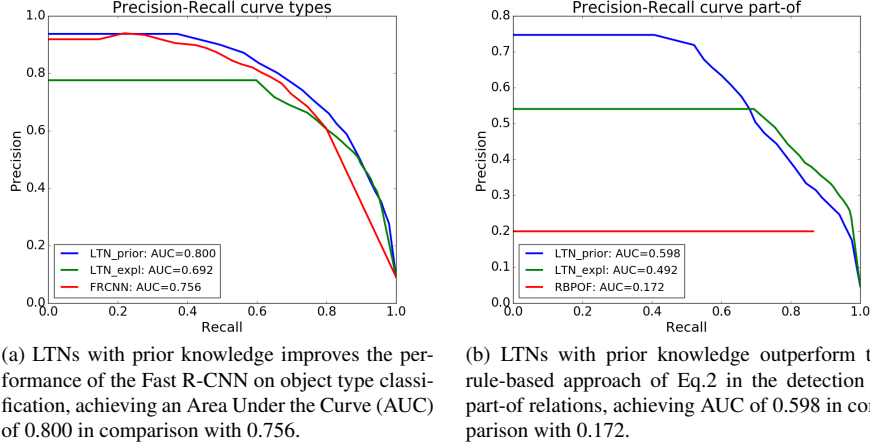
Figure 1: Precision-recall curves for indoor objects type classification and the partOf relation between objects.
