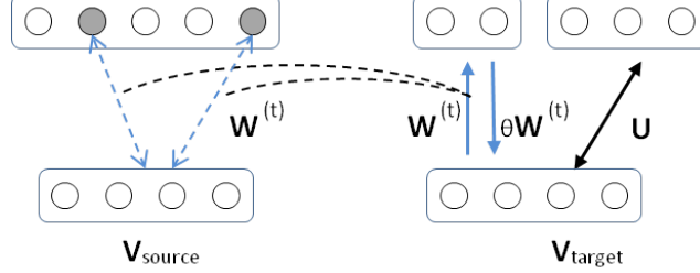
Figure 1: General adaptive feature transfer mechanism for unsupervised learning
