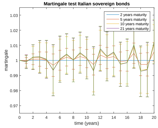
Figure 8: Martingale tests performed on sovereign German and Italian coupon bonds with 100 Monte Carlo simulations and parameter reported in Tables 1, 2 and 3. The error bars are the 97.5% confidence intervals.
